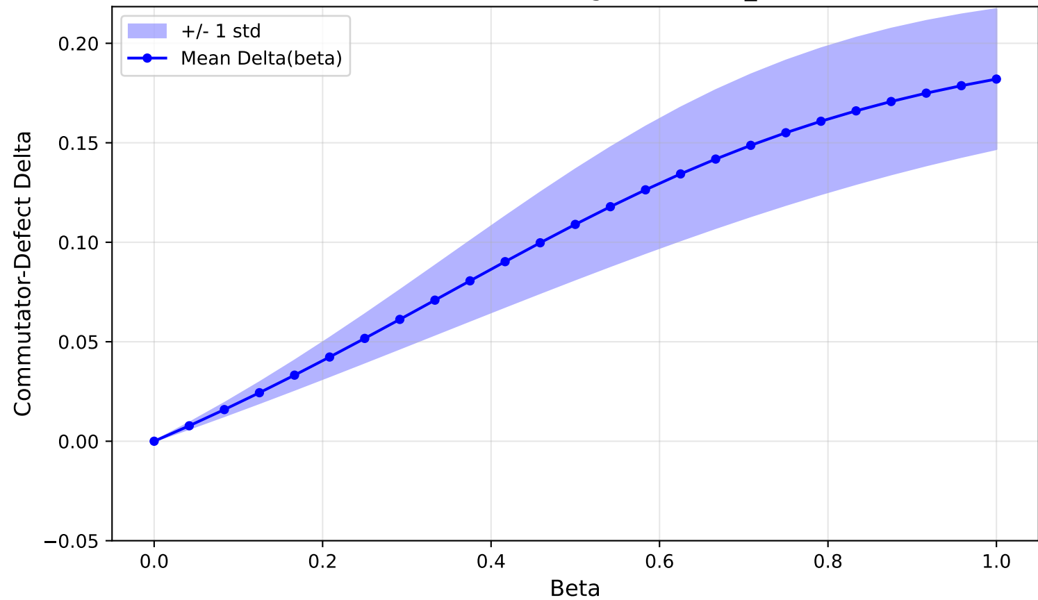
Commutator-Defect Surrogate (n=6, N_seeds=7)
