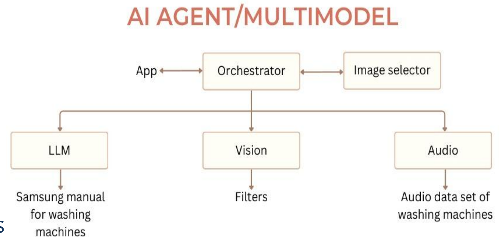
Fig. 1: Overall Architecture of entire application
