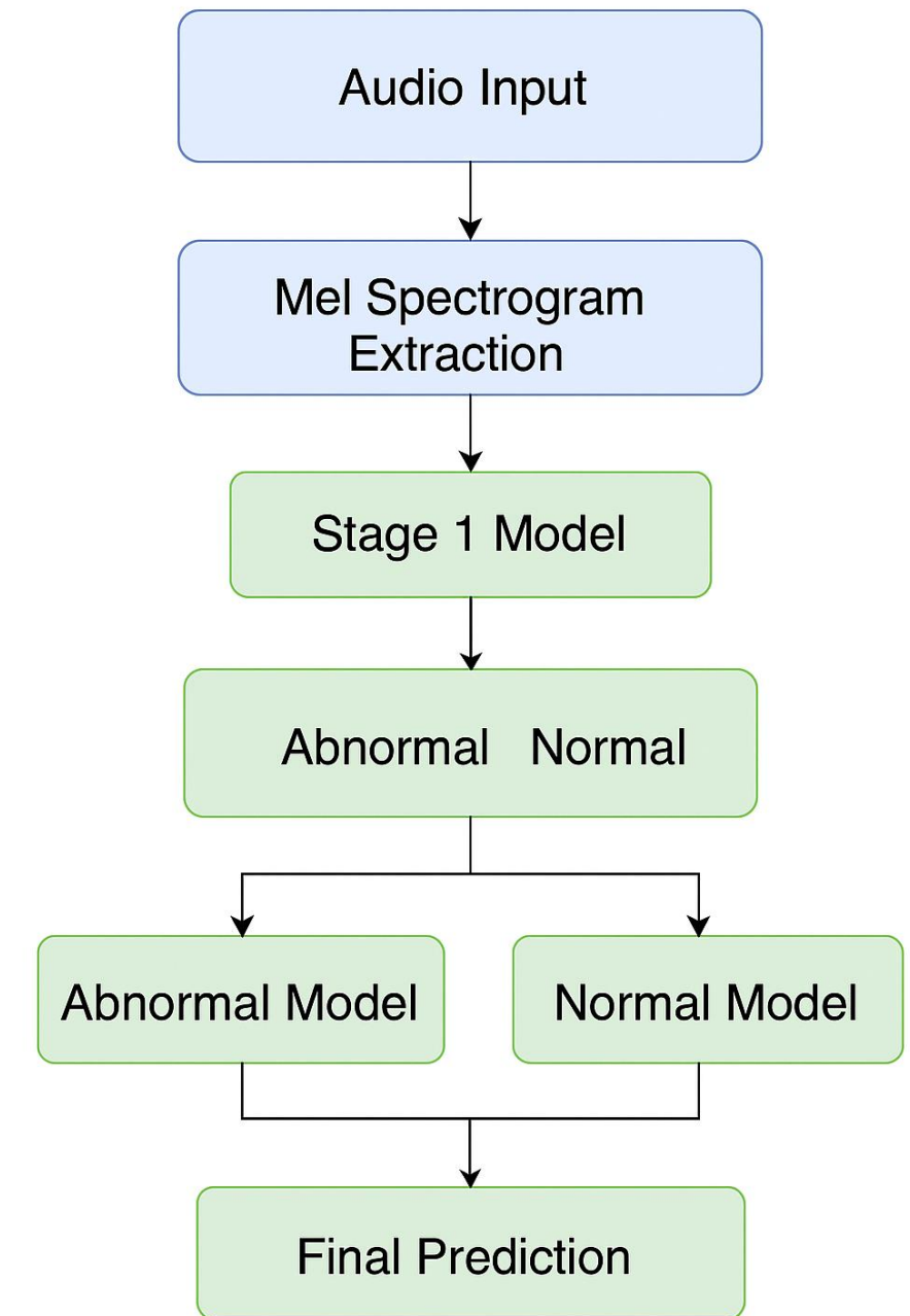
Fig. 5: Architecture of audio model
