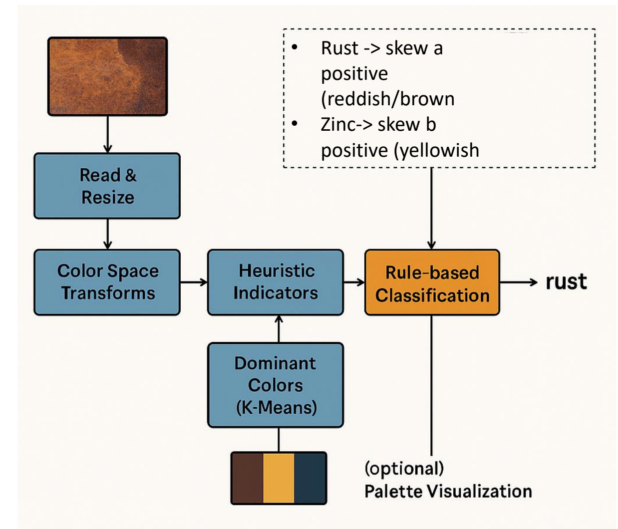
Fig. 3: Architecture of vision model
