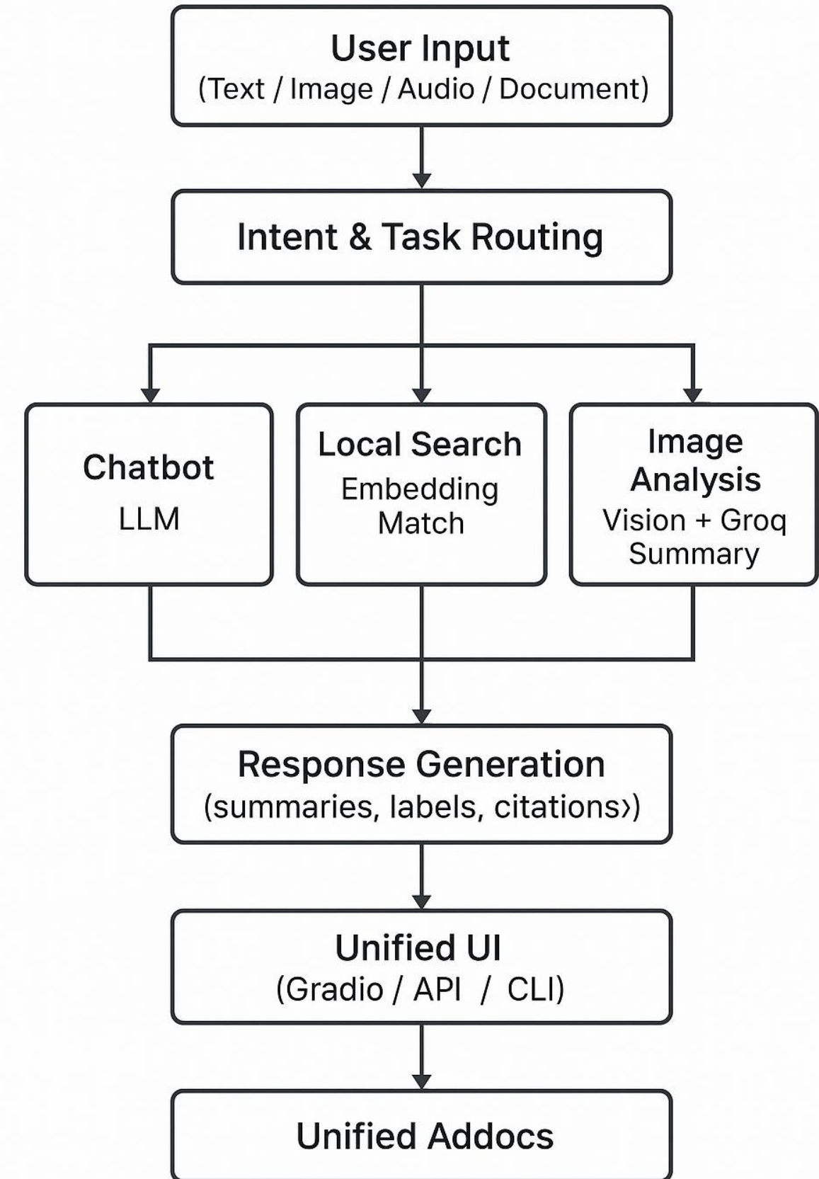
Fig. 2: Architecture of Orchestrator
