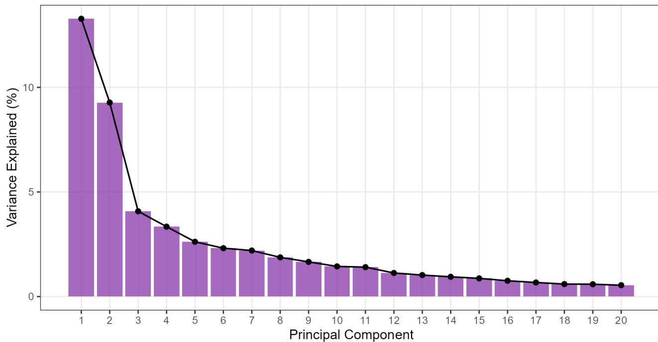
Scree Plot — Variance Explained by Each PC
