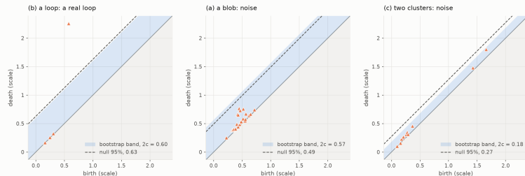
H_1 of the three Part 1 clouds: only a point above both lines is a feature
