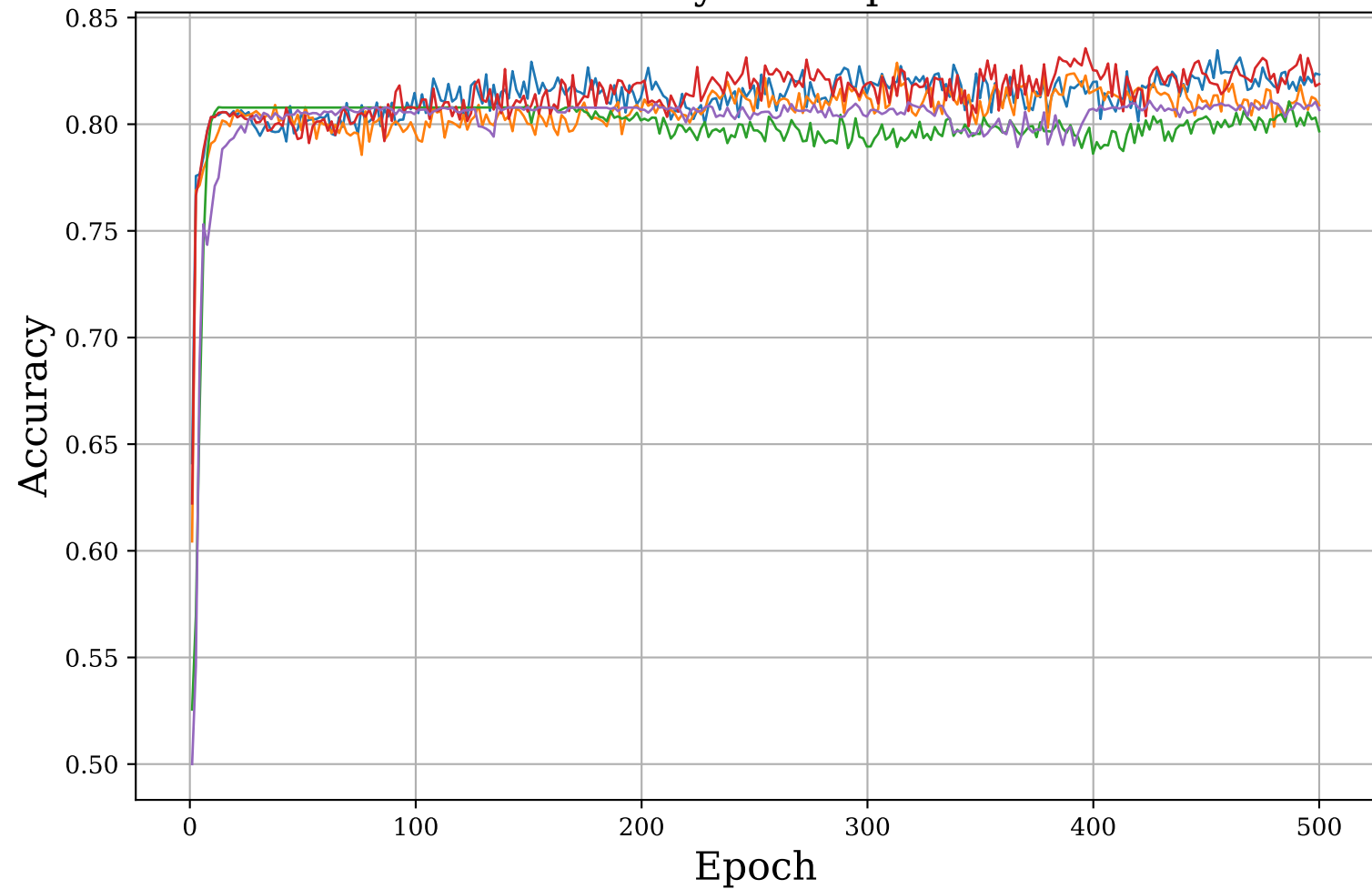
Accuracy over Epochs
