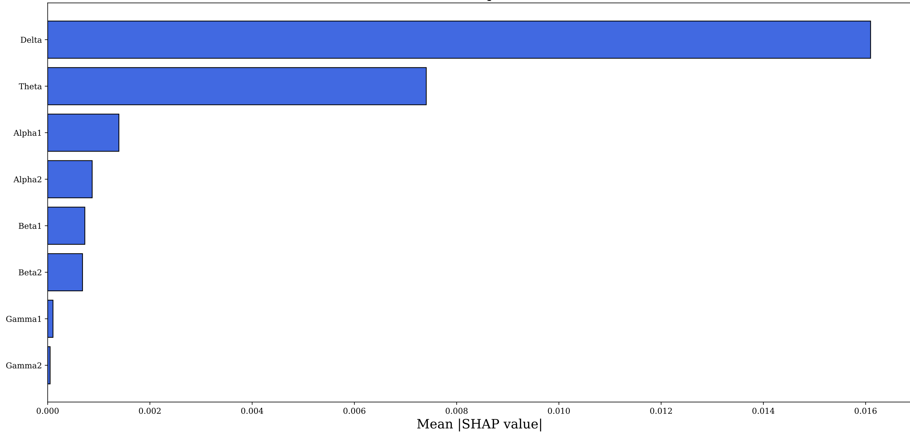
Feature Importance
