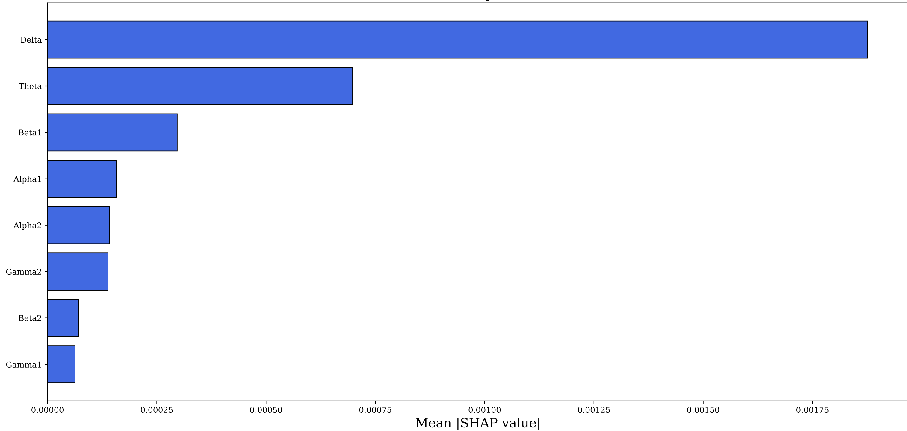
Feature Importance
