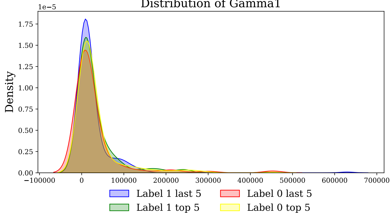
Distribution of Gamma1
