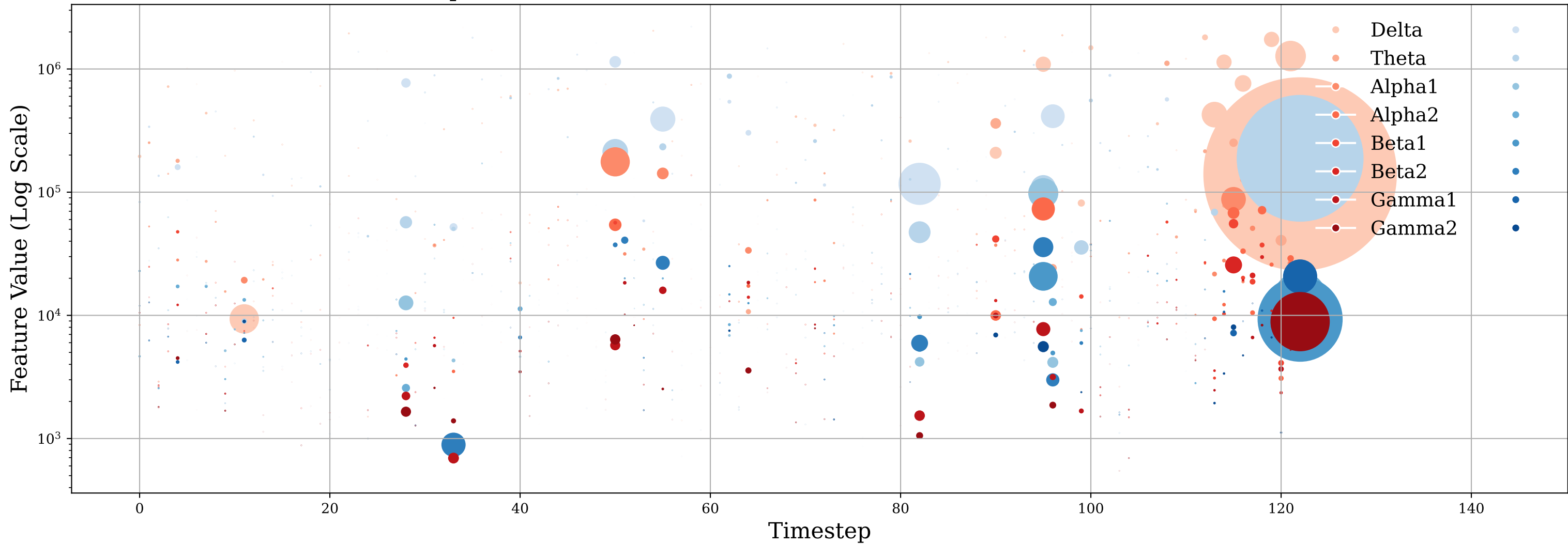
Sample 15. True value 'Confused'. Predicted 1 with 99.95% confidence
