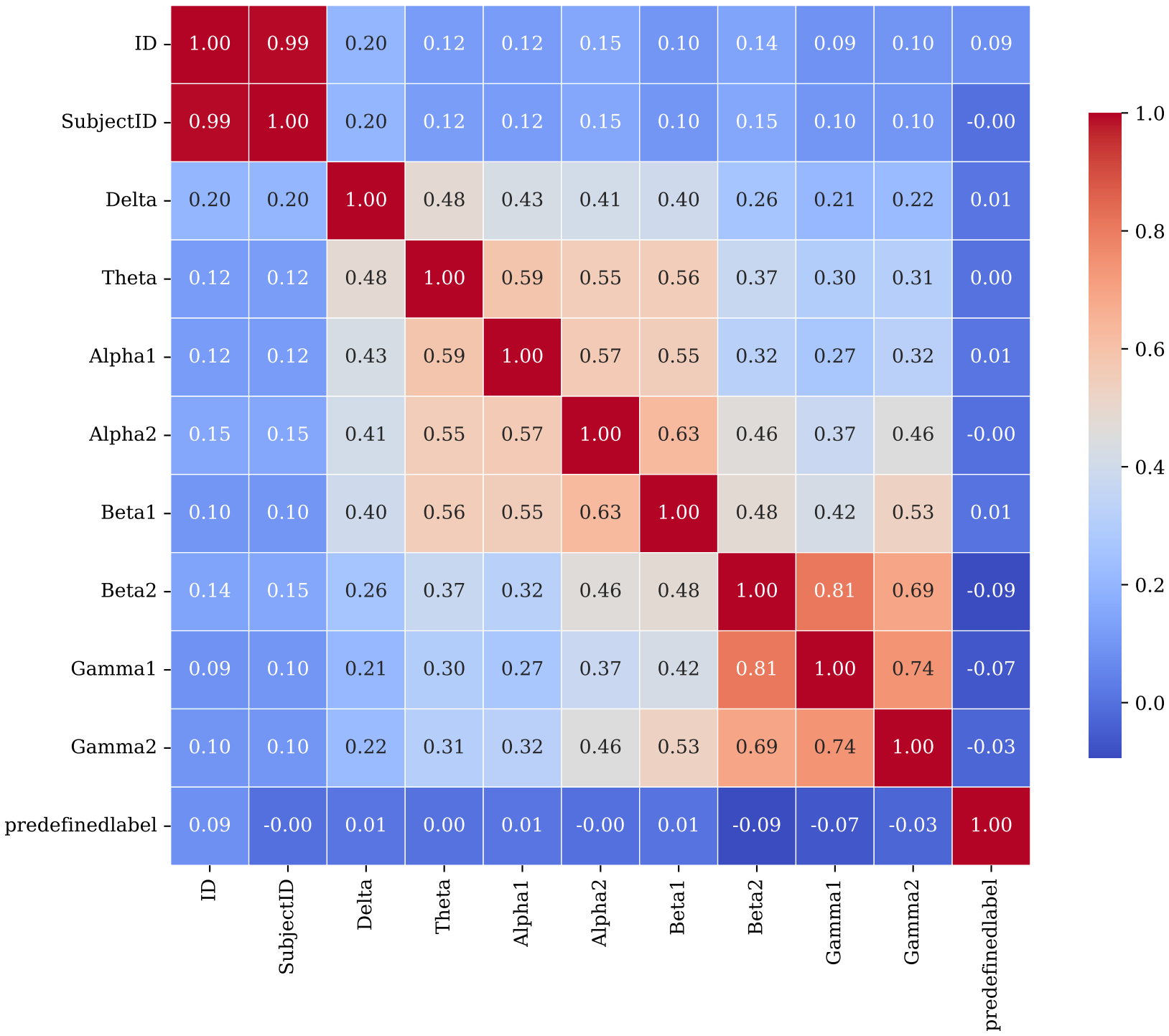
Correlation Matrix
