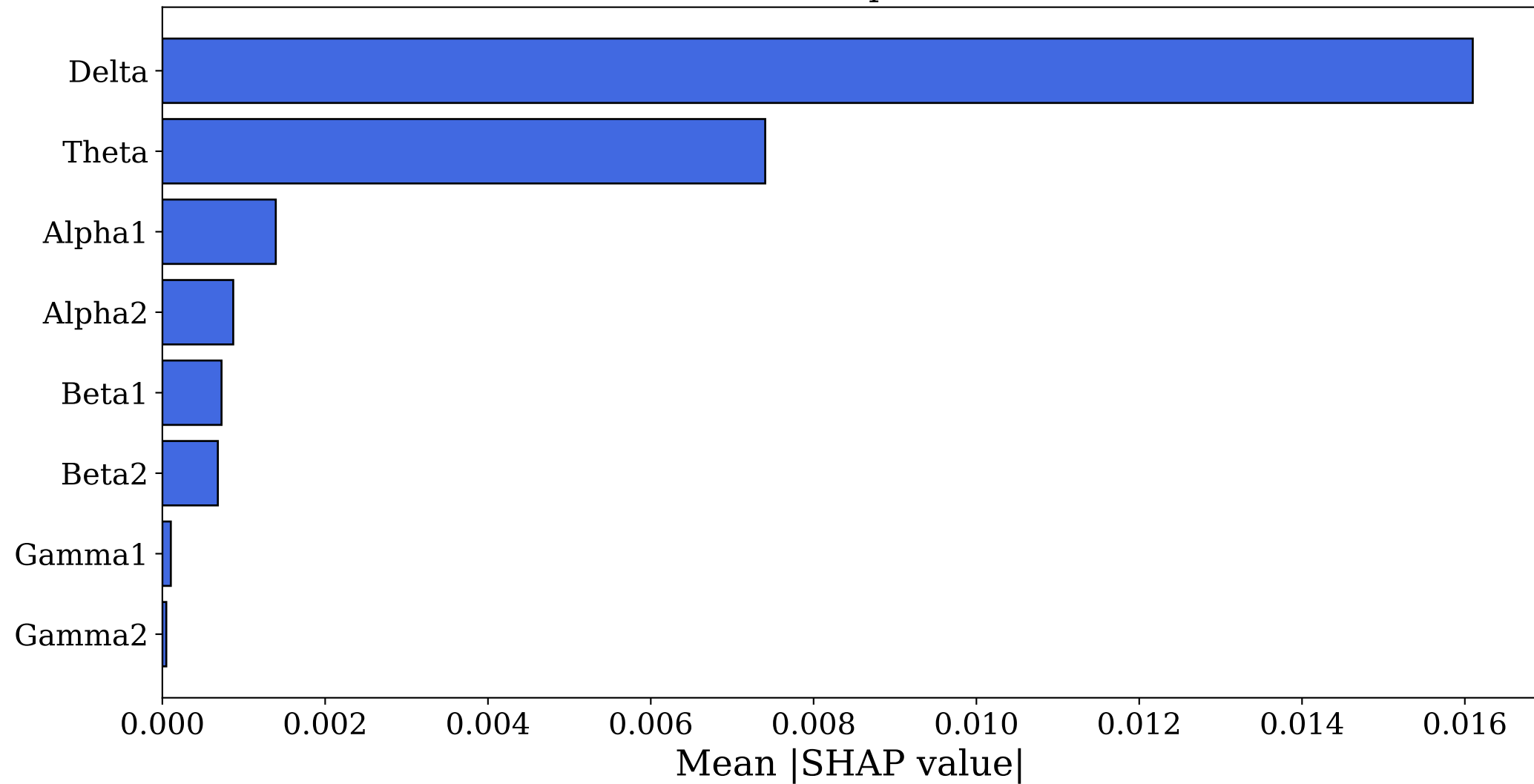
Feature Importance
