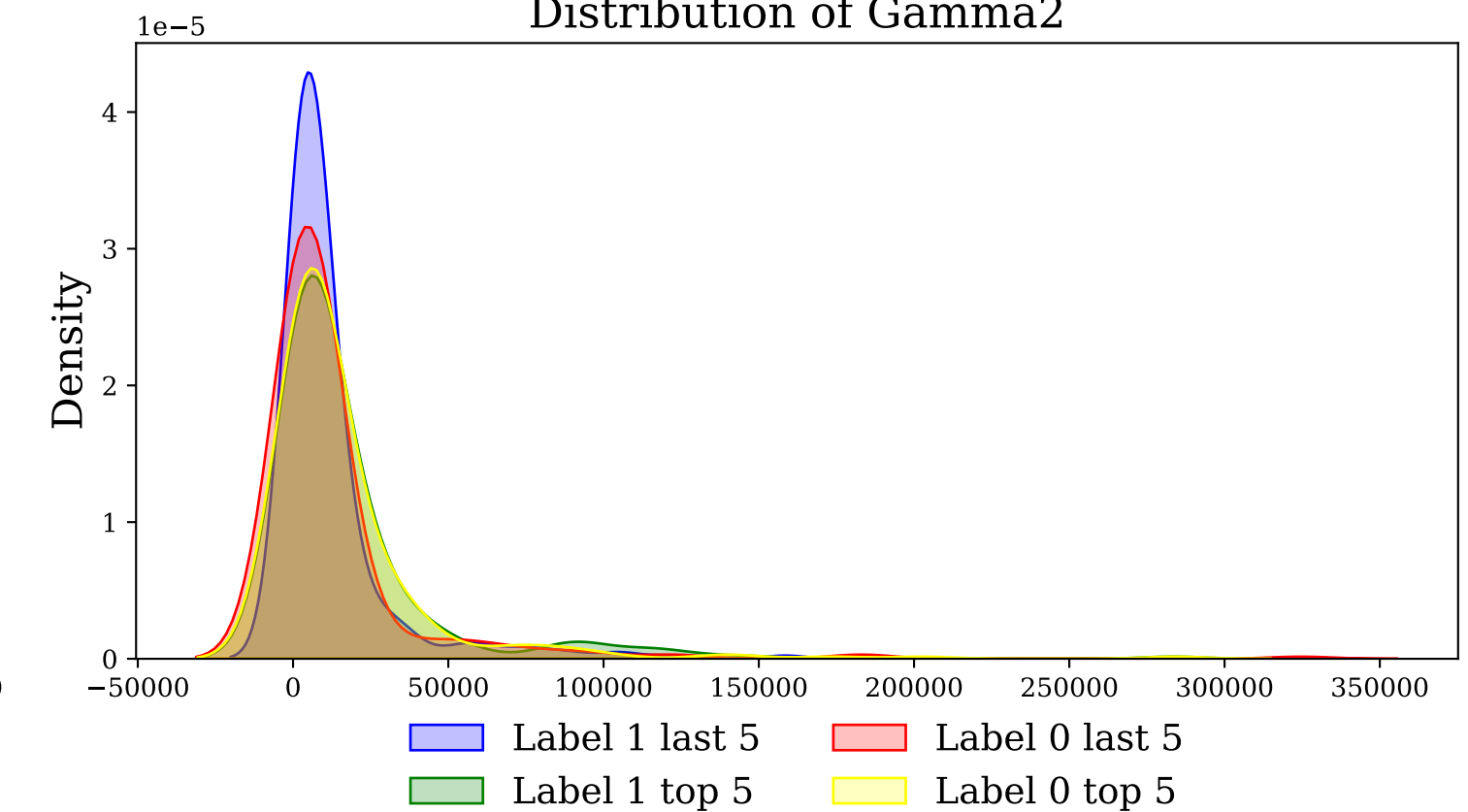
Distribution of Gamma2
