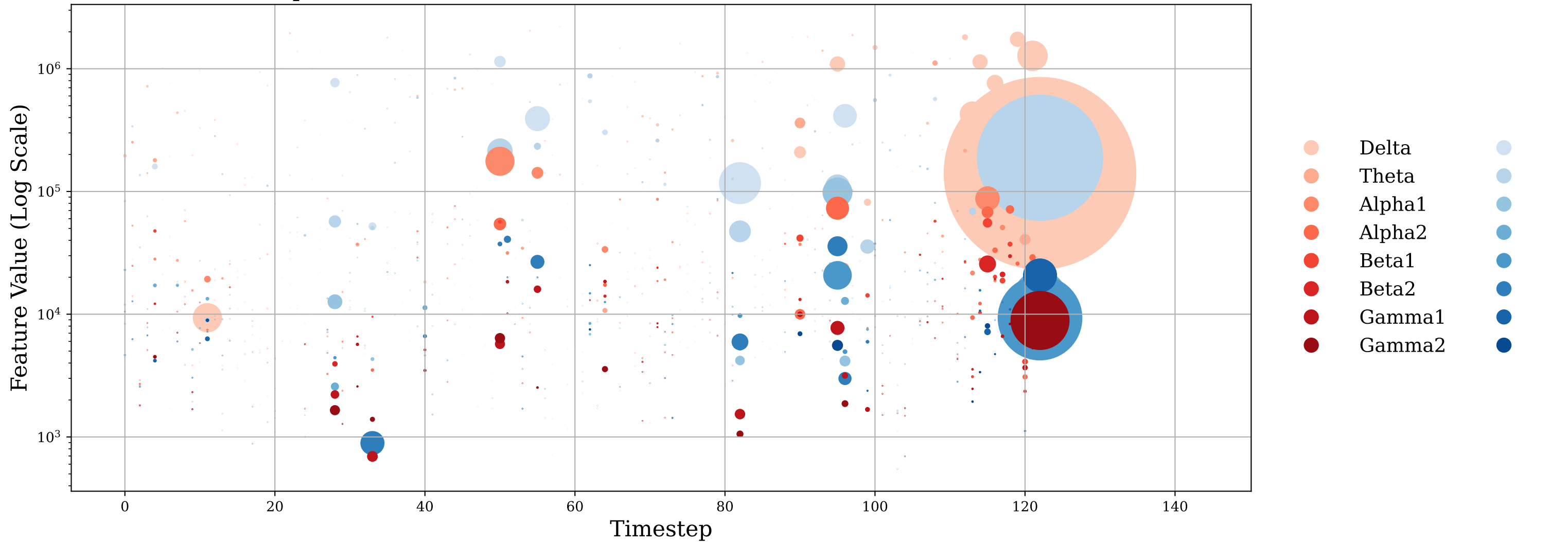
Sample 15. True value 'Confused'. Predicted 1 with 99.95% confidence
