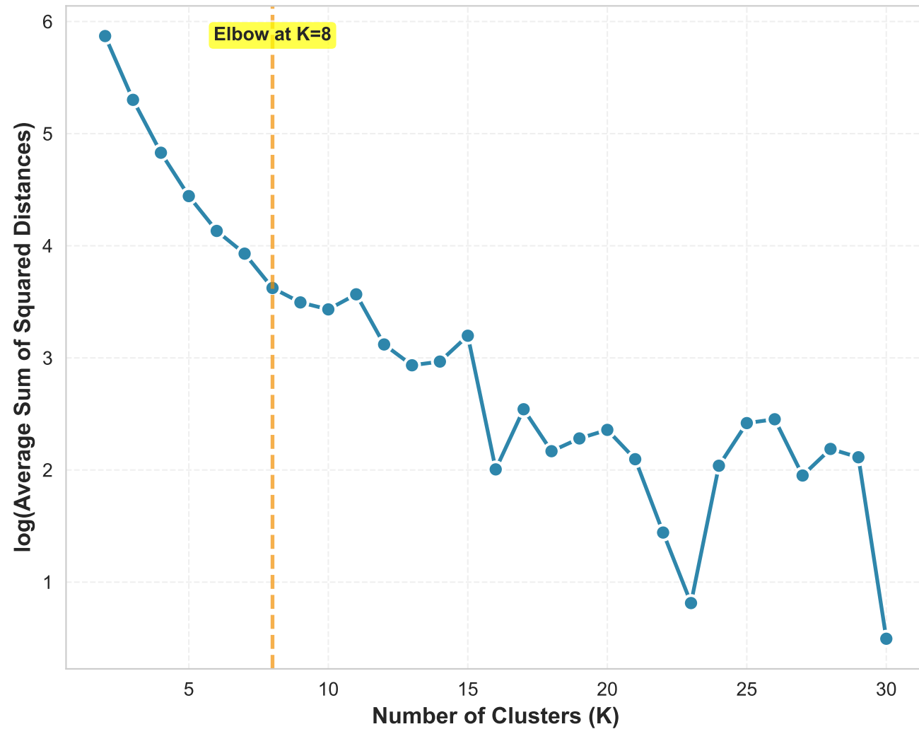
Elbow Curve
