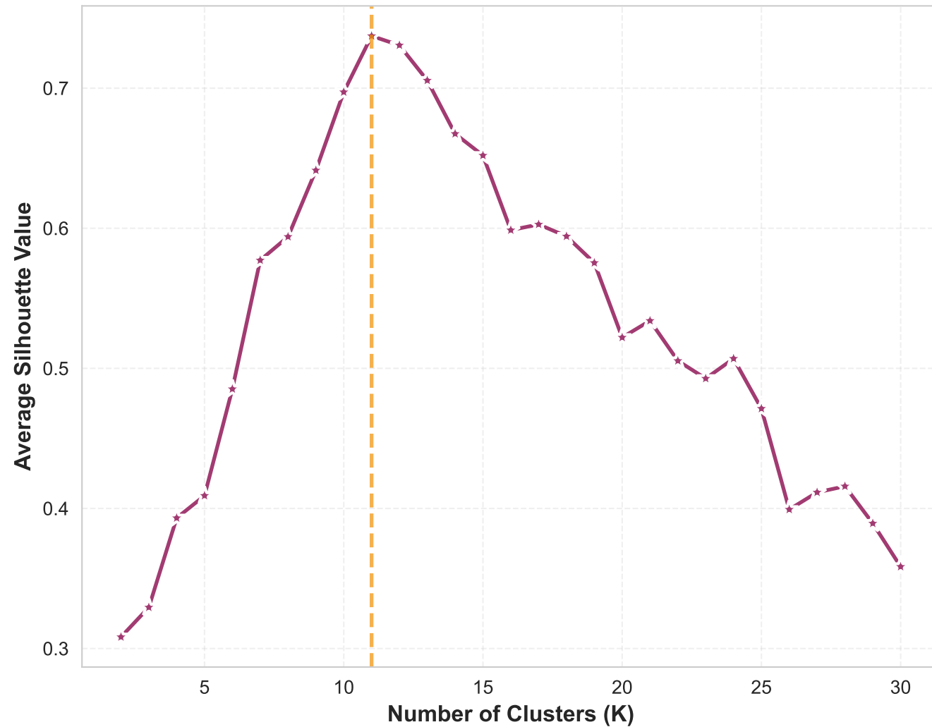
Silhouette Analysis
