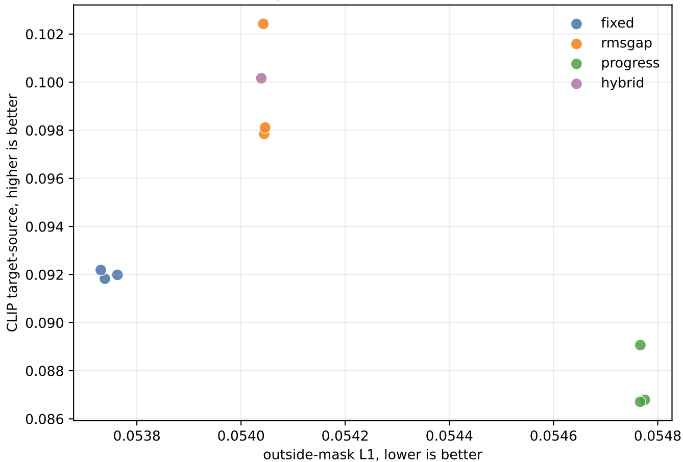
Edit-preserve tradeoff, cat crown
