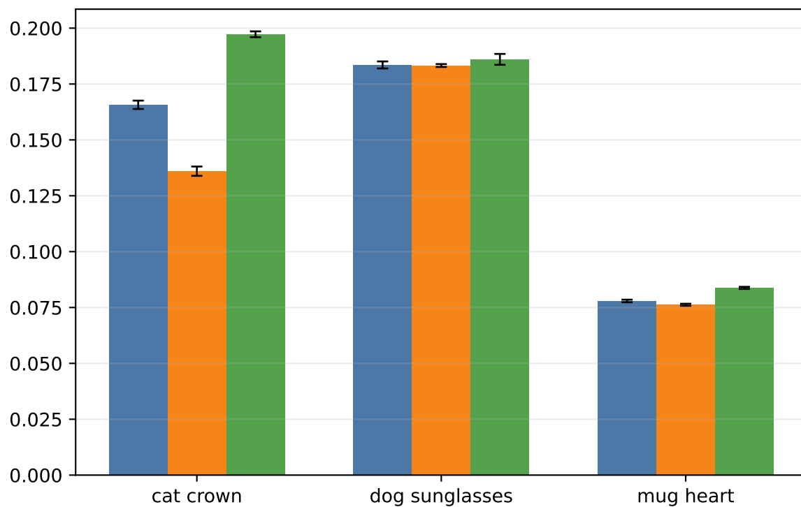
Inside L1
