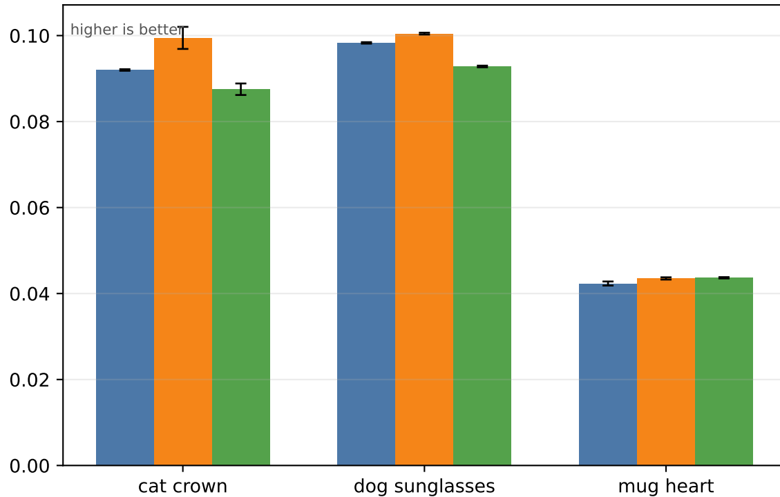
Inside L1
