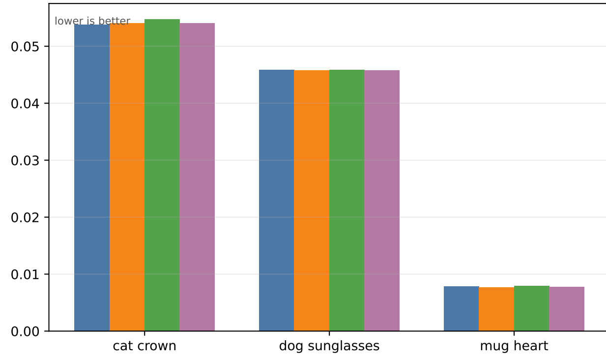
Source SSIM
