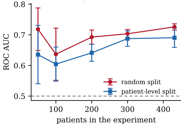
(a) estimates by sample size
