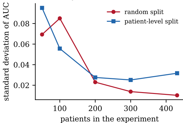
(b) stability of the estimate
