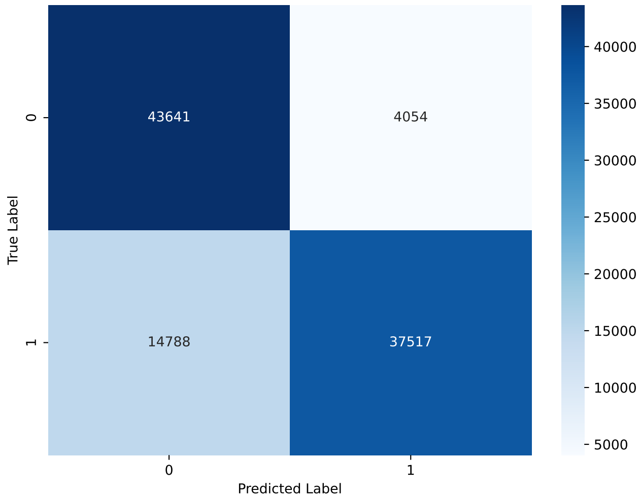
Confusion Matrix for Nb Final
