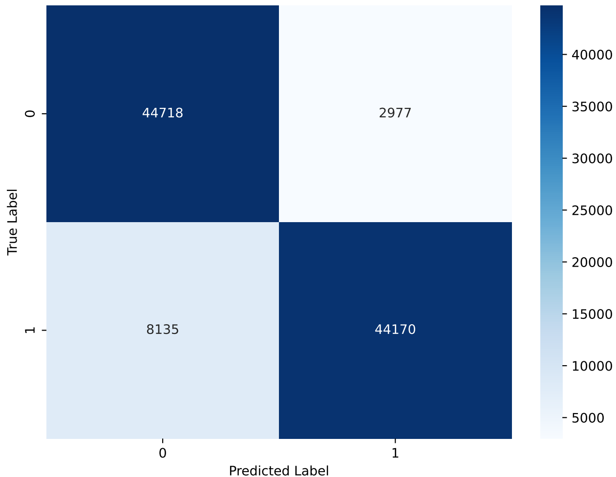
Confusion Matrix for Baseline
