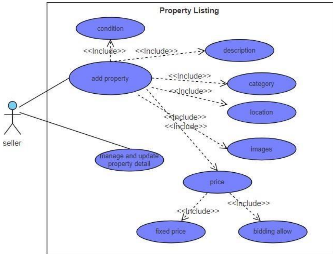
8 Figure: Use Case Diagram - Property Listing
