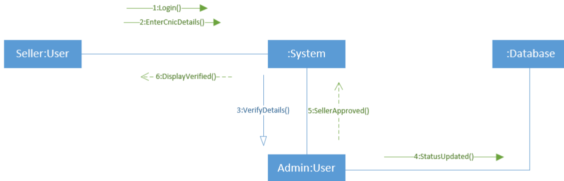
61 Figure: Collaboration Diagram - Seller's verification
