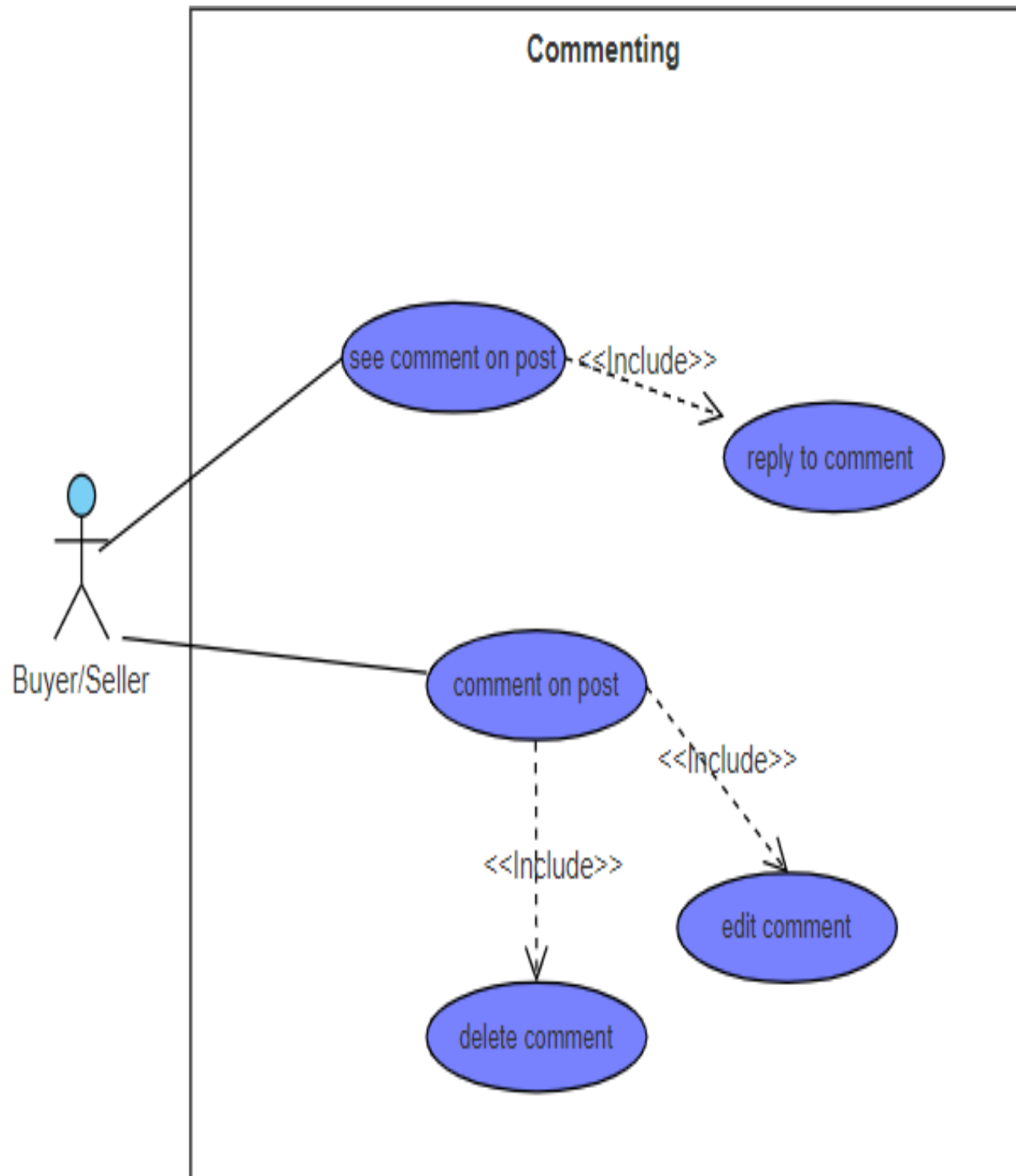
13 Figure: Use Case Diagram - Commenting
