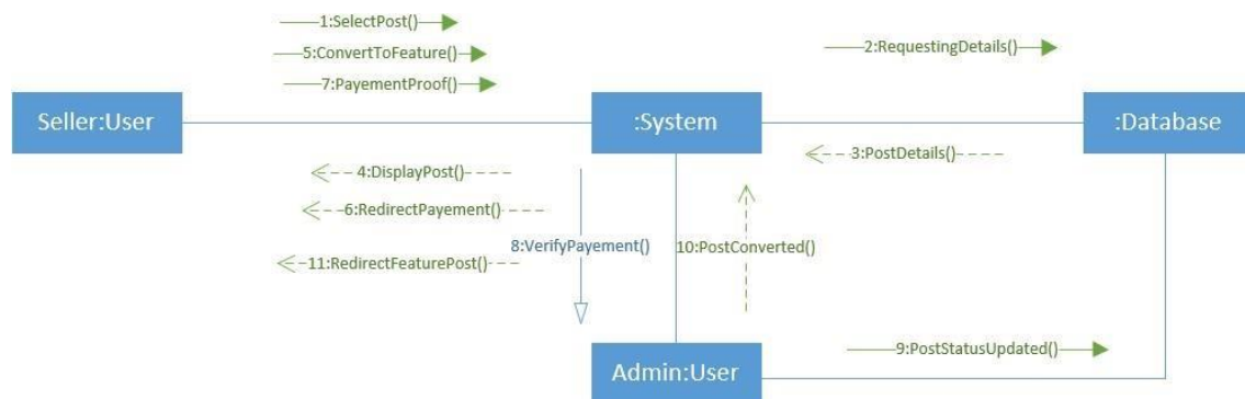
66Figure: Collaboration Diagram - Featured property
