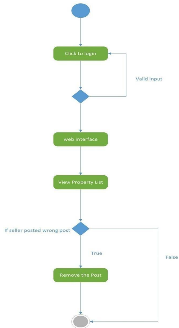
29 Figure: Activity Diagram - Action against post
