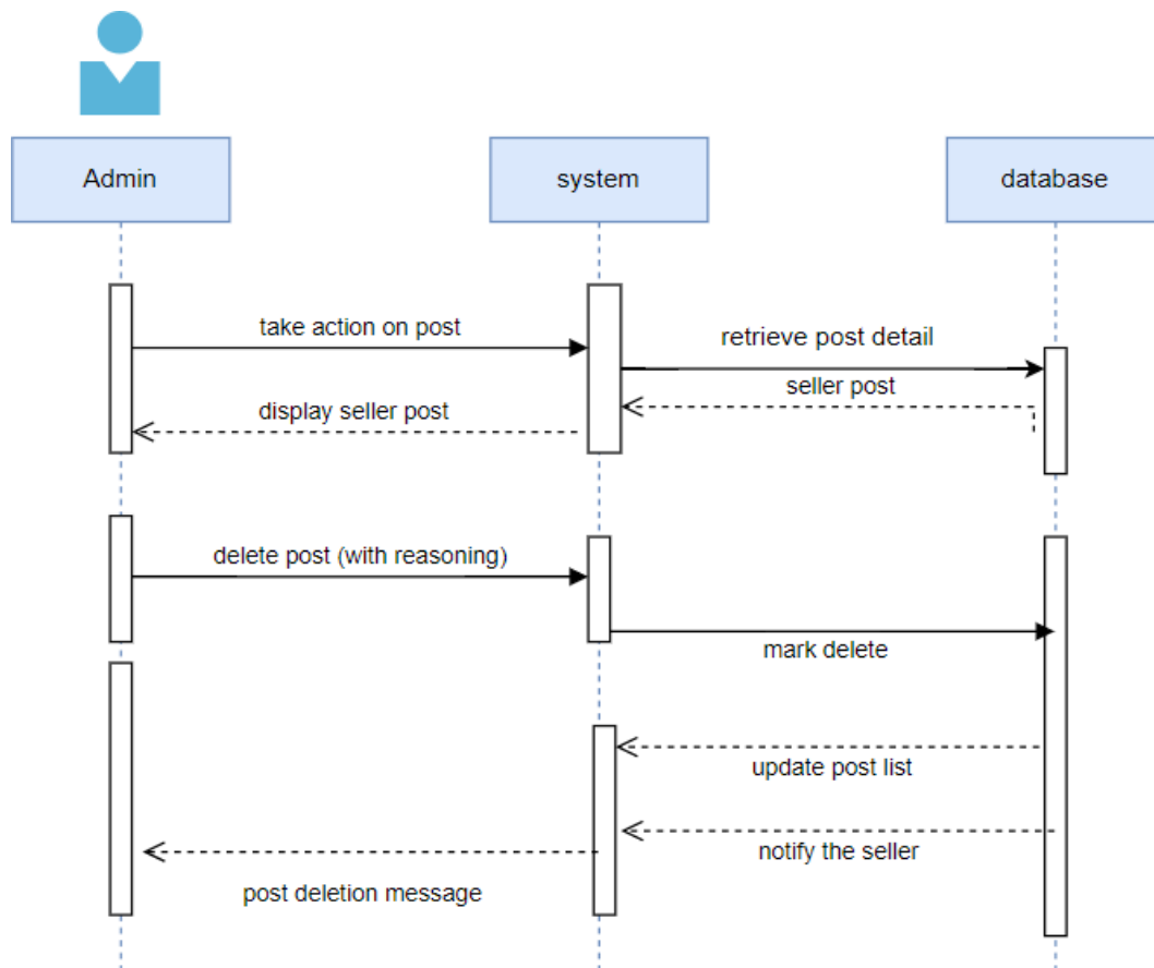
51 Figure: Sequence Diagram - Action against post
