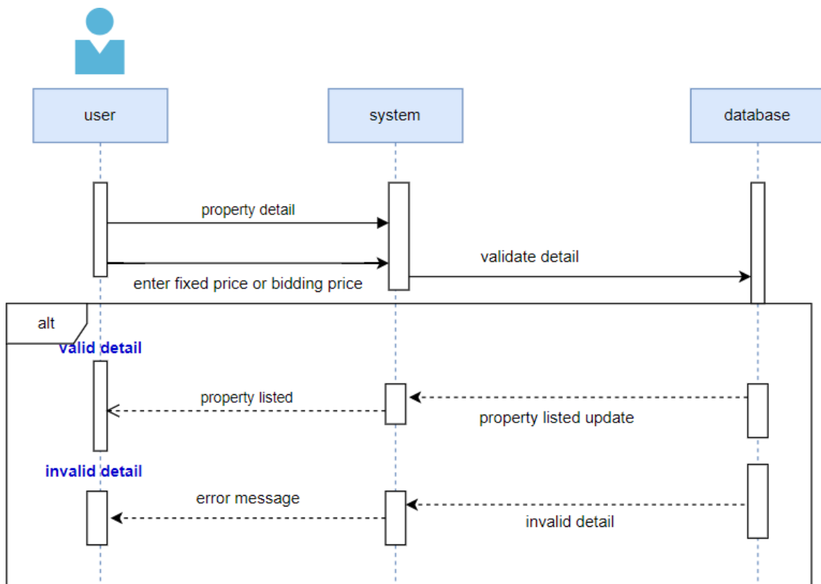
42 Figure: Sequence Diagram - Property Listing
