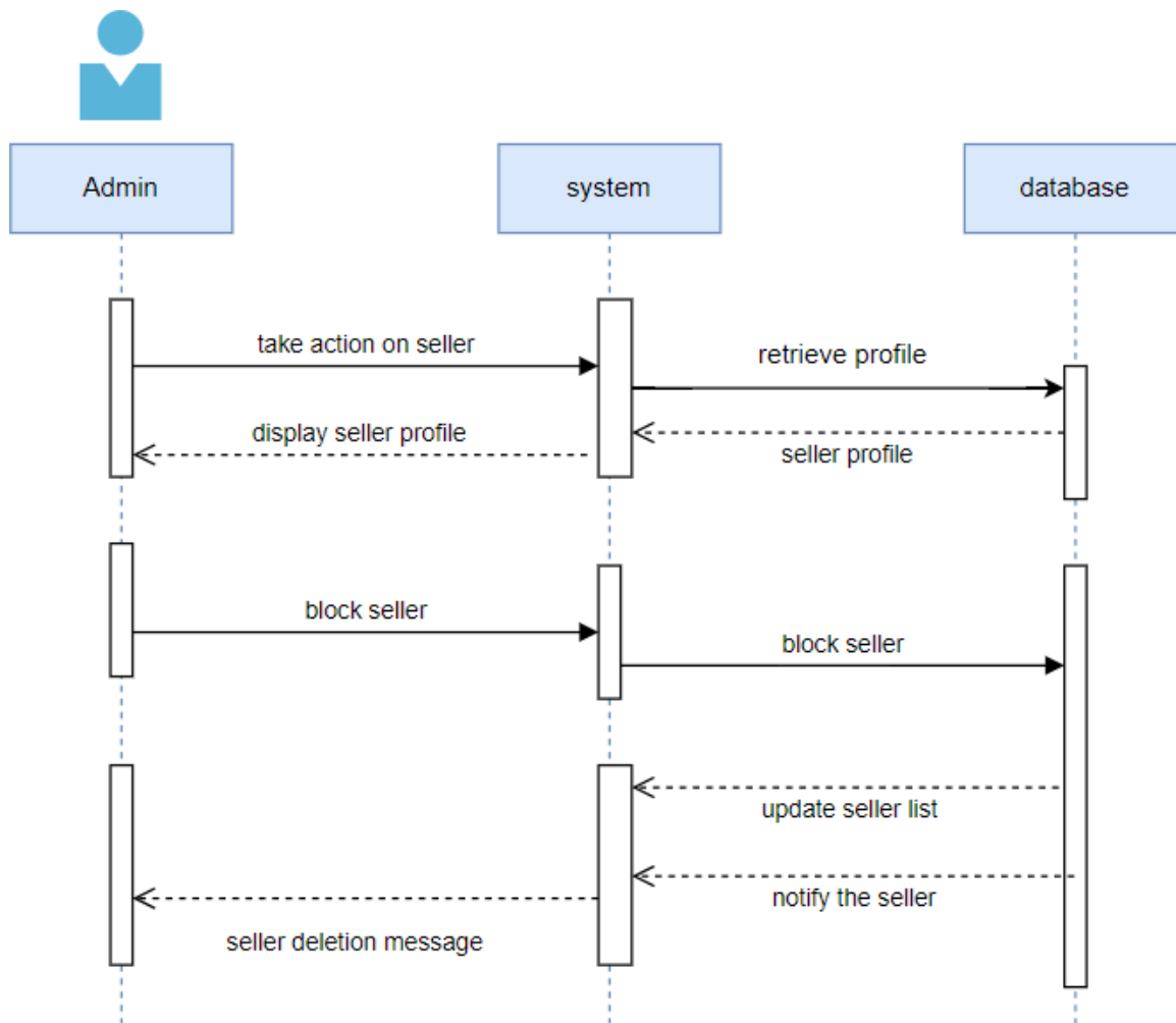
52 Figure: Sequence Diagram - Action against seller
