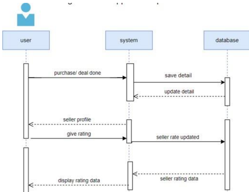
49 Figure: Sequence Diagram - Rating
