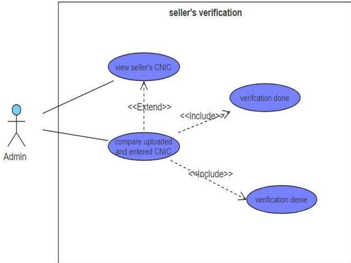
18 Figure: Use Case Diagram - Seller's Verification
