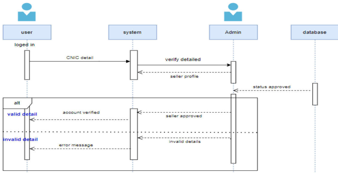
41Figure: Sequence Diagram - Become Seller
