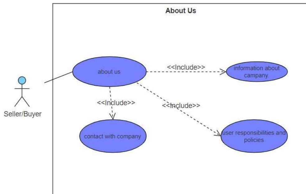
5 Figure: Use Case Diagram - About Us
