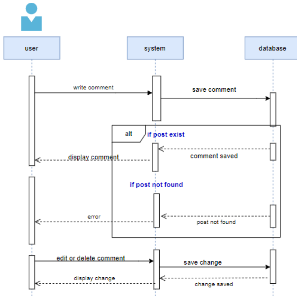
48 Figure: Sequence Diagram - Commenting
