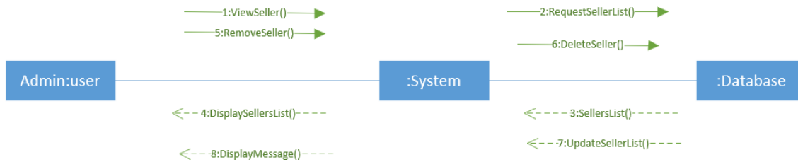
71Figure: Collaboration Diagram - Action against seller
