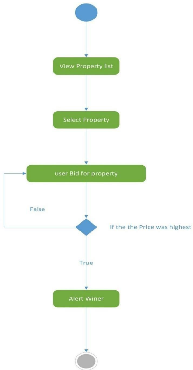
32Figure: Activity Diagram - Bidding
