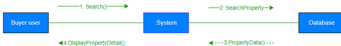
67Figure: Collaboration Diagram - Searching
