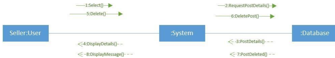
64Figure: Collaboration Diagram - Delete post
