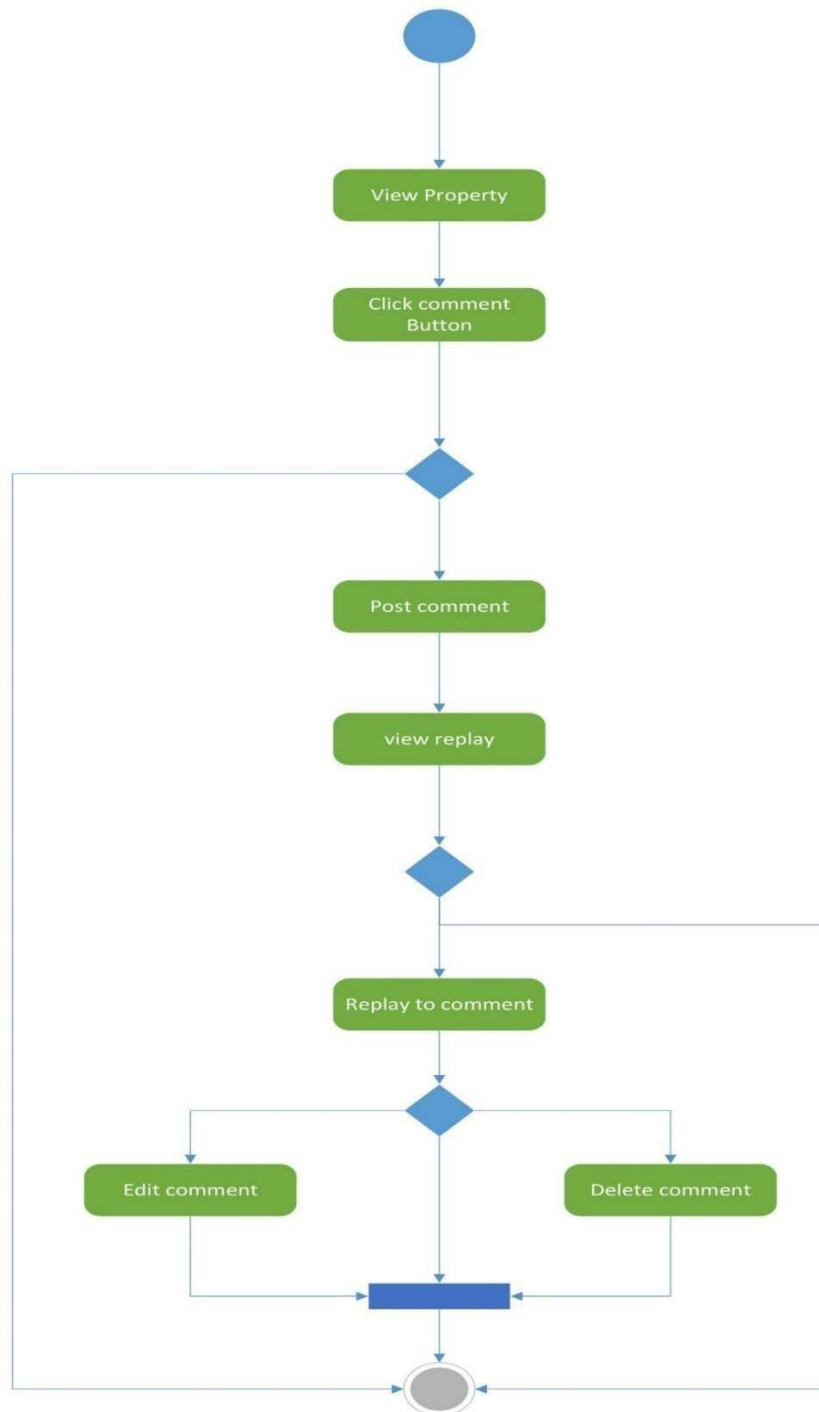
31 Figure: Activity Diagram - Commenting
