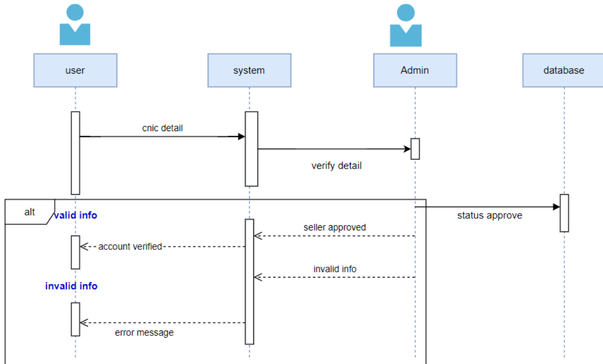
53 Figure: Sequence Diagram - Seller's Verification
