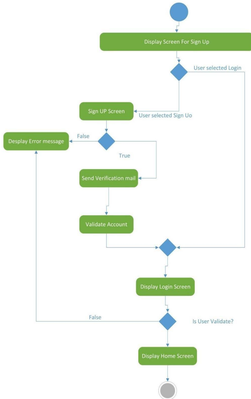
21 Figure: Activity Diagram - Sign up
