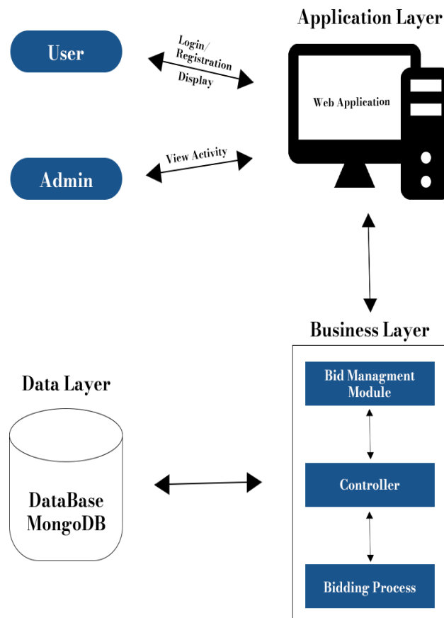
54 Figure: Software Architecture Diagram
