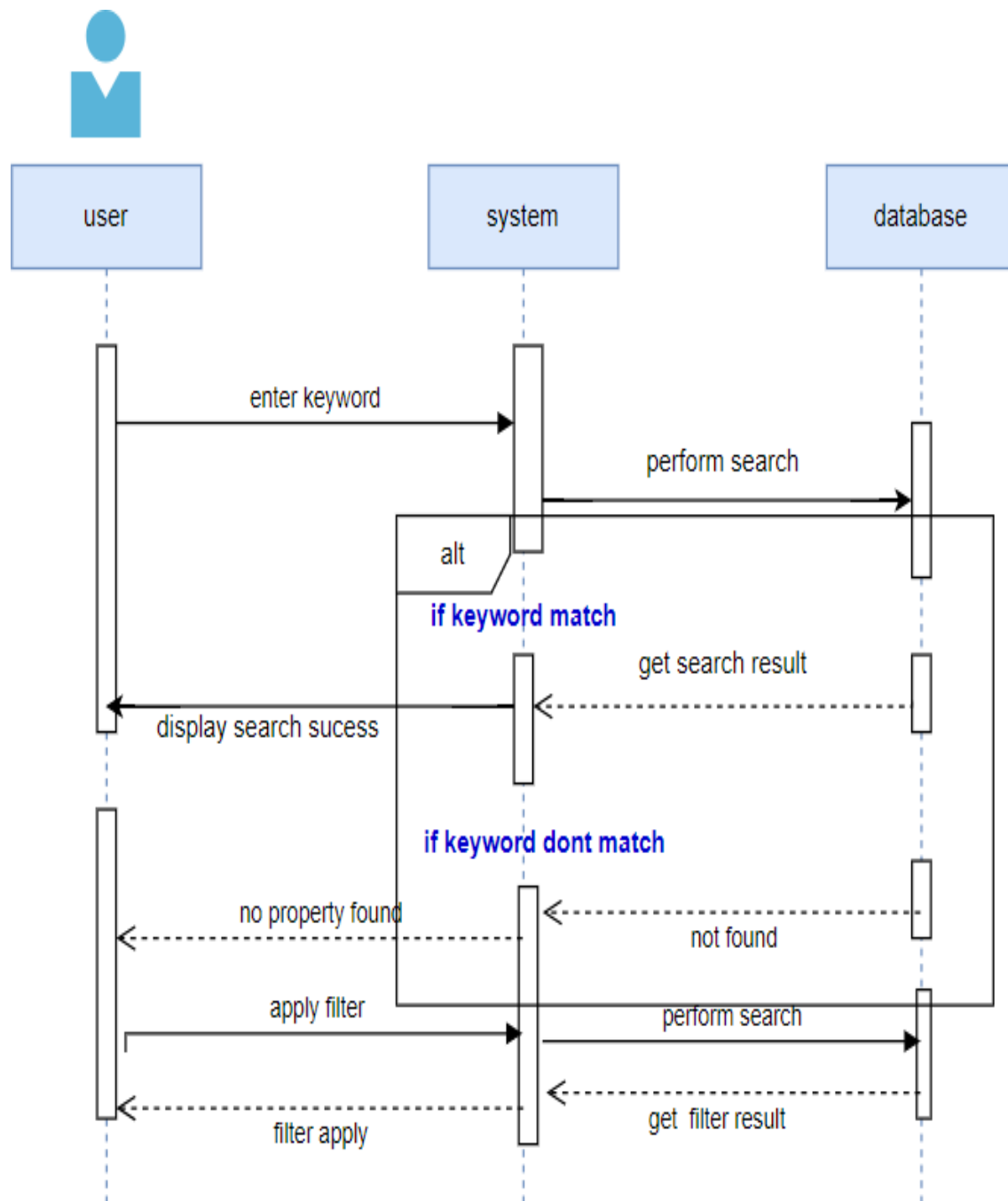
47 Figure: Sequence Diagram - Searching
