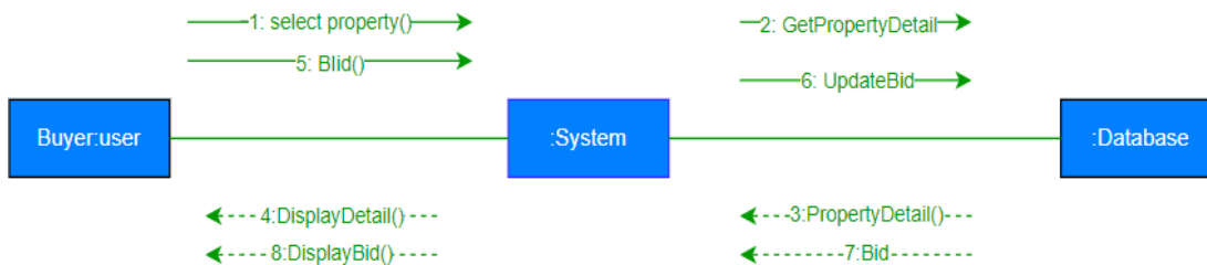
69Figure: Collaboration Diagram - Bidding
