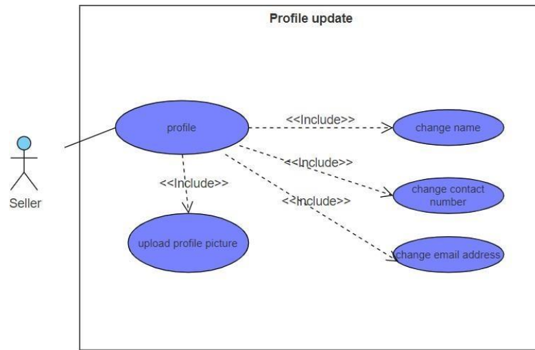
6 Figure: Use Case Diagram - Profile Update
