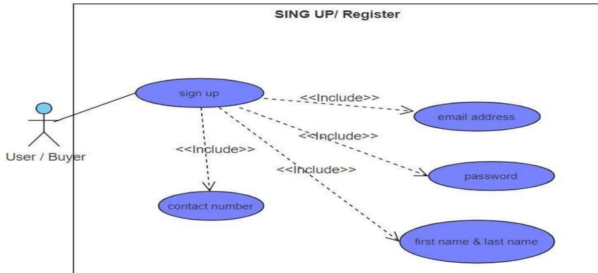
2 Figure 2: Use Case Diagram - Sign Up
