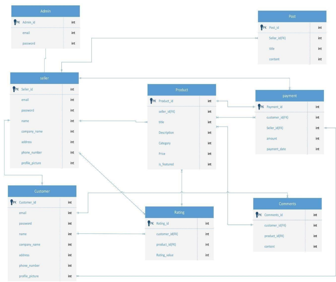
56 Figure: Database Diagram
