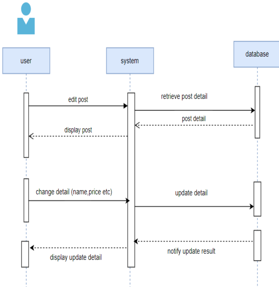
44 Figure: Sequence Diagram - Edit Post
