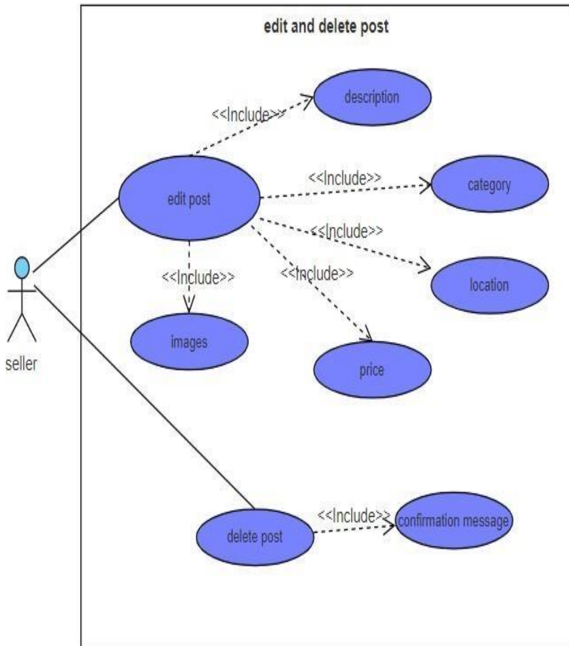
9 Figure: Use Case Diagram - Edit and Delete Post
