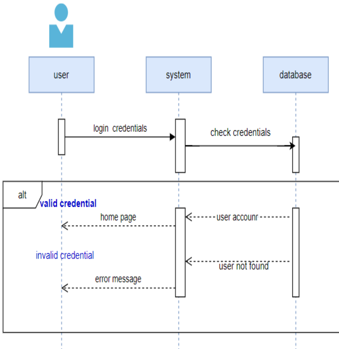
35 Figure: Sequence Diagram - Login
