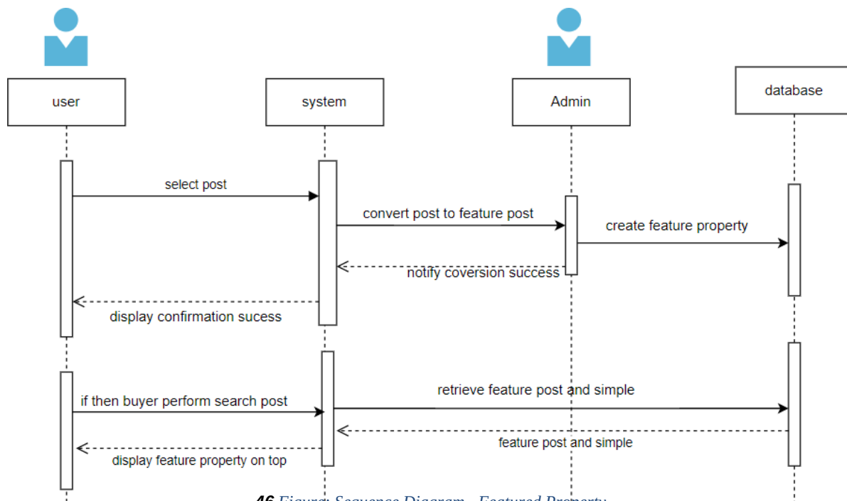
46 Figure: Sequence Diagram - Featured Property
