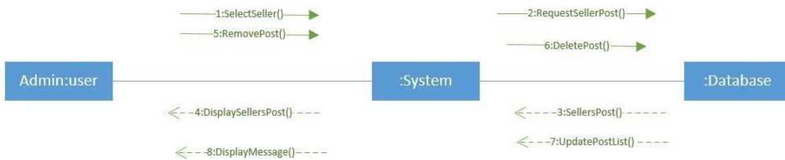
70Figure: Collaboration Diagram - Action against post
