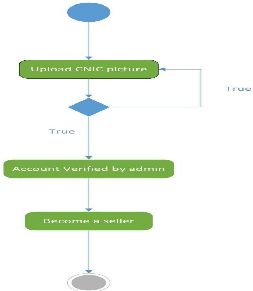
23 Figure: Activity Diagram - Become Seller
