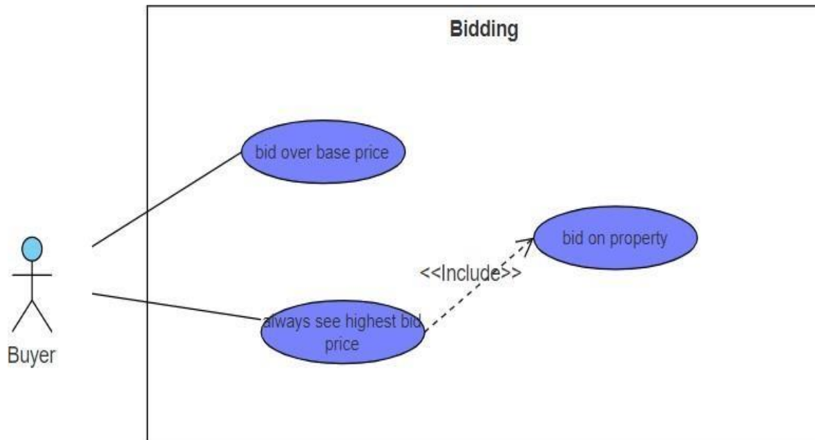
14 Figure: Use Case Diagram - Bidding
