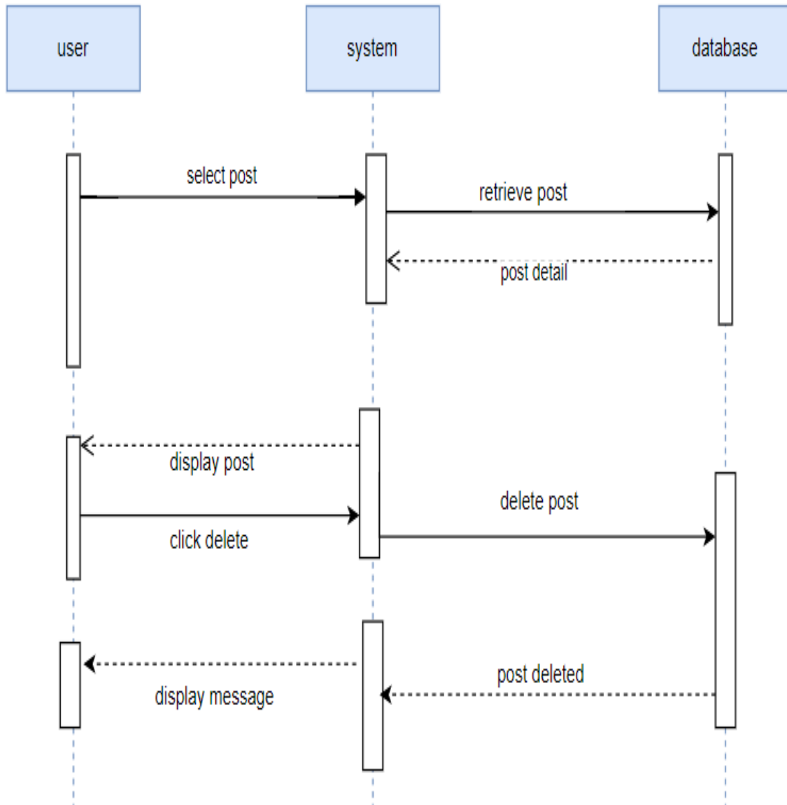
43 Figure: Sequence Diagram - Delete post
