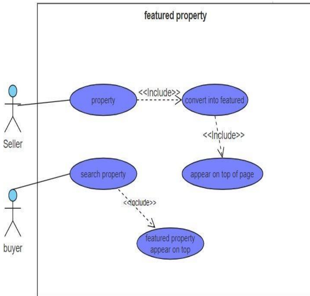
11 Figure: Use Case Diagram - Featured Property
