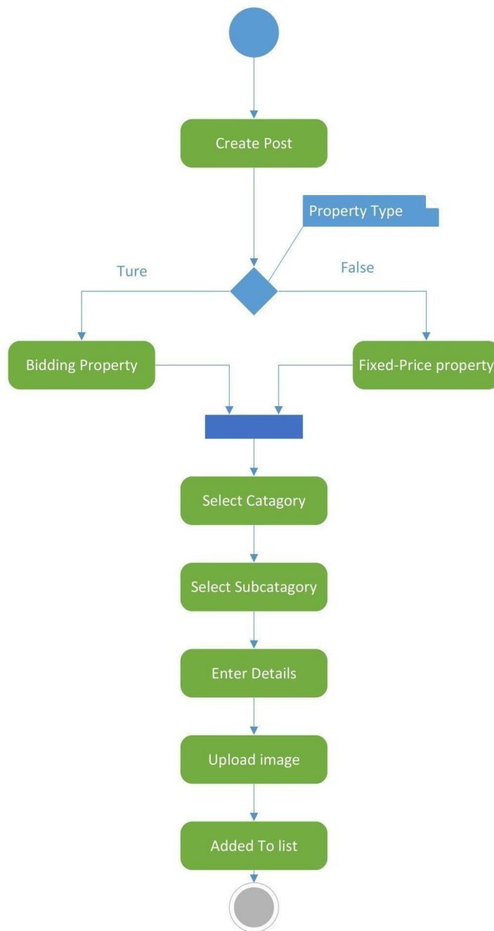
24 Figure: Activity Diagram - Property Listing
