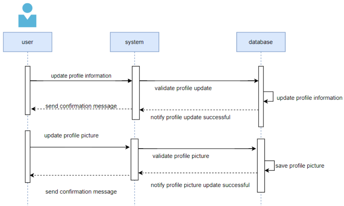
40Figure: Sequence Diagram - Profile Update
