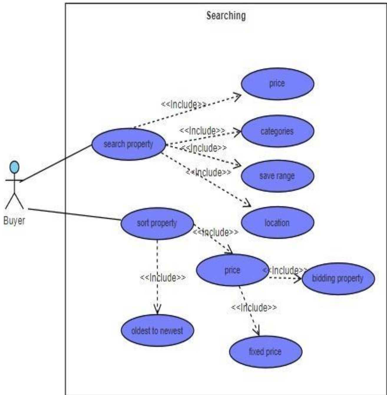
12 Figure: Use Case Diagram - Searching
