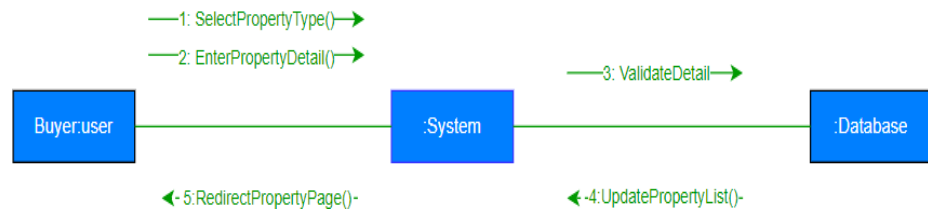
62 Figure: Collaboration Diagram - Property listing
