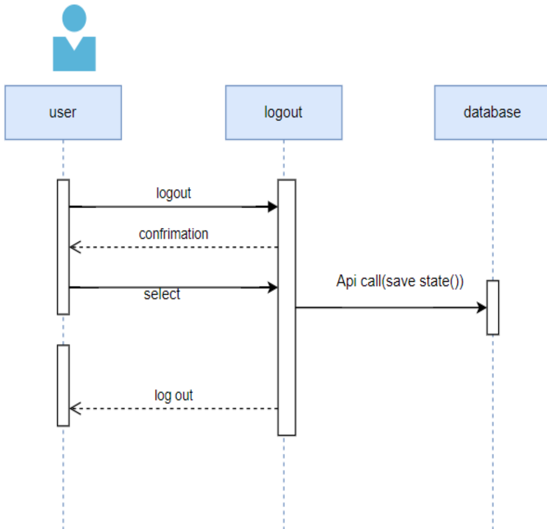
37 Figure: Sequence Diagram - Logout
