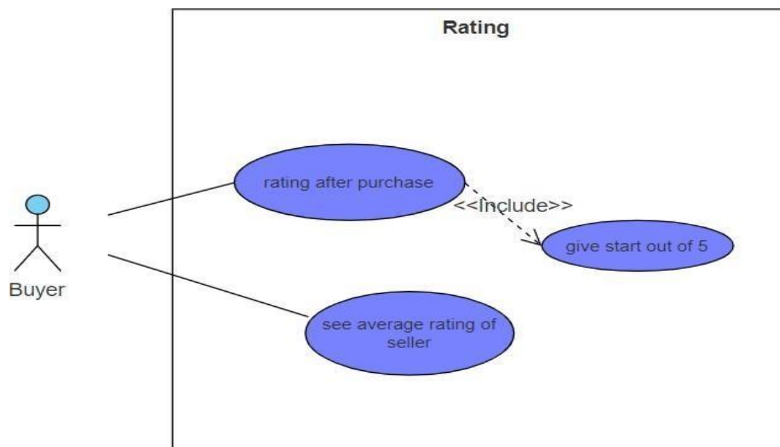
15 Figure: Use Case Diagram - Rating
