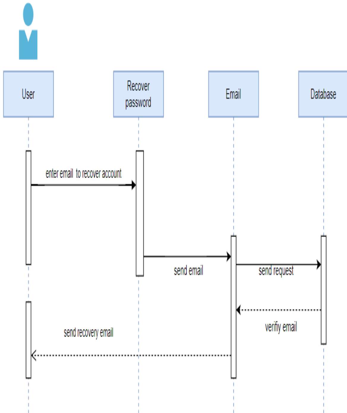
38 Figure: Sequence Diagram - Forget password
