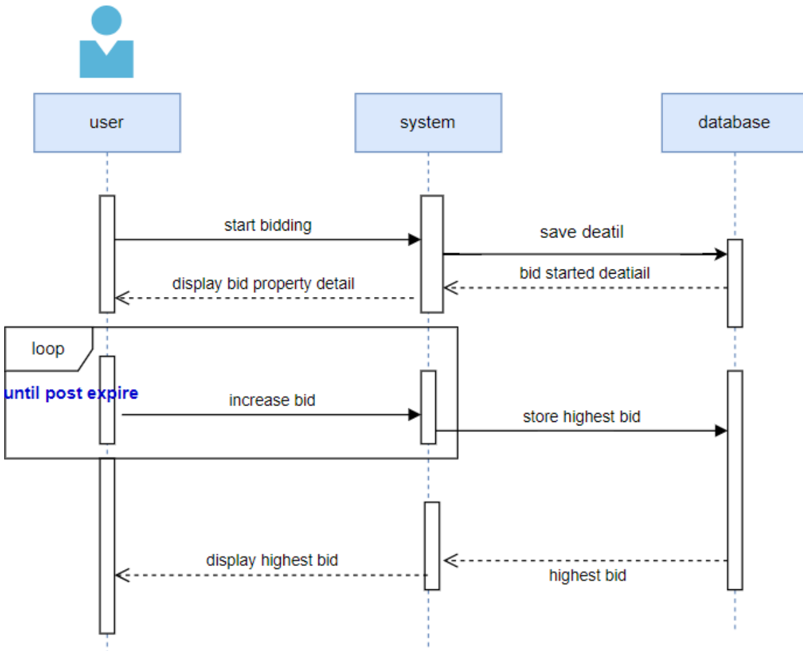
50 Figure: Sequence Diagram - Bidding
