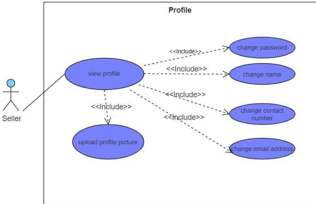
10 Figure: Use Case Diagram - Profile
