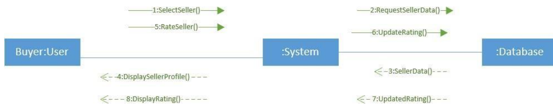
68Figure: Collaboration Diagram - Rating
