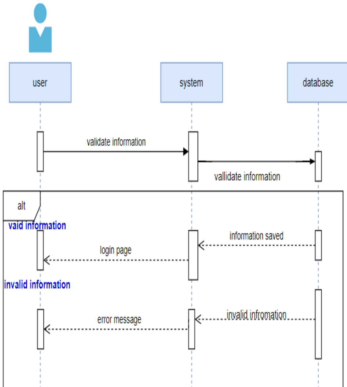
36 Figure: Sequence Diagram - Sign up
