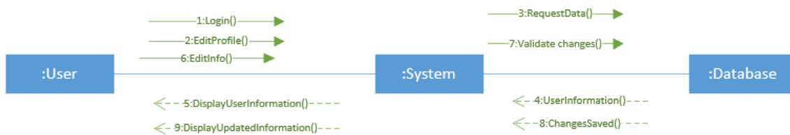
60Figure: Collaboration Diagram - Edit profile
