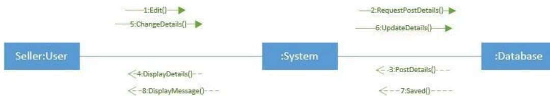
63 Figure: Collaboration Diagram - Edit post
