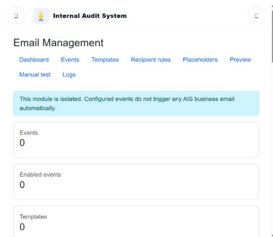
Figure 15.1: Email Management
