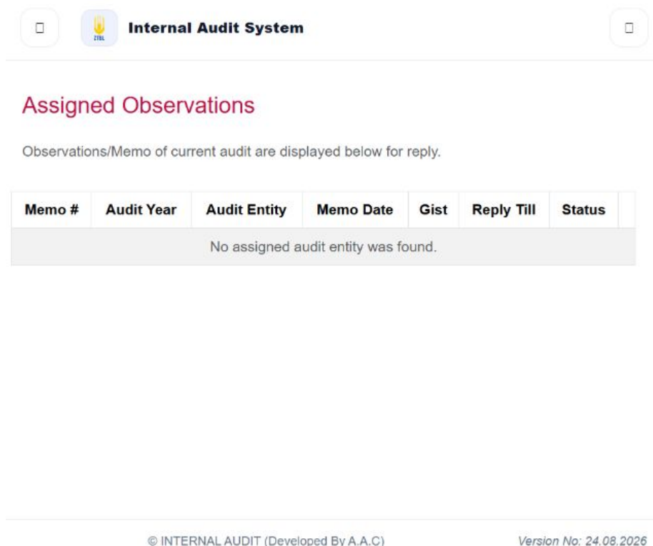
Figure 6.1: Observation Assigned
