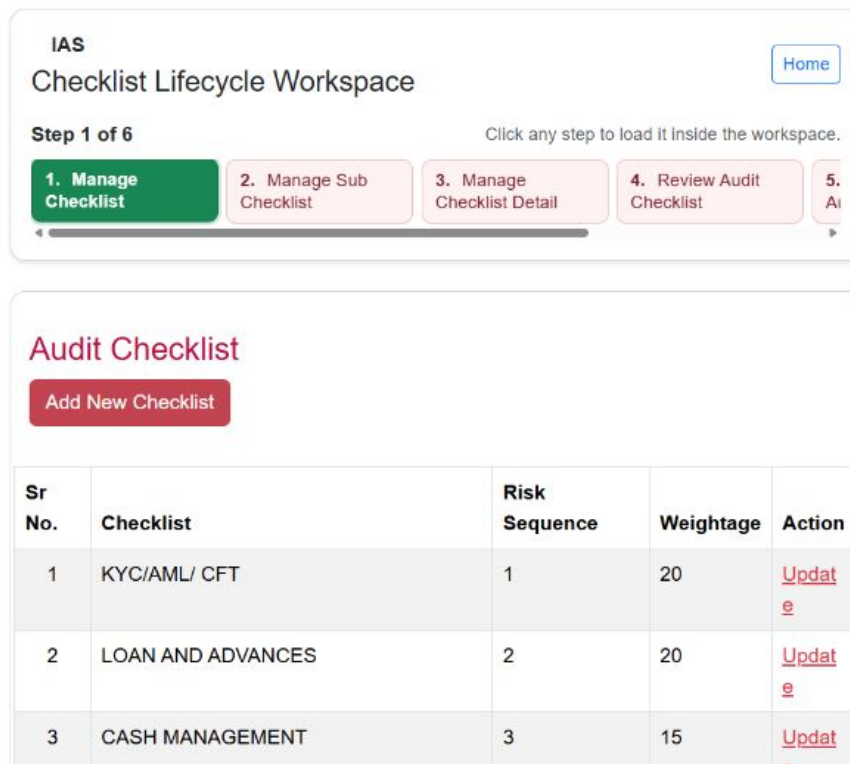
Figure 13.1: Checklist Dashboard
