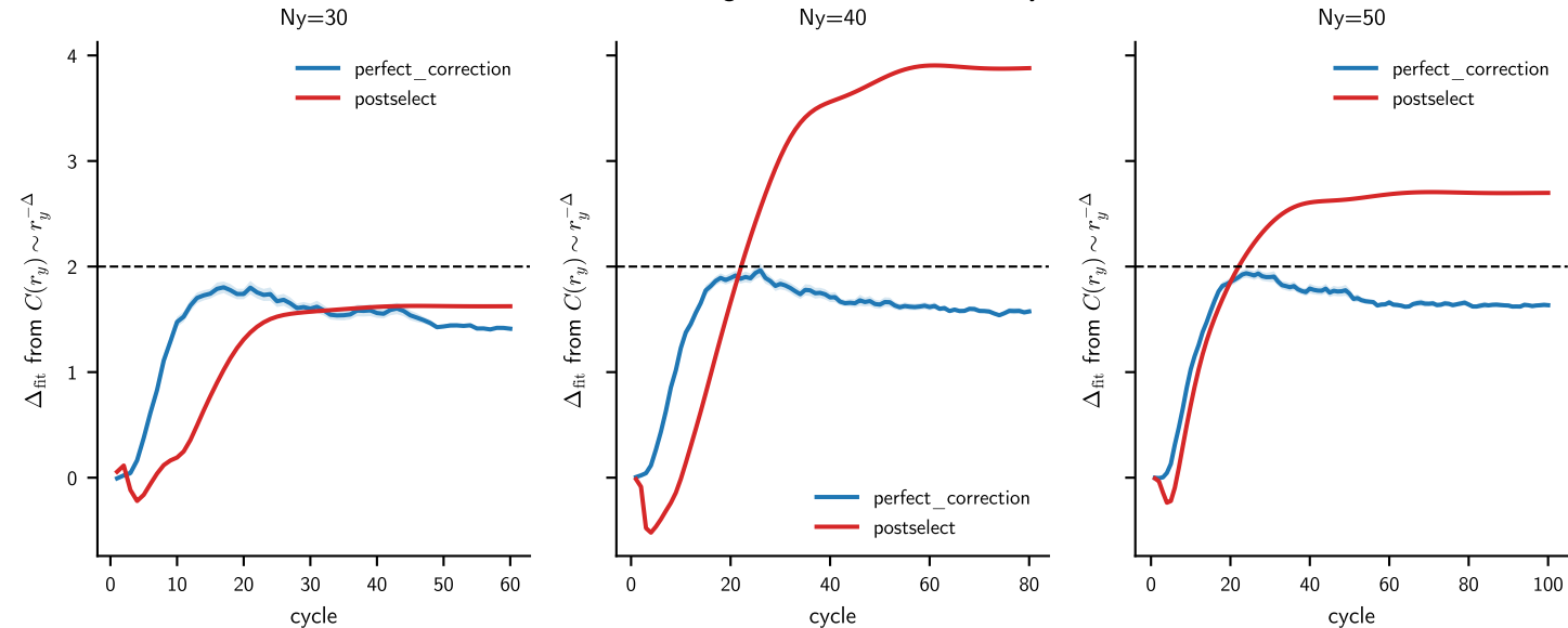
Default x-averaged correlator fits across cycle
