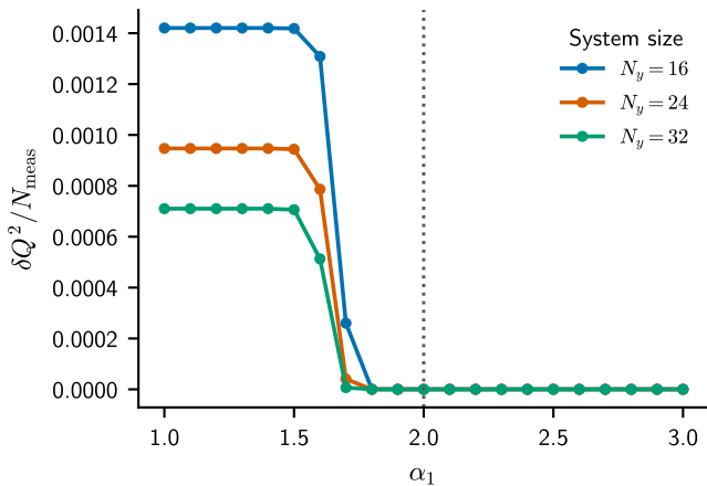
post-selection: Charge-variance density
