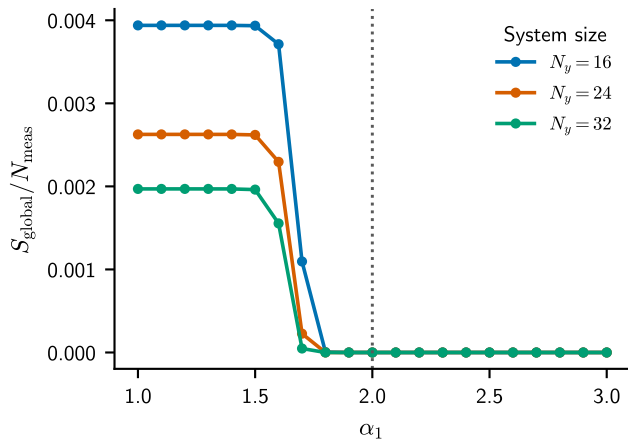
post-selection: Entropy density
