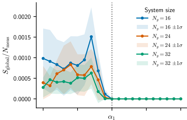
post-selection: Entropy density
