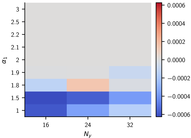
postselection: \Delta(S/N_{\text{meas}})
