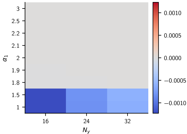
postselection: \Delta(S/N_{\text{meas}})
