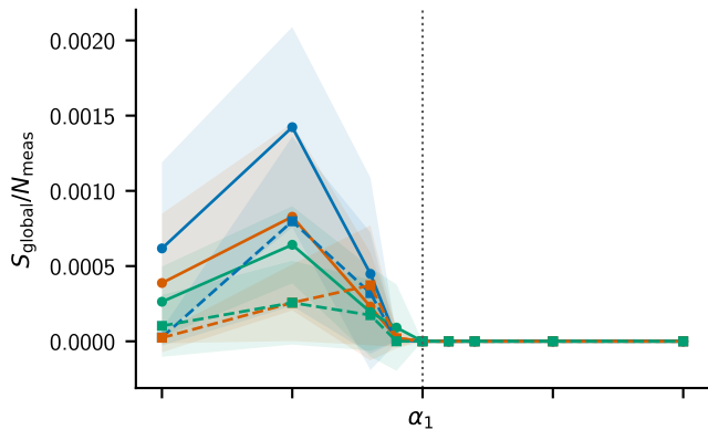
postselection: Entropy density
