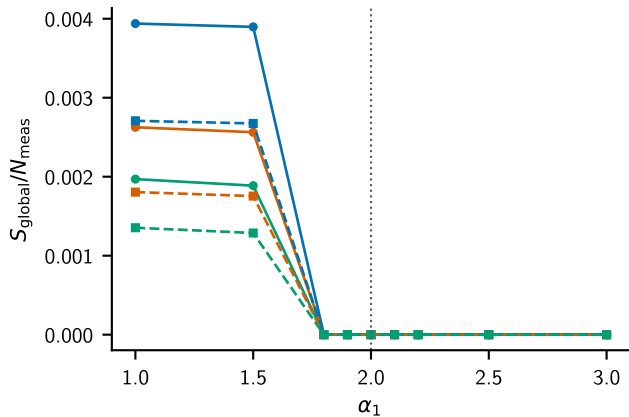
postselection: Entropy density
