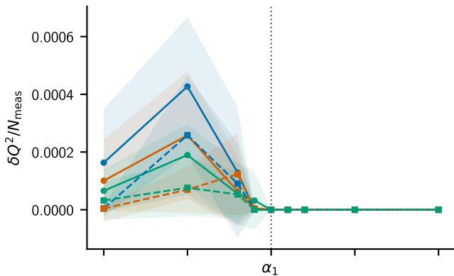
postselection: Charge-variance density
