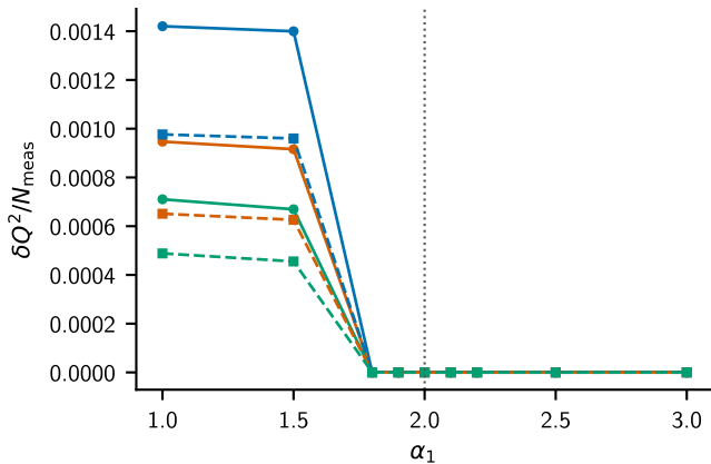
postselection: Charge-variance density
