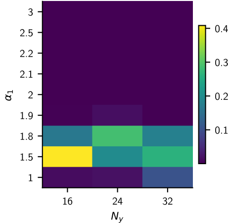
postselection, dwtrunc0: Entropy
