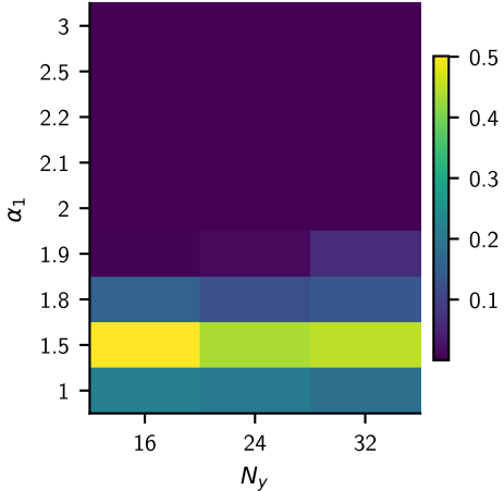
postselection, dwtrunc1: Entropy
