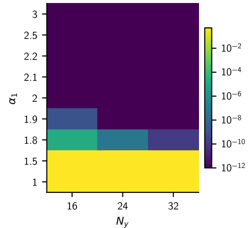
postselection, dwtrunc0: Charge variance
