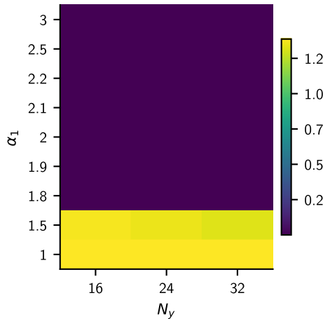
postselection, dwtrunc0: Entropy
