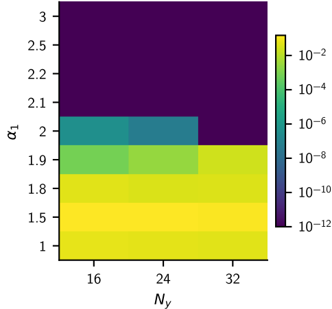
postselection, dwtrunc1: Charge variance
