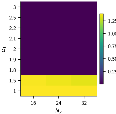
postselection, dwtrunc1: Entropy
