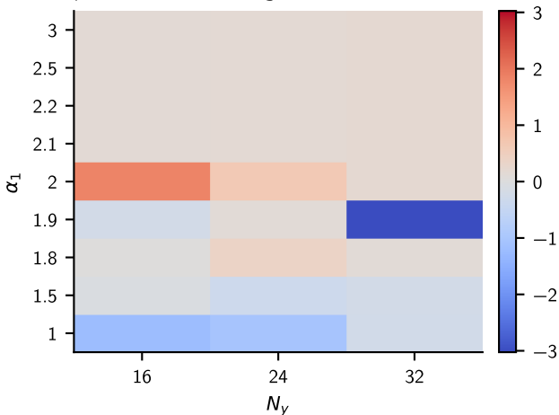
postselection: \log_{10} [(S_0 + \epsilon)/(S_1 + \epsilon)]
