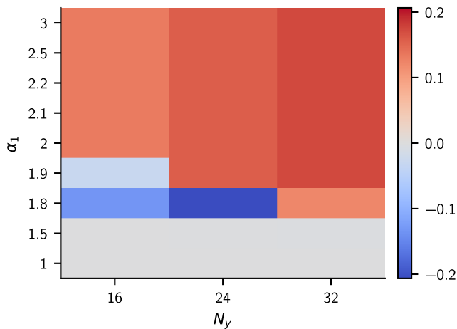
postselection: \log_{10} [(S_0 + \epsilon)/(S_1 + \epsilon)]
