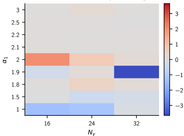
postselection: \log_{10} [(\delta Q_0^2 + \epsilon)/(\delta Q_1^2 + \epsilon)]
