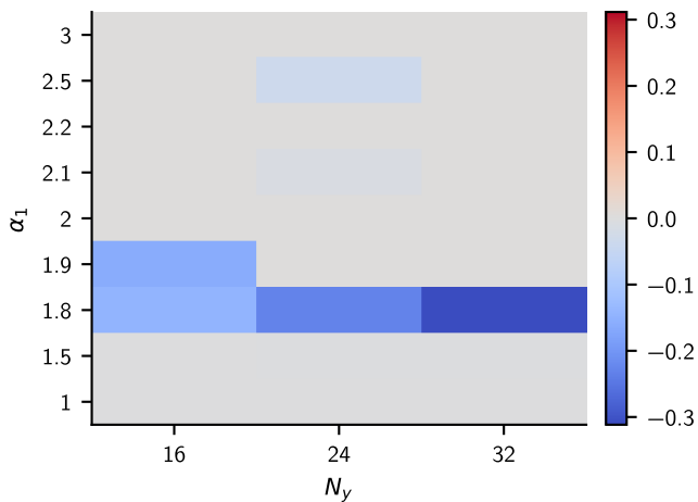
postselection: \log_{10} [(\delta Q_0^2 + \epsilon)/(\delta Q_1^2 + \epsilon)]
