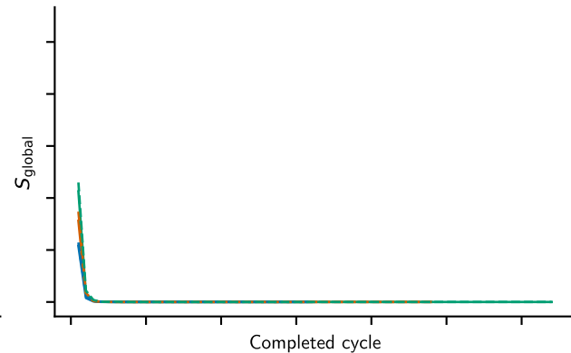
postselection, \alpha_1 = 3
