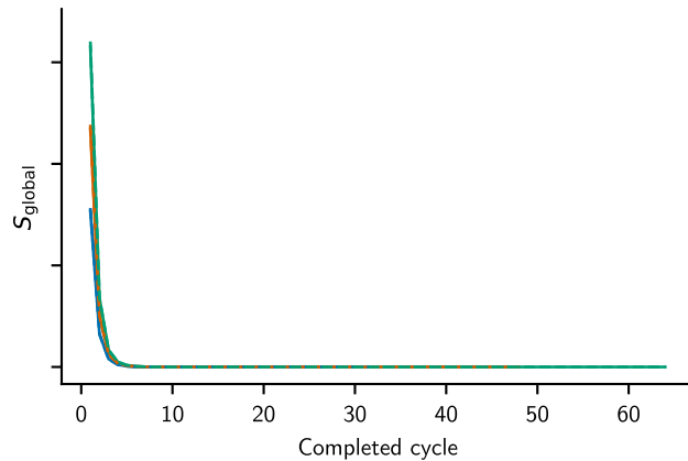
postselection, \alpha_1 = 2
