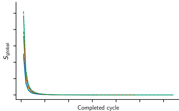
postselection, \alpha_1 = 2
