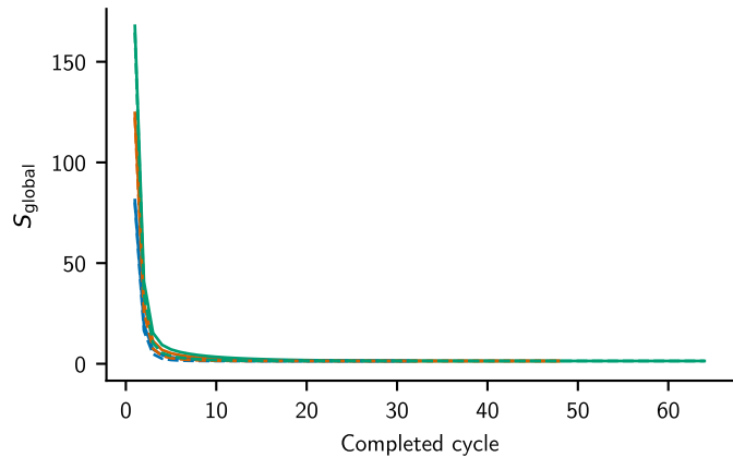
postselection, \alpha_1 = 1
