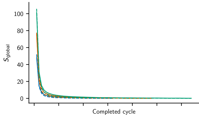
postselection, \alpha_1 = 1
