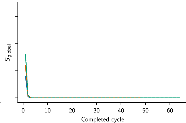
postselection, \alpha_1 = 3
