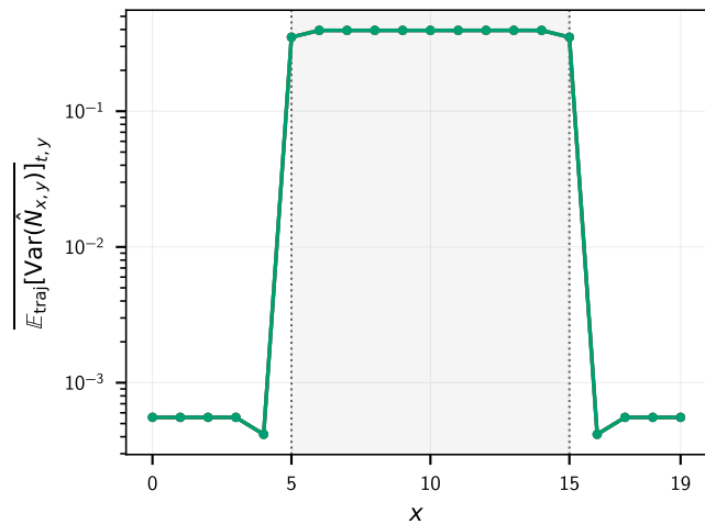
(c) Within-trajectory quantum variance
