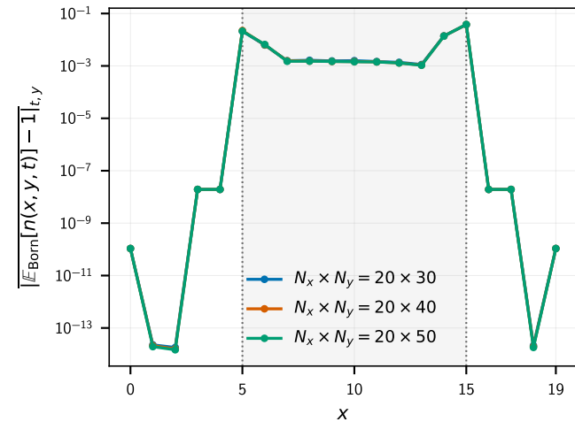
(a) Ensemble-mean occupancy bias
