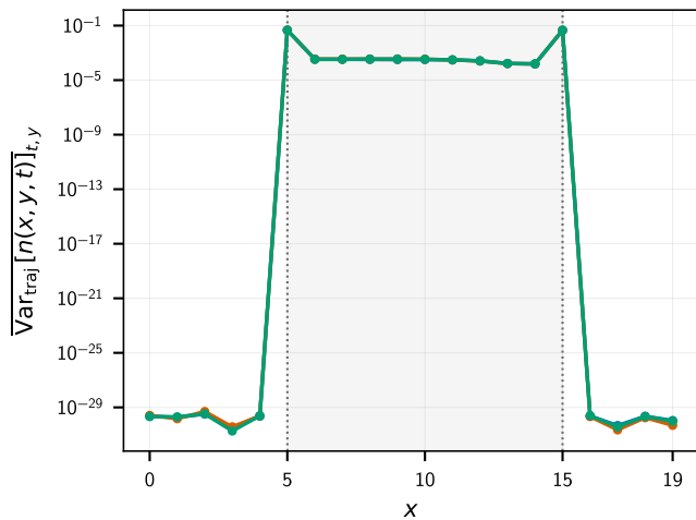
(b) Between-trajectory variance
