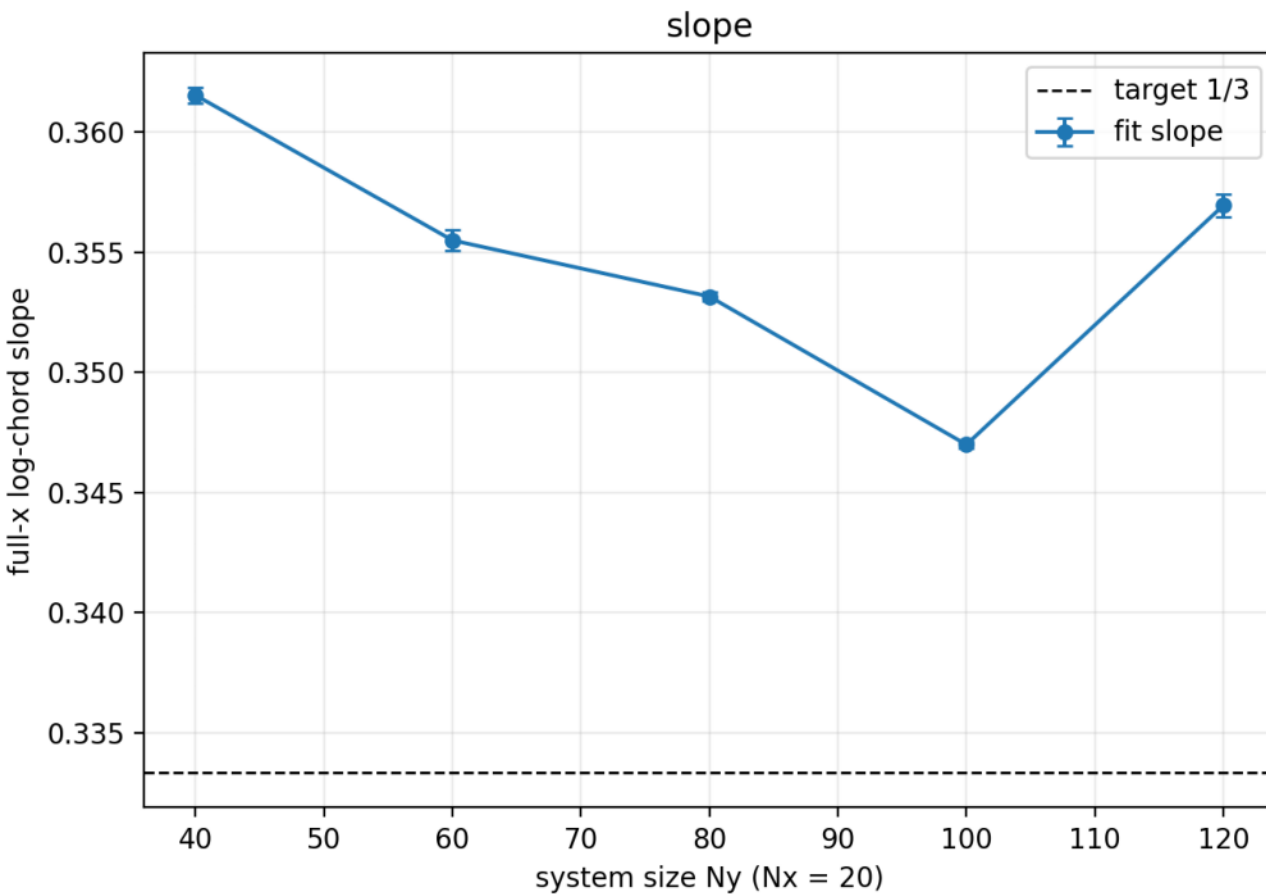
Pure-state entanglement fit quality vs system size
