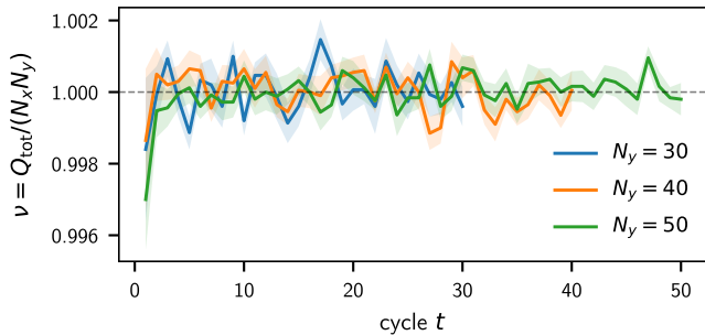
post-selection, DW off
