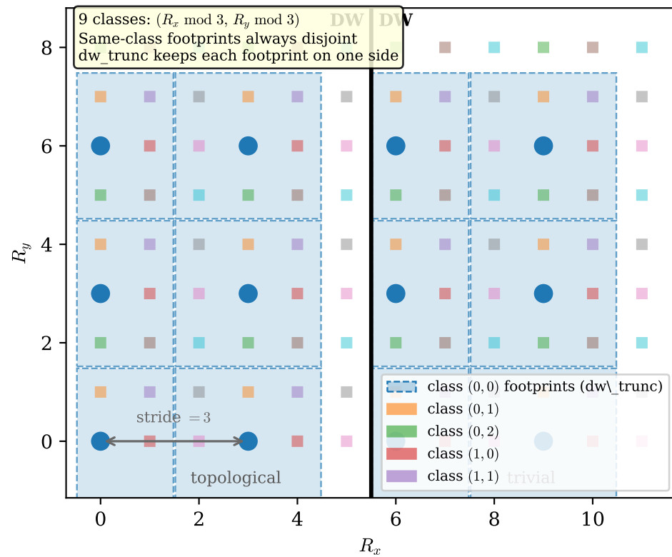
(a) Stride-3 color-class tiling ( n_{\text{shell}} = 1 , \text{stride} = 2n_{\text{shell}} + 1 = 3 )
