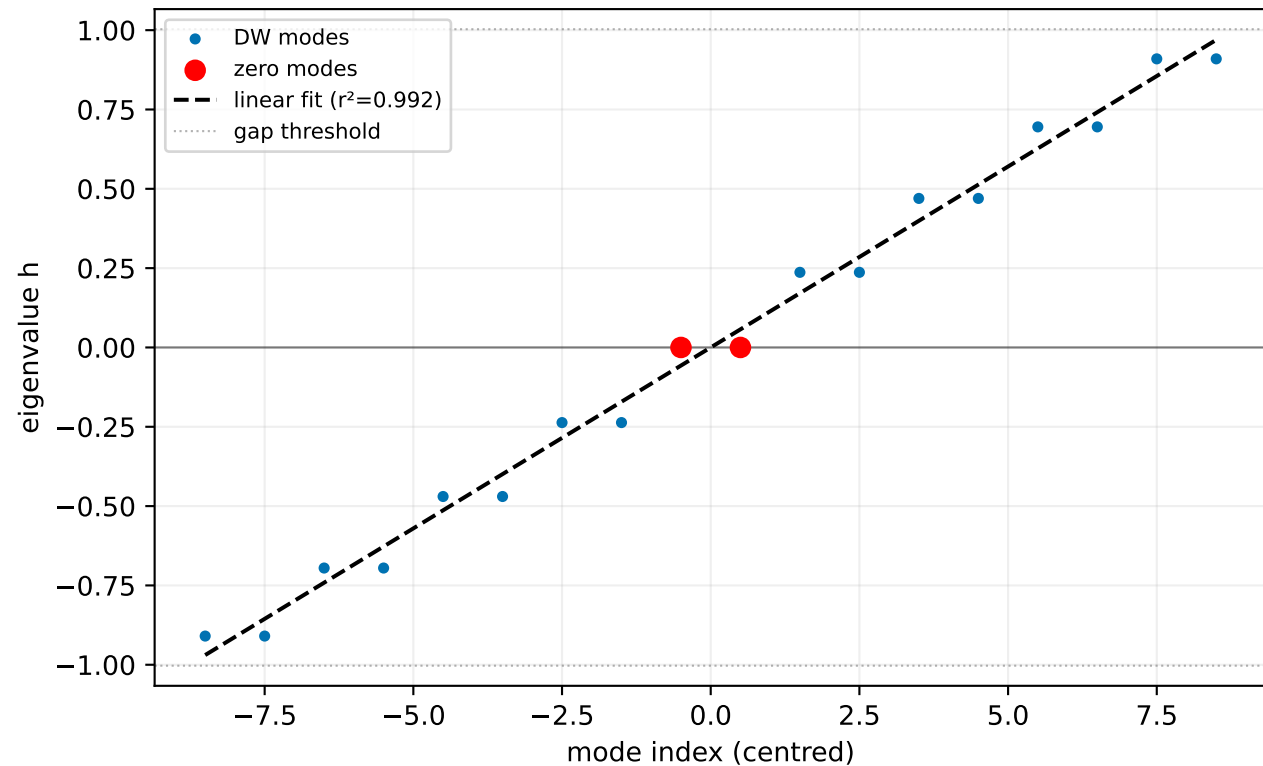
DW in-gap band (18 modes, 2 zero, 16 dispersive)
