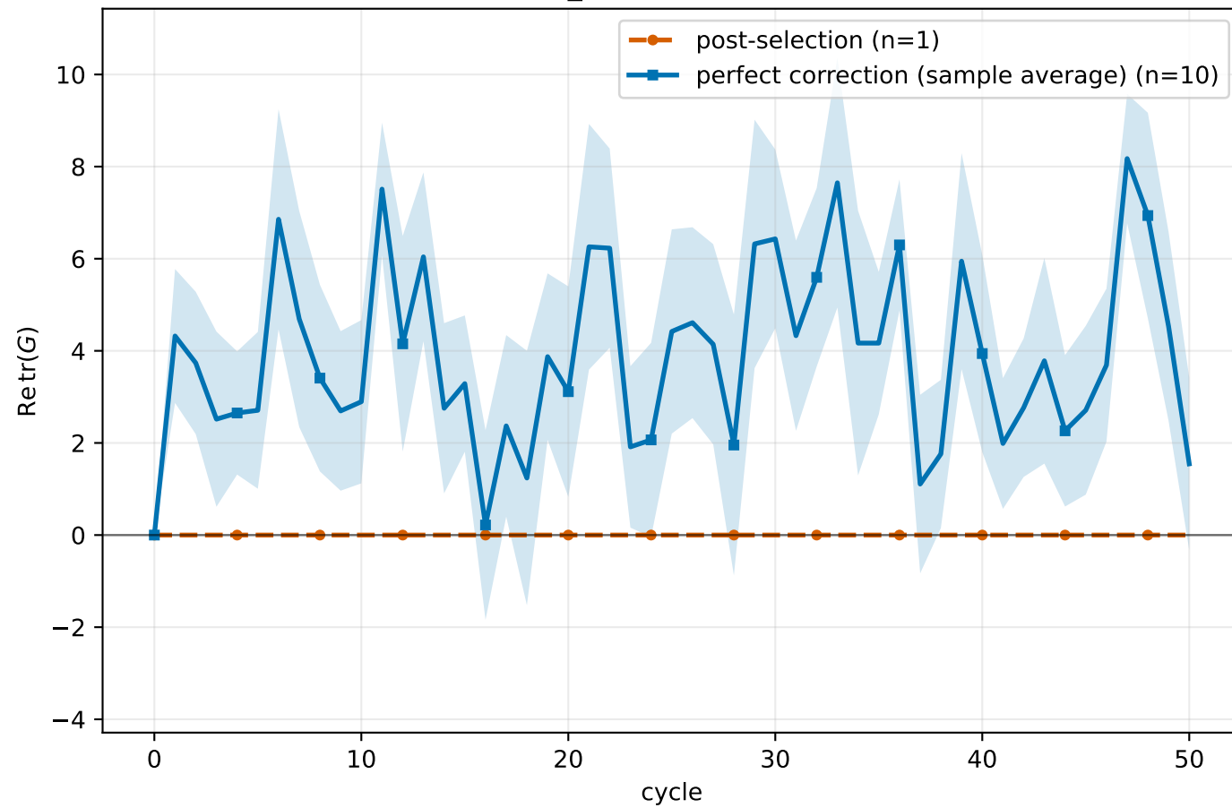
N20x40_C50_dwtrunc1: Re tr(G) vs cycle by init mode
