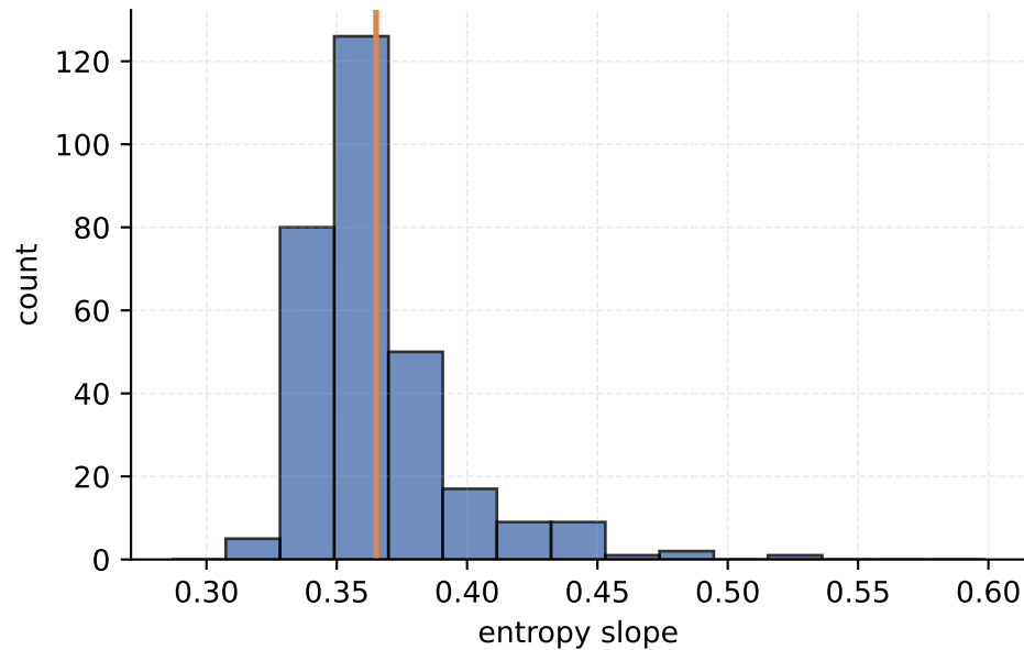
N20x20 perfect_correction late ensemble (cycles 21-50) mean=0.365086, n=300
