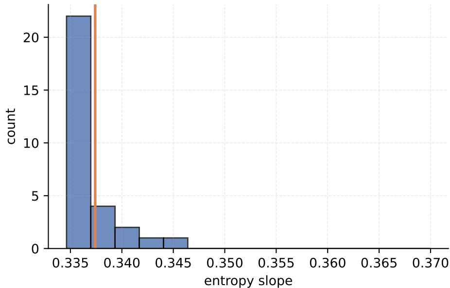
N20x20 postselect late ensemble (cycles 21-50) mean=0.337407, n=30
