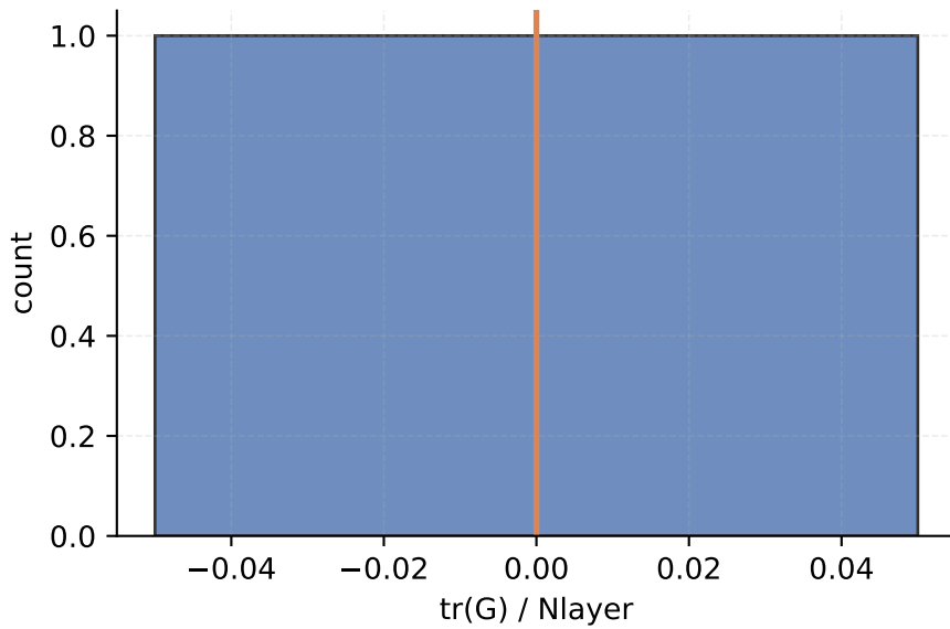
N20x20 postselect cycle 40 mean=-4.9738e-16, n=1
