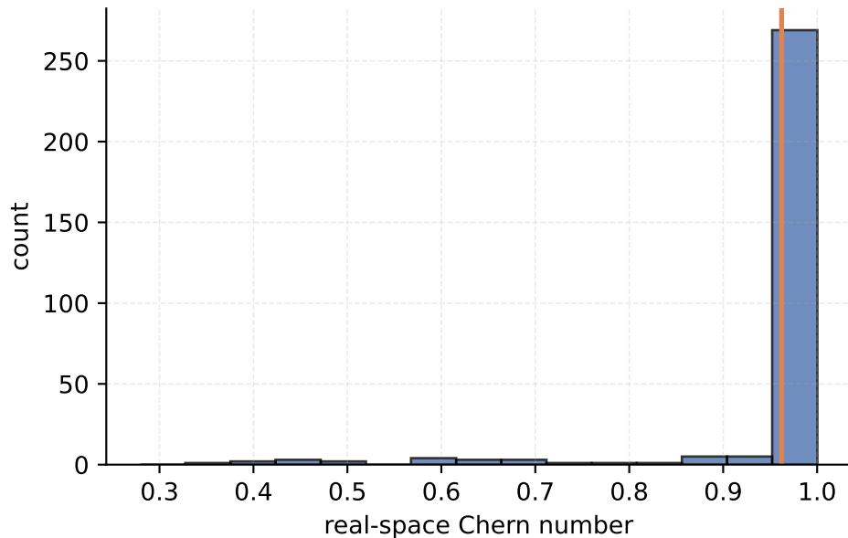
N20x20 perfect_correction late ensemble (cycles 21-50) mean=0.962225, n=300
