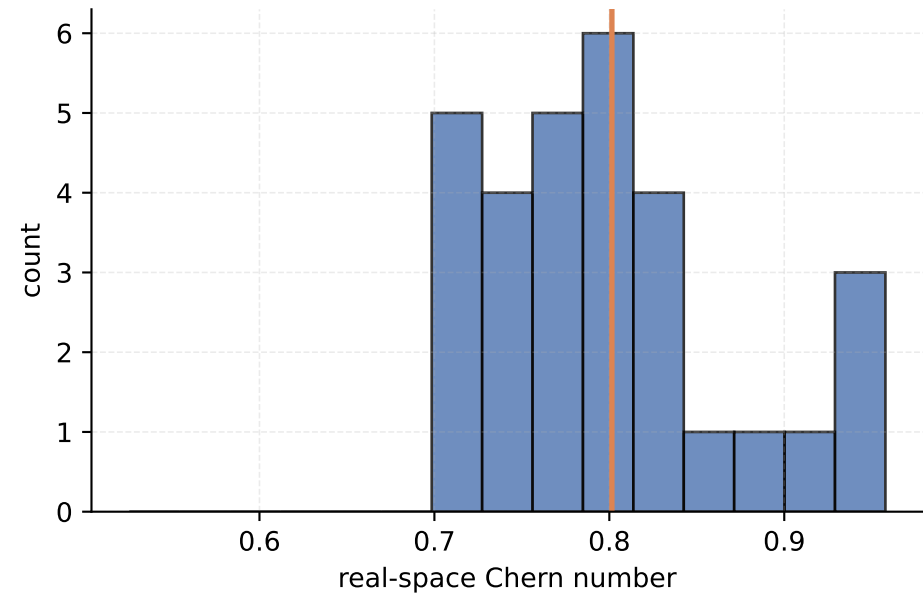
N20x40 postselect late ensemble (cycles 21-50) mean=0.801473, n=30
