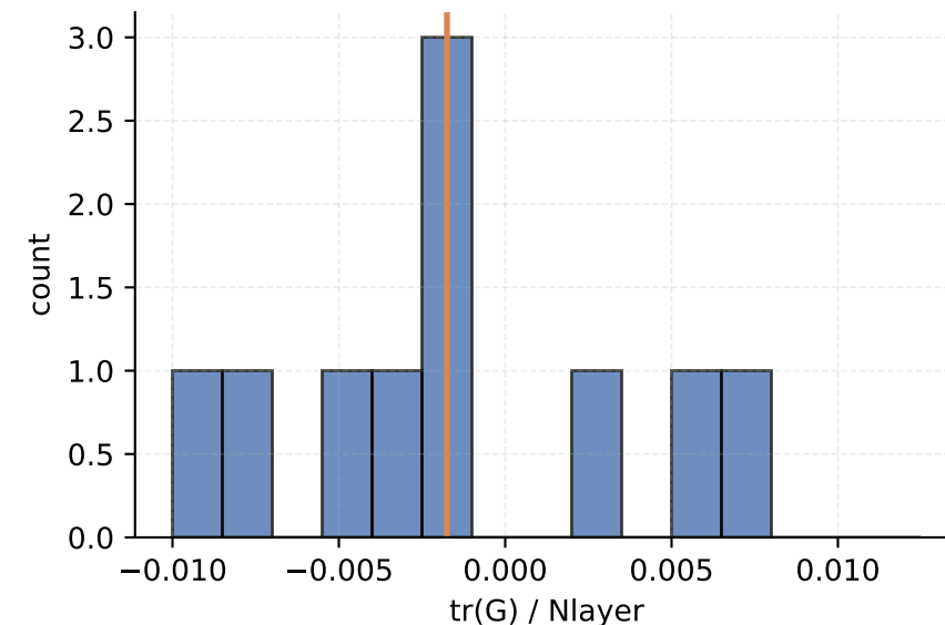
N20x20 perfect_correction cycle 30 mean=-0.00175, n=10
