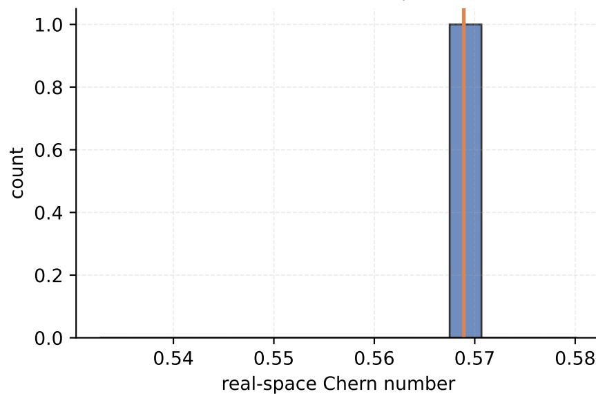
N20x20 postselect cycle 50 mean=0.568911, n=1
