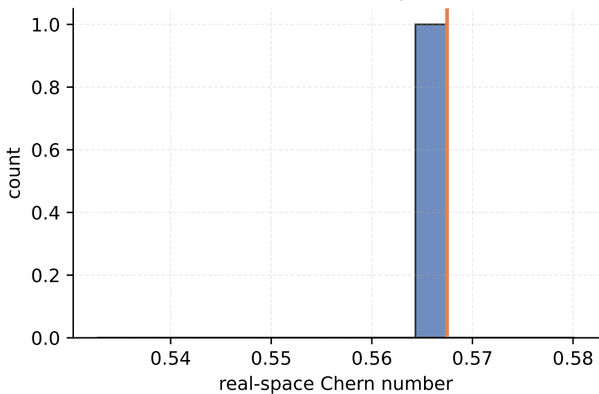
N20x20 postselect cycle 40 mean=0.567473, n=1
