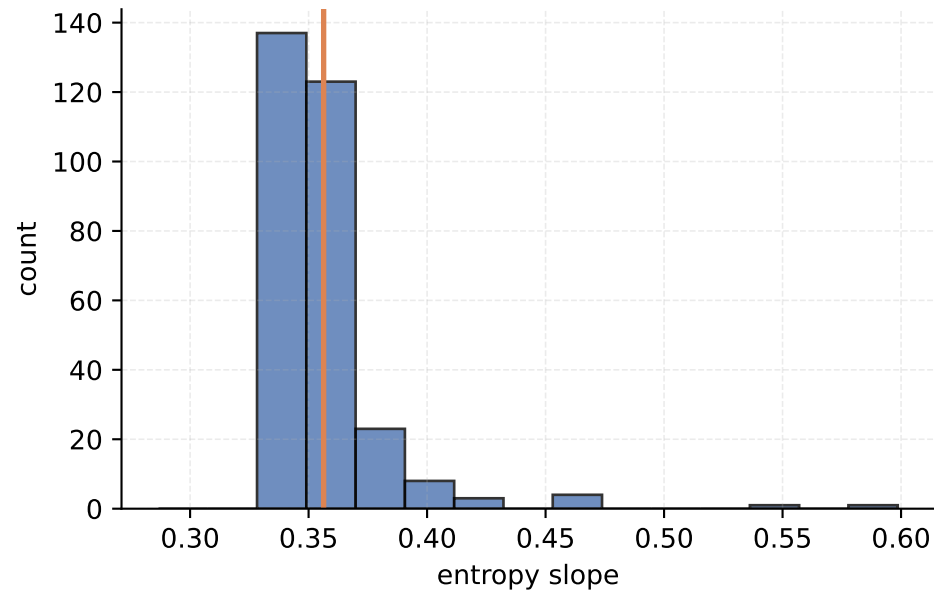
N20x30 perfect_correction late ensemble (cycles 21-50) mean=0.356355, n=300
