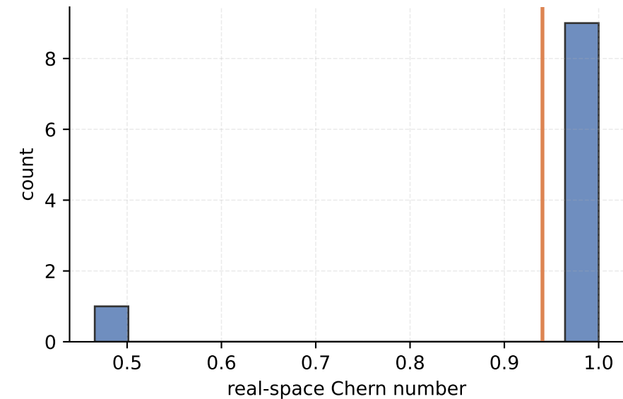
N20x20 perfect_correction cycle 30 mean=0.94041, n=10
