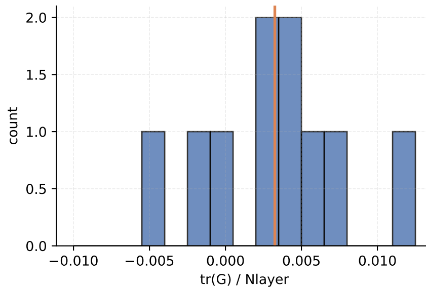
N20x20 perfect_correction cycle 50 mean=0.00325, n=10
