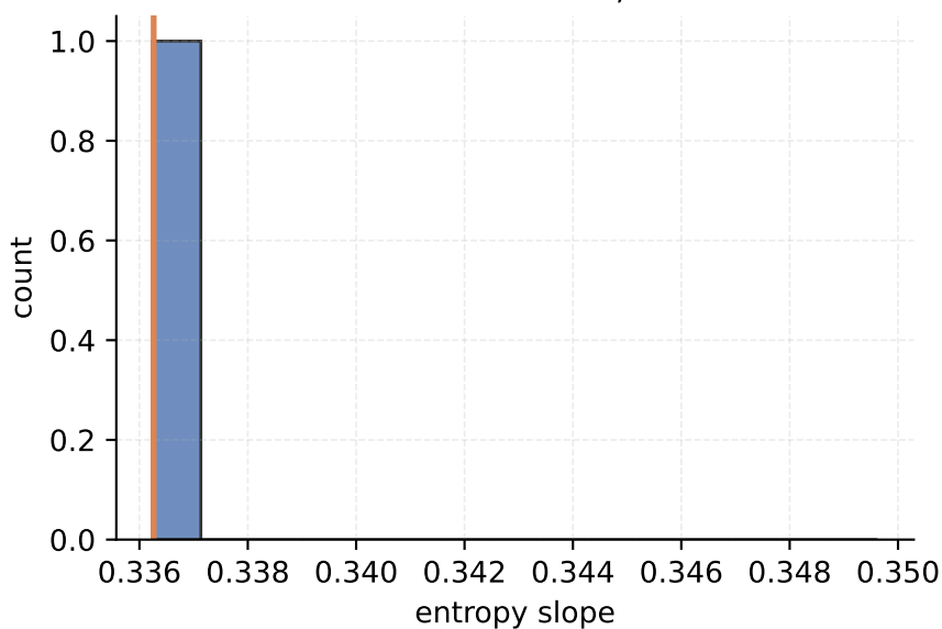
N20x20 postselect cycle 40 mean=0.336263, n=1
