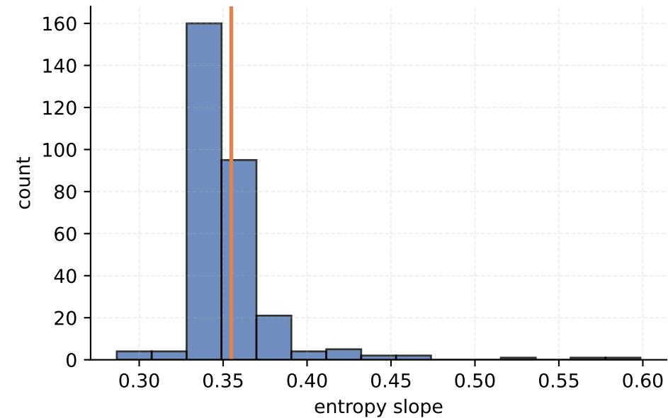
N20x40 perfect_correction late ensemble (cycles 21-50) mean=0.354868, n=300
