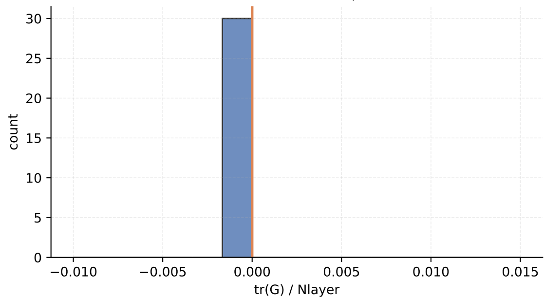
N20x30 postselect late normalized trace histogram (cycles 21-50) mean=-2.35269e-16, n=30
