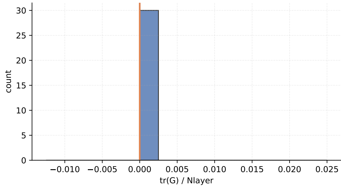
N20x20 postselect late normalized trace histogram (cycles 21-50) mean=-5.54223e-16, n=30
