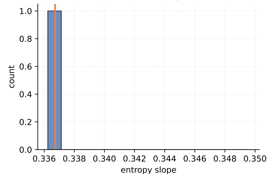
N20x20 postselect cycle 30 mean=0.336722, n=1
