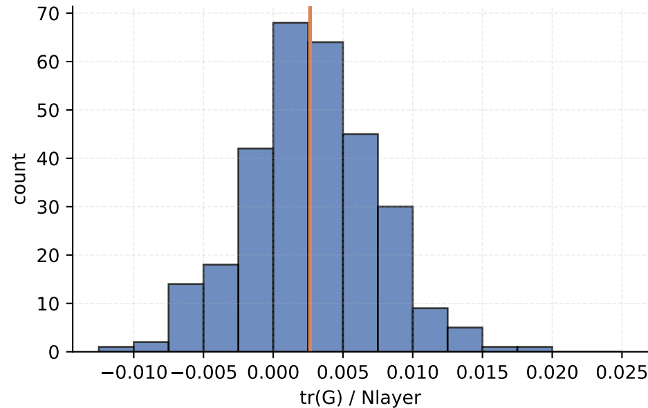
N20x40 perfect_correction late ensemble (cycles 21-50) mean=0.00264167, n=300
