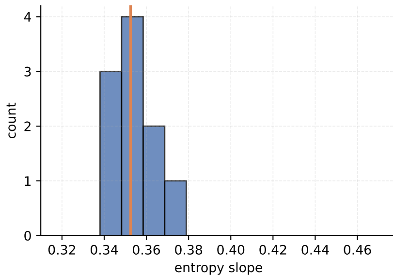
N20x20 perfect_correction cycle 40 mean=0.352543, n=10
