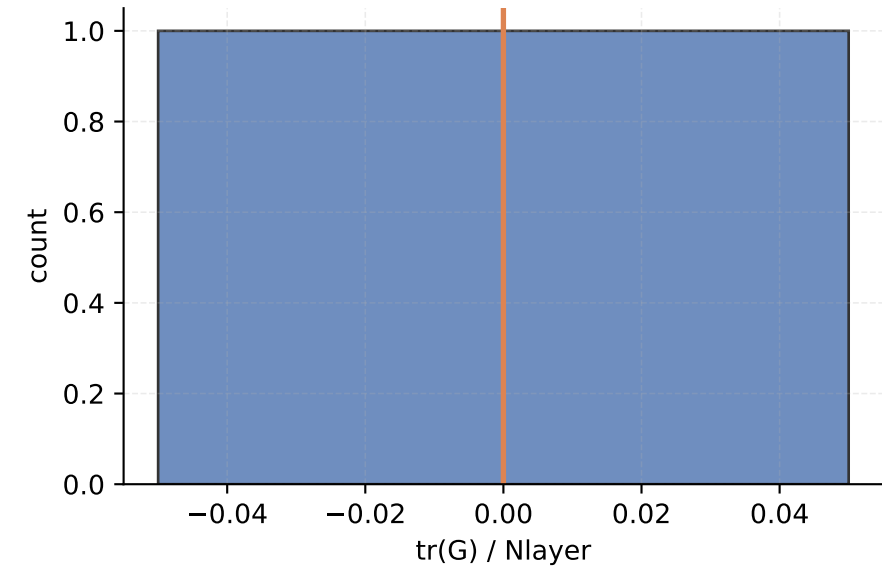
N20x20 postselect cycle 30 mean=-4.9738e-16, n=1
