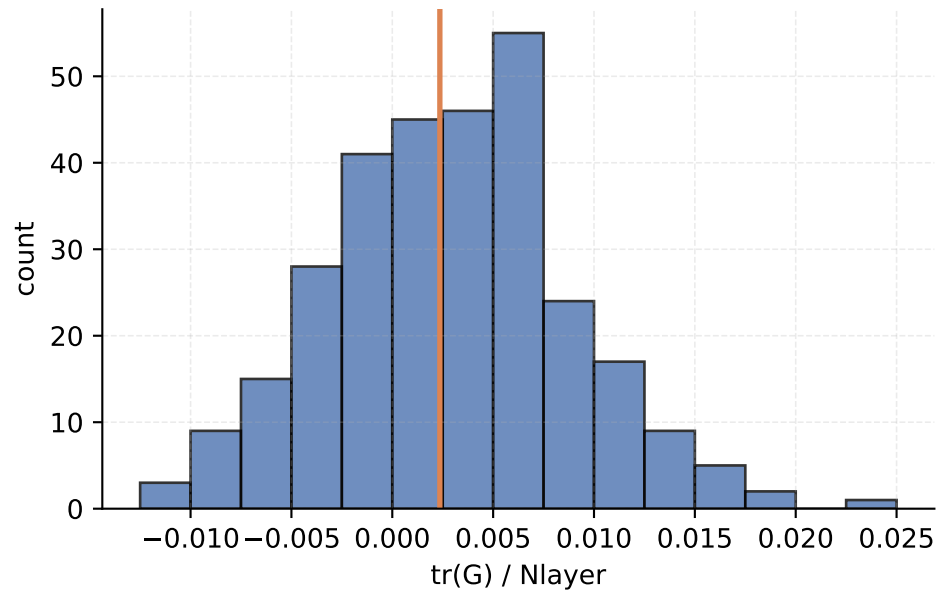
N20x20 perfect_correction late ensemble (cycles 21-50) mean=0.00235833, n=300
