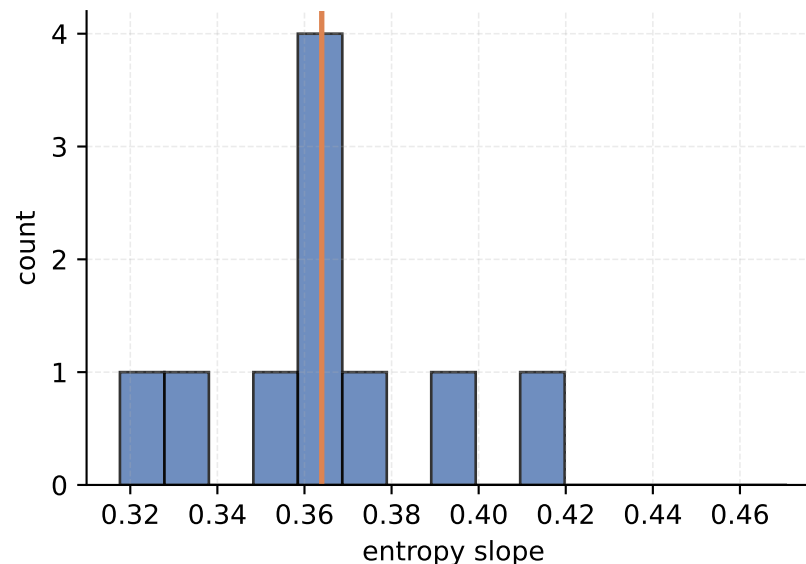
N20x20 perfect_correction cycle 50 mean=0.365142, n=10
