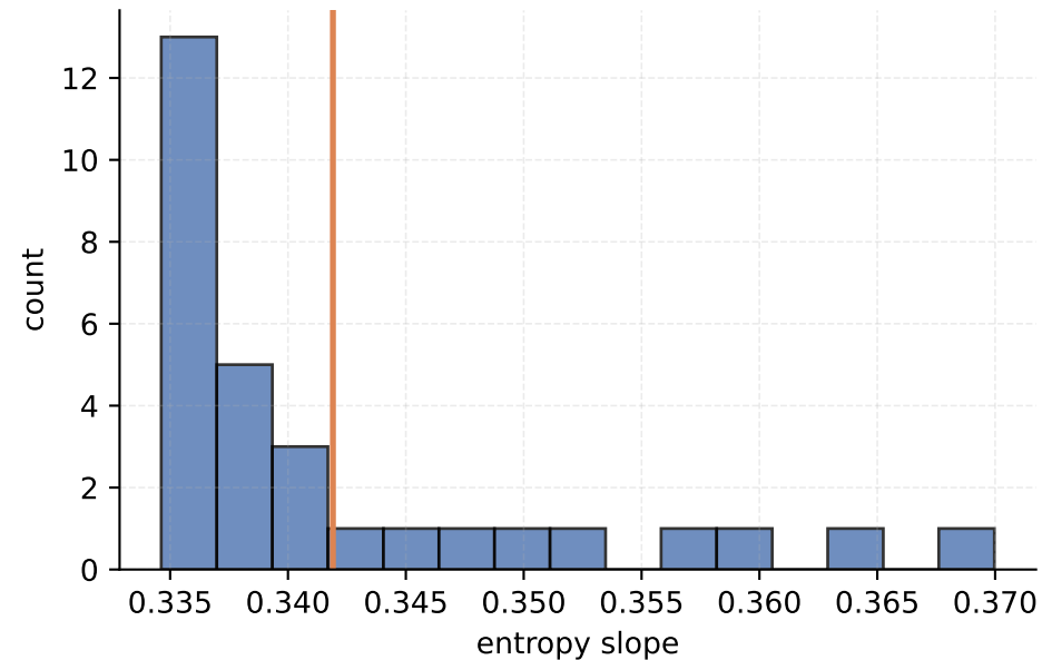
N20x40 postselect late ensemble (cycles 21-50) mean=0.341907, n=30
