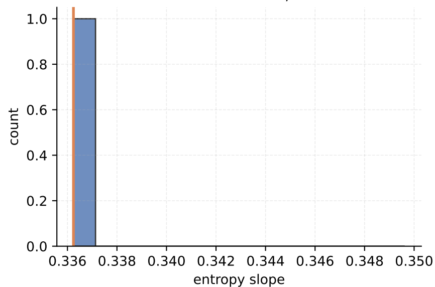
N20x20 postselect cycle 50 mean=0.336242, n=1
