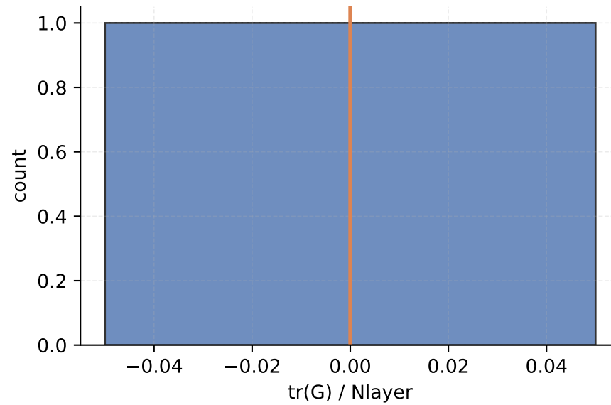
N20x20 postselect cycle 50 mean=-5.68434e-16, n=1
