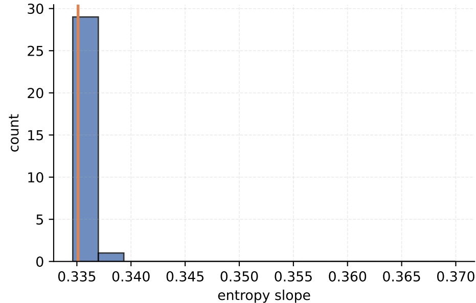
N20x30 postselect late ensemble (cycles 21-50) mean=0.335111, n=30
