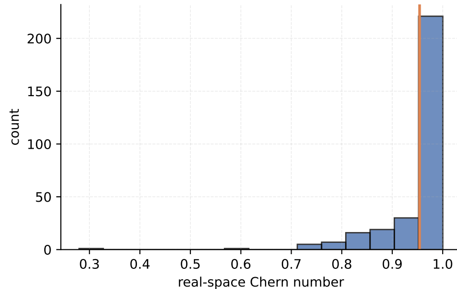
N20x40 perfect_correction late ensemble (cycles 21-50) mean=0.954185, n=300
