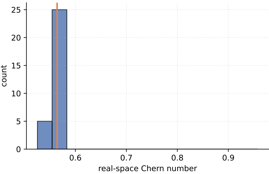
N20x20 postselect late ensemble (cycles 21-50) mean=0.564153, n=30
