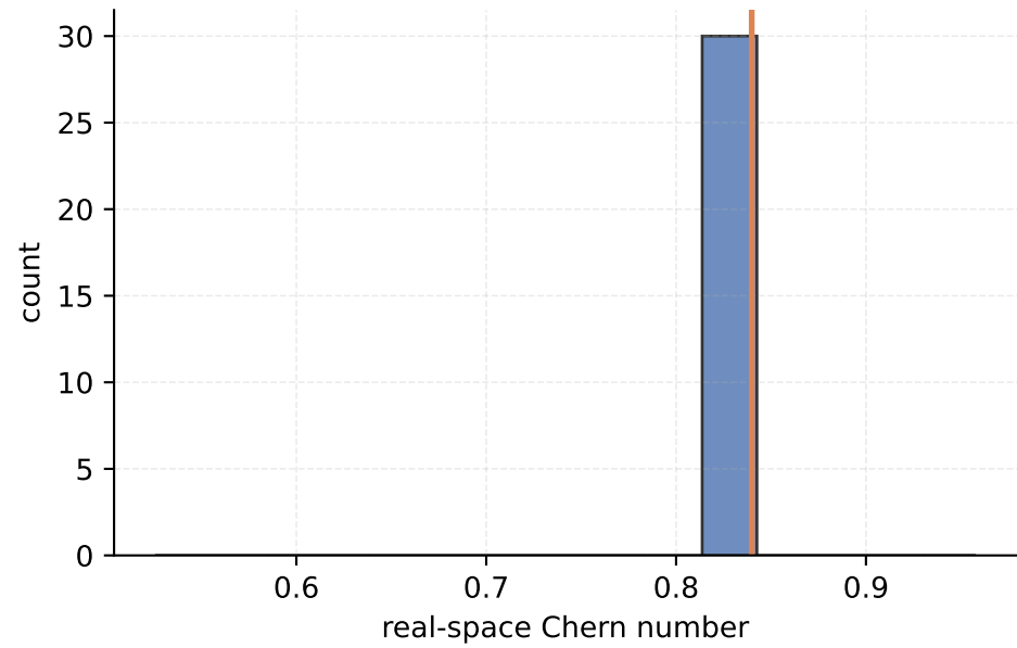
N20x30 postselect late ensemble (cycles 21-50) mean=0.839836, n=30
