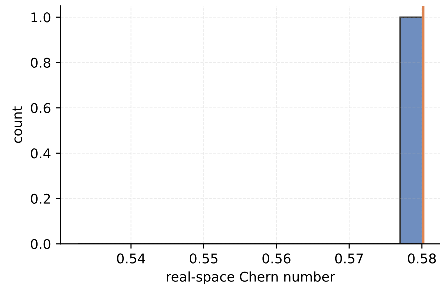
N20x20 postselect cycle 30 mean=0.580165, n=1
