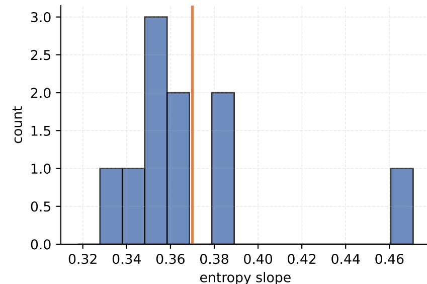
N20x20 perfect_correction cycle 30 mean=0.370015, n=10
