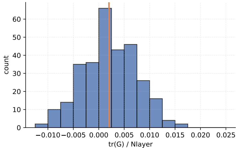
N20x30 perfect_correction late ensemble (cycles 21-50) mean=0.00200556, n=300
