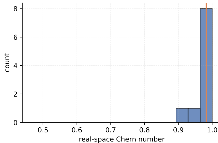
N20x20 perfect_correction cycle 50 mean=0.982783, n=10
