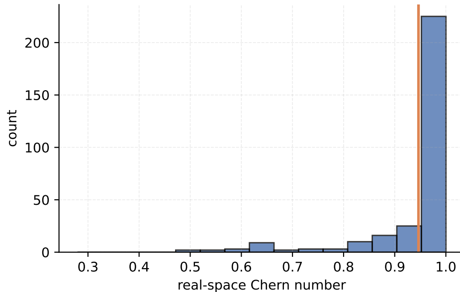
N20x30 perfect_correction late ensemble (cycles 21-50) mean=0.94649, n=300
