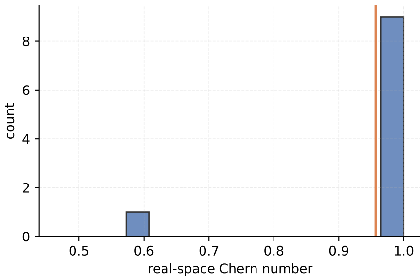
N20x20 perfect_correction cycle 40 mean=0.956954, n=10
