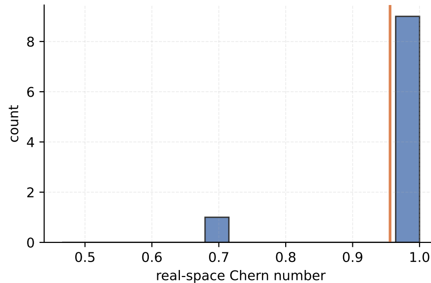
N20x20 perfect_correction cycle 50 mean=0.982783, n=10
