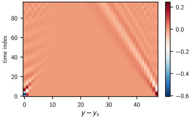
physical density response
