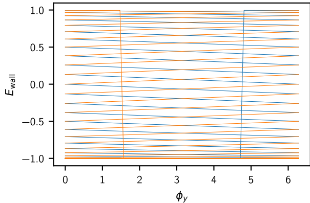
twist spectral flow
