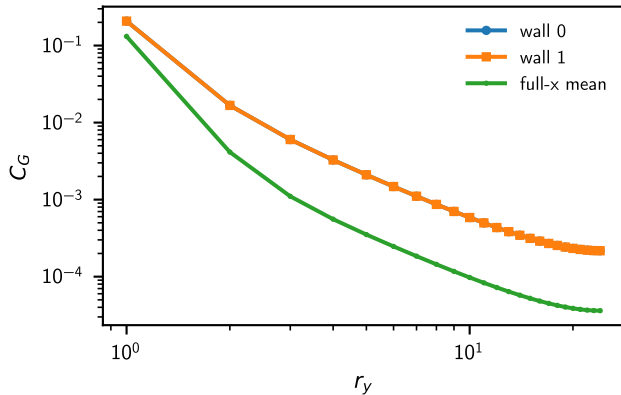
fixed-slice correlators
