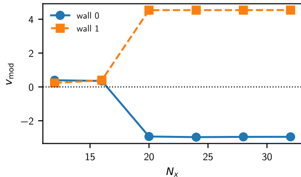
hard_exterior: endpoint handedness
