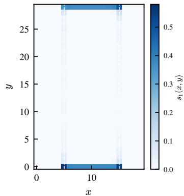
(a) fixed half-strip S_1 contour
