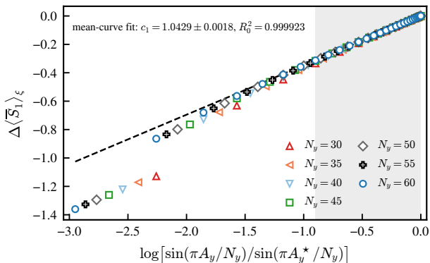
(a) ensemble-mean von Neumann entropy
