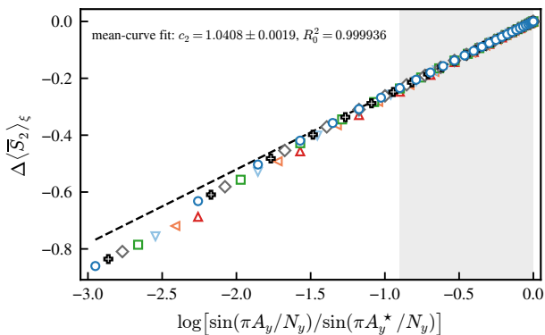
(b) ensemble-mean Rényi-2 entropy
