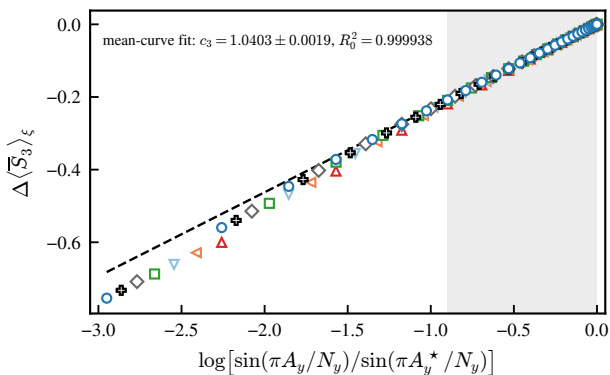
(c) ensemble-mean Rényi-3 entropy
