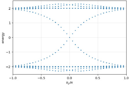
Flattened H vs k_y/\pi , \tau \in \sigma_x
