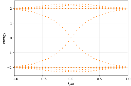
Flattened H vs k_y/\pi , \tau \in \sigma_y
