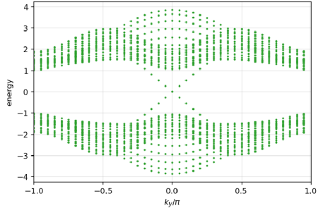
Flattened H vs k_y/\pi , \tau \in \sigma_z
