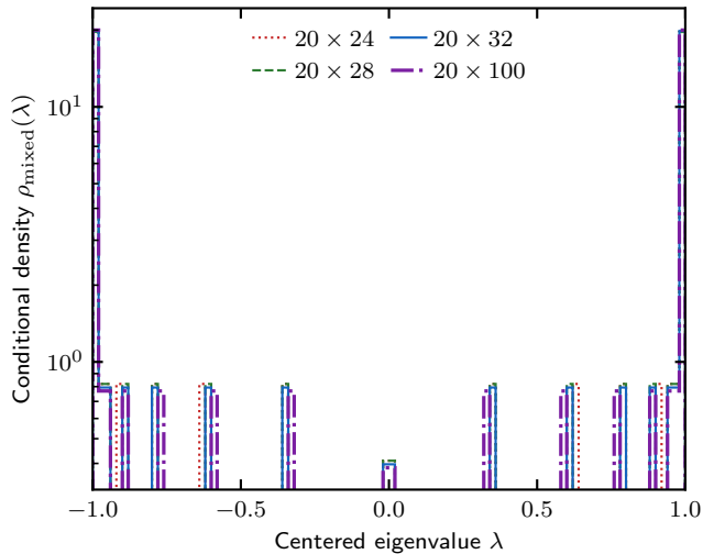
Equilibrium ground state: half-system
