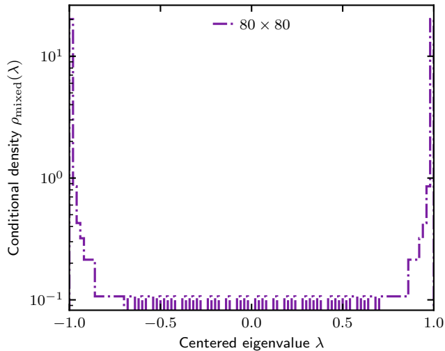
Square ground state: half-system
