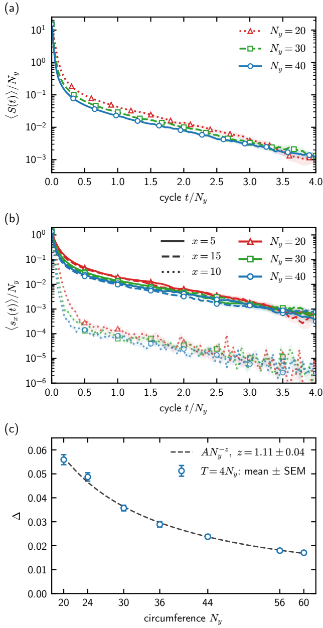
FIG. 1. Hard-wall purification and endpoint Lyapunov gap. Panels (a,b): 100 independent trajectories per size, N_y = 20, 30, 40 , from bundle 07. Panel (c): bundle-13 endpoints at T = 4N_y , with sample SEM and the weighted power-law fit \Delta \propto N_y^{-1.11 \pm 0.04} . See the accompanying README for the full estimator and sampling definitions.
