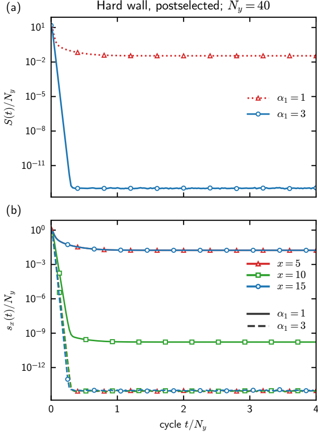
FIG. 1. Hard-wall postselected purification at N_x = 20 , N_y = 40 , \alpha_2 = 30 , n_{\text{shell}} = 1 , and T = 160 cycles. Each \alpha_1 = 1, 3 run is a single fully postselected trajectory from a maximally mixed active slab, with raster- y measurements and no feedback. (a) Total entropy S(t)/N_y . (b) Column entropy s_x(t)/N_y , summed over y and the two orbitals, at x = 5, 10, 15 . Colors and markers identify columns; solid and dashed curves identify \alpha_1 = 1, 3 , respectively. All 161 cycles are shown with logarithmic entropy and linear rescaled time. No averaging, fits, or uncertainty bars are applied. The \alpha_1 = 3 near-zero tails are roundoff-limited.
