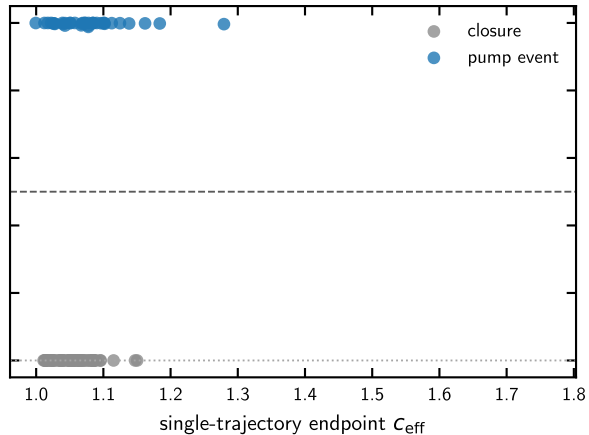
(b) Hard wall, r = 0.26
