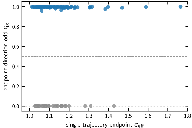
(a) Soft wall, r = 0.08
