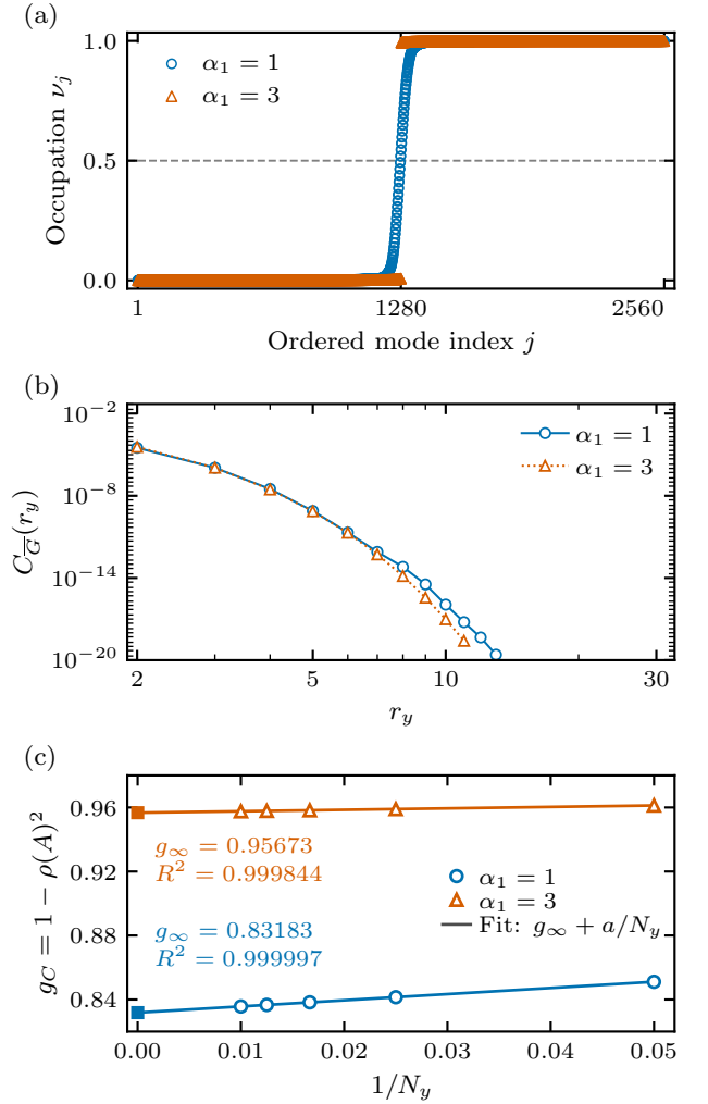
FIG. 11. Trajectory-averaged dynamics and channel gap. (a) Ordered occupation spectrum of \bar{G} and (b) its squared correlator C_{\bar{G}}(r_y) for N_x = 20 , N_y = 64 , after 128 cycles from maximal mixing. Open circles and triangles denote \alpha_1 = 1, 3 . Panel (b) uses logarithmic axes, r_y \geq 2 , and omits correlations below 10^{-20} . (c) Fits of g_C = 1 - \rho(A)^2 to g_{\infty} + a/N_y at fixed N_x = 20 , using N_y = 20, 40, 60, 80, 100 ; squares mark extrapolated intercepts. These deterministic calculations use the fixed repeated raster schedule. There are no sampled trajectories or statistical error bars.
