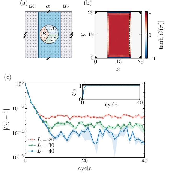
FIG. 2. Bulk topology in the domain-wall geometry.
