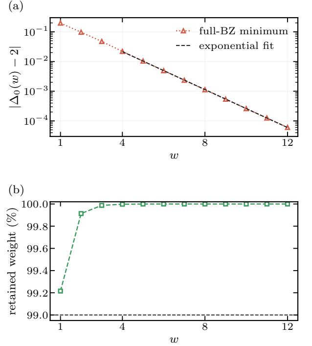
FIG. A1. Finite-range truncation at \alpha = 1 . (a) Deviation of the truncated-parent half-filling gap from its untruncated value, with the existing fit |\Delta_0(w) - 2| \propto e^{-w/\xi} for w \geq 4 on a logarithmic vertical axis. Here \xi \simeq 1.36 is the convergence length measured in truncation shells. (b) Fraction of the squared OW norm retained inside the window. These are deterministic parent-band calculations.
