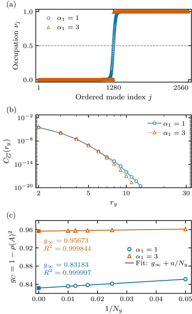
FIG. 10. Trajectory-averaged dynamics and channel gap. (a) Ordered occupation spectrum of \bar{G} and (b) its squared correlator C_{\bar{G}}(r_y) for N_x = 20 , N_y = 64 , after 128 cycles from maximal mixing. Open circles and triangles denote \alpha_1 = 1, 3 . Panel (b) uses logarithmic axes, r_y \geq 2 , and omits correlations below 10^{-20} . (c) Fits of g_C = 1 - \rho(A)^2 to g_\infty + a/N_y at fixed N_x = 20 , using N_y = 20, 40, 60, 80, 100 ; squares mark extrapolated intercepts. These deterministic calculations use the fixed repeated raster schedule. There are no sampled trajectories or statistical error bars.
