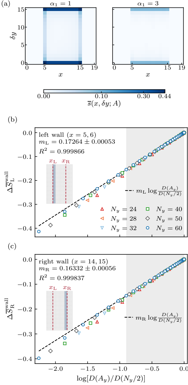
FIG. 8. Spatial entanglement and entropy carried by each wall. Each ensemble uses S = 100 independent random-pure half-filled trajectories, N_x = 20 , with a Born-prepared pure exterior. (a) Mean half-strip contours at N_y = 32 , cycle 64: the \alpha_1 = 1 endpoint ensemble of (b,c) and an independent \alpha_1 = 3 control, on a shared square-root scale; \delta y is relative to the strip origin. (b,c) Contour weight in columns x = 5, 6 and x = 14, 15 at \alpha_1 = 1 , for N_y = 24, 28, 32, 40, 50, 60 after 2N_y slab-only cycles. Vertical \Delta subtracts each trajectory's half-strip value. Dashed joint fits use 8 \leq A_y \leq N_y/2 (shaded), with equal total weight per size. Bars and fit errors are trajectory SEMs. Insets mark the integrated columns; A_y = 1 is omitted only from display.
