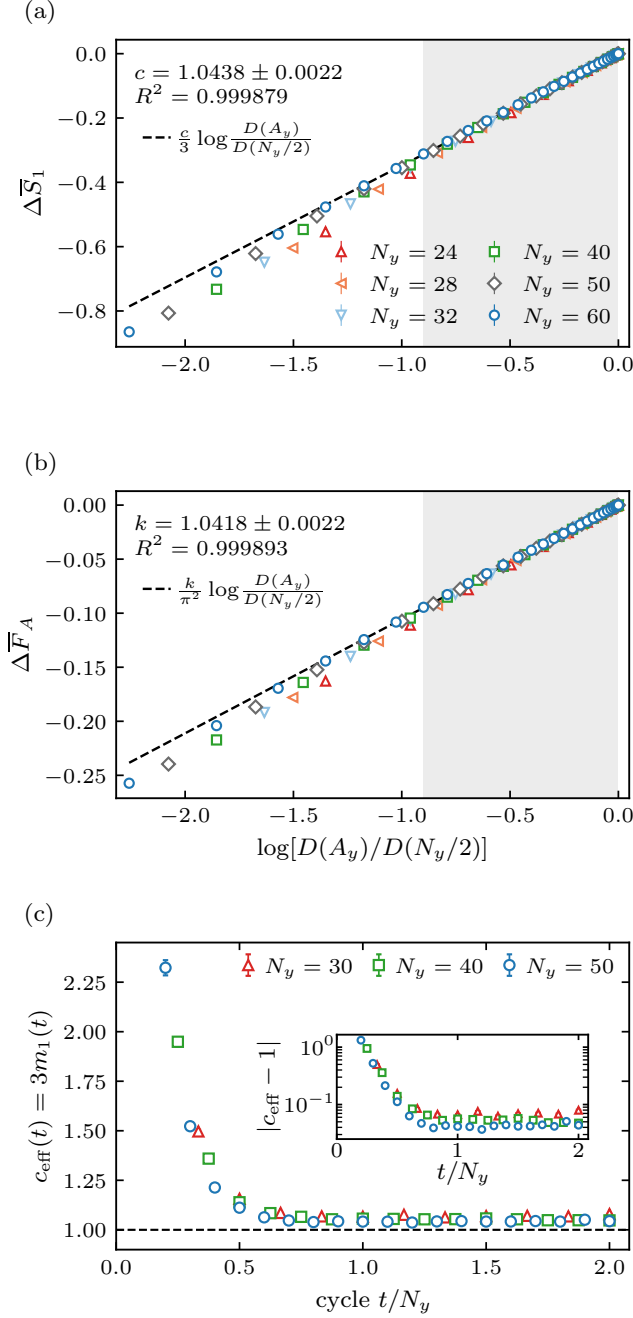
FIG. 6. Entanglement and charge fluctuations. Each ensemble has N_x = 20 and S = 100 independent random-pure half-filled trajectories. (a,b) Mean strip entropy and charge variance for N_y = 24, 28, 32, 40, 50, 60 at 2N_y cycles, with slab-only measurements and a Born-prepared pure exterior. Vertical \Delta subtracts each trajectory's value at A_y = N_y/2 . Dashed joint fits to Eq. (23) use 8 \leq A_y \leq N_y/2 (shaded), with equal total weight per size. Bars and fit errors are trajectory SEMs; A_y = 1 is omitted only from display. (c) Independent c_{\text{eff}} = 3m_1 histories for N_y = 30, 40, 50 through 2N_y cycles: free-intercept mean-entropy fits over 8 \leq A_y \leq N_y/2 , every fifth cycle from t = 10 . Bars are three slope regression standard errors; the inset shows |c_{\text{eff}} - 1| on a log axis.
