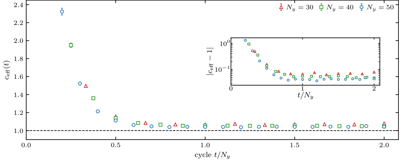
FIG. 8. Convergence of the entropy coefficient. Independent random-pure half-filled ensembles with N_x = 20 and S = 100 trajectories per N_y = 30, 40, 50 , through 2N_y cycles. At each displayed cycle (every fifth cycle from t = 10 ), a free-intercept fit of the trajectory-averaged strip entropy to Eq. (23) over 8 \leq A_y \leq N_y/2 gives c_{\text{eff}} = 3m_1 . Bars are three slope regression standard errors. The dashed line is c_{\text{eff}} = 1 ; the inset shows |c_{\text{eff}} - 1| on a logarithmic vertical axis. These pure-state histories are independent of the mixed-state purification and fresh endpoint ensembles.
