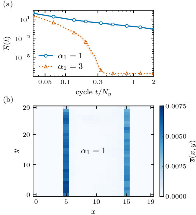
FIG. 3. Slow purification and residual entropy at the walls. Full-system maximally mixed initial states on a 20 \times 30 lattice, evolved for 60 full-measurement cycles with S = 100 independent trajectories per \alpha_1 . (a) Mean total entropy for \alpha_1 = 1, 3 on logarithmic axes; bands are one trajectory SEM. The trivial plateau is a numerical floor. (b) Full-system entropy contour \bar{S}(x, y; 60) for \alpha_1 = 1 [Eq. (13)], summed over both orbitals. Contours are evaluated within each trajectory and then averaged without normalization, translation averaging, or smoothing. The contour sum equals the mean total entropy at cycle 60; the remaining entropy is concentrated at the two interfaces.
