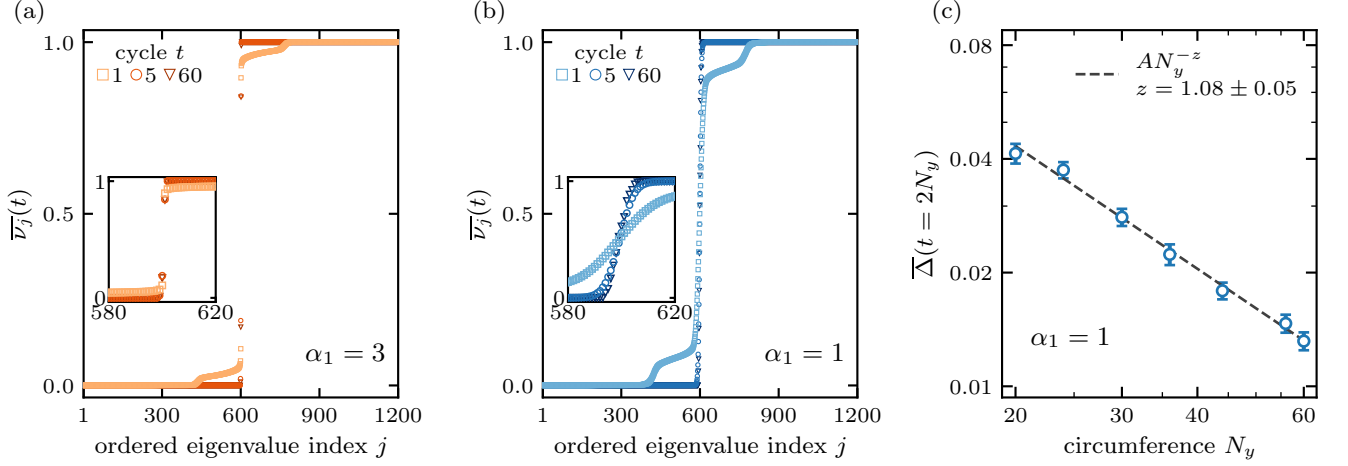
FIG. 4. Occupation spectra and finite-time Lyapunov gap. (a,b) Mean ascending occupation spectra at t = 1, 5, 60 for (a) \alpha_1 = 3 and (b) \alpha_1 = 1 , from the full-system maximally mixed 20 \times 30 ensembles of Fig. 3. Eigenvalues are sorted within each trajectory and cycle before averaging at fixed rank; all 1,200 ranks are displayed as open markers. Increasing cycle number runs from light to dark orange-red in (a) and blue in (b), with the same marker shapes in both panels. Insets show ranks 580 \leq j \leq 620 with identical limits. (c) Mean gap \overline{\Delta}(t = 2N_y) for \alpha_1 = 1 and N_y = 20, 24, 30, 36, 44, 56, 60 at fixed N_x = 20 , on logarithmic axes. The dashed line is an SEM-weighted fit over all seven sizes, with z = 1.08 \pm 0.05 ; error bars are one trajectory SEM. This separate size sweep uses slab-only measurements, an initially maximally mixed slab, and a pure decoupled exterior. Each panel uses S = 100 independent trajectories; the full-measurement spectra and slab-only gaps are distinct protocols and are not pooled.
