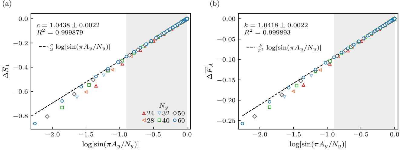
FIG. 6. Entanglement and charge fluctuations. Each ensemble has N_x = 20 and S = 100 independent random-pure half-filled trajectories. (a,b) Mean strip entropy and charge variance for N_y = 24, 28, 32, 40, 50, 60 at 2N_y cycles, with slab-only measurements and a Born-prepared pure exterior. Vertical \Delta subtracts each trajectory's value at A_y = N_y/2 . Dashed joint fits to Eq. (23) use 8 \leq A_y \leq N_y/2 (shaded), with equal total weight per size. Bars and fit errors are trajectory SEMs; A_y = 1 is omitted only from display.
