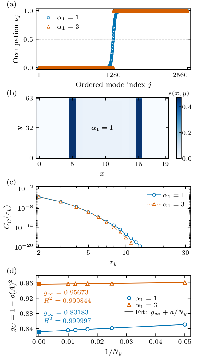
FIG. 11. Trajectory-averaged dynamics and channel gap. (a) Ordered occupation spectrum of \bar{G} for \alpha_1 = 1, 3 . (b) Full-system entropy contour s(x, y) of the outcome-averaged Gaussian state for \alpha_1 = 1 , evaluated from \bar{G} and summed over both orbitals, in nats per unit cell. The contour is unnormalized; dashed lines delimit the slab. It is not an average of trajectory entropy contours. (c) Squared correlator C_{\bar{G}}(r_y) for both controls. Panels (a-c) use N_x = 20 , N_y = 64 , after 128 cycles from maximal mixing. Open circles and triangles denote \alpha_1 = 1, 3 . Panel (c) uses logarithmic axes, r_y \geq 2 , and omits correlations below 10^{-20} . (d) Fits of g_C = 1 - \rho(A)^2 to g_\infty + a/N_y at fixed N_x = 20 , using N_y = 20, 40, 60, 80, 100 ; squares mark extrapolated intercepts. These deterministic calculations use the fixed repeated raster schedule. There are no sampled trajectories or statistical error bars.
