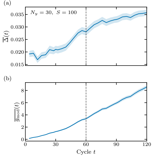
FIG. A2. Fixed-size purification diagnostic. (a) Mean finite-time rate \bar{\Delta}(t) and (b) mean raw modular gap \bar{g}_{\text{mod}}(t) for N_x = 20 , N_y = 30 , \alpha_1 = 1 , \alpha_2 = 30 , and w = 1 , through 120 cycles. The saved slab-only protocol starts with a maximally mixed slab and a Born-prepared pure exterior; S = 100 independent trajectories. The minimum is taken within each trajectory before averaging. Bands are one trajectory SEM; the vertical reference marks 2N_y . No time fit or extrapolation is shown.
