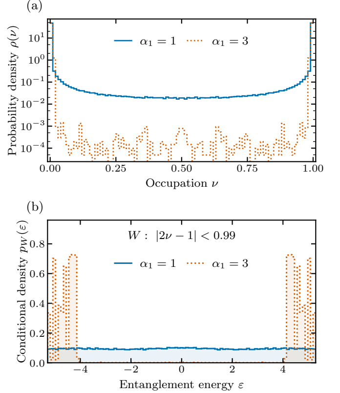
FIG. 7. Restricted occupation and energy spectra. Hard-wall states at N_x = 20 , N_y = 32 , cycle 64, from S = 100 independent random-pure half-filled trajectories for \alpha_1 = 1, 3 . (a) Unit-area occupation histograms on a logarithmic vertical axis. (b) Conditional unit-area energy densities for |2\nu - 1| < 0.99 , using 101 bins on [-\log 199, \log 199] . Both panels pool all 32 translated half-strips. The energy window contains 95,398 and 83,326 observations for \alpha_1 = 1, 3 .
