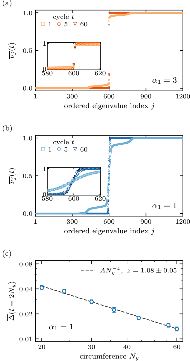
FIG. 4. Occupation spectra and finite-time Lyapunov gap. (a,b) Mean ascending occupation spectra at t = 1, 5, 60 for (a) \alpha_1 = 3 and (b) \alpha_1 = 1 , from the full-system maximally mixed 20 \times 30 ensembles of Fig. 3. Eigenvalues are sorted within each trajectory and cycle before averaging at fixed rank; all 1,200 ranks are displayed as open markers. Increasing cycle number runs from light to dark orange-red in (a) and blue in (b), with the same marker shapes in both panels. Insets show ranks 580 \leq j \leq 620 with identical limits. (c) Mean gap \overline{\Delta}(t = 2N_y) for \alpha_1 = 1 and N_y = 20, 24, 30, 36, 44, 56, 60 at fixed N_x = 20 , on logarithmic axes. The dashed line is an SEM-weighted fit over all seven sizes, with z = 1.08 \pm 0.05 ; error bars are one trajectory SEM. This separate size sweep uses slab-only measurements, an initially maximally mixed slab, and a pure decoupled exterior. Each panel uses S = 100 independent trajectories; the full-measurement spectra and slab-only gaps are distinct protocols and are not pooled.
