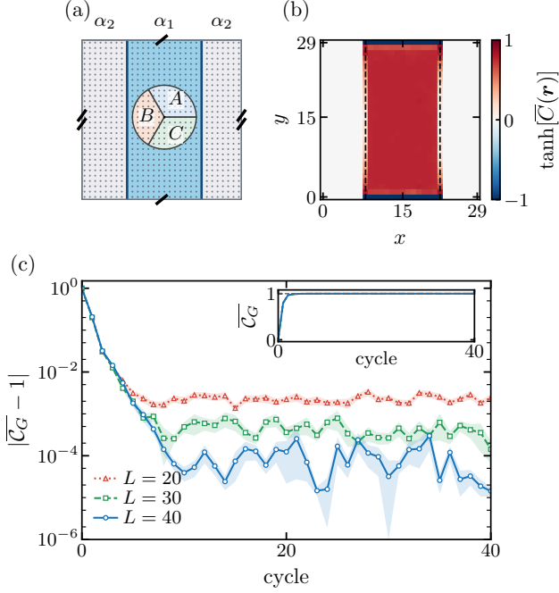
FIG. 2. Bulk topology in the domain-wall geometry. (a) A 30 \times 30 lattice with interfaces at x = 8, 22 and a three-sector disk of radius R = 6 . The drawn transverse center is representative; matching single and double slashes identify opposite periodic edges. (b) Local Chern marker [Eq. (11)] at L = 30 , cycle 40, displayed as \tanh[\bar{C}(\mathbf{r})] after averaging S = 100 independent trajectories. The bounded color scale compresses the periodic-coordinate seam contribution. (c) |\bar{G} - 1| for L = 20, 30, 40 on a logarithmic vertical axis, with the untransformed \bar{G} in the inset. Each cycle averages ten randomly chosen disk centers per trajectory, then S = 100 independent trajectories. Shading is one trajectory SEM. All ensembles start from random pure half-filled states and use \alpha_1 = 1 , \alpha_2 = 30 , and w = 1 .
