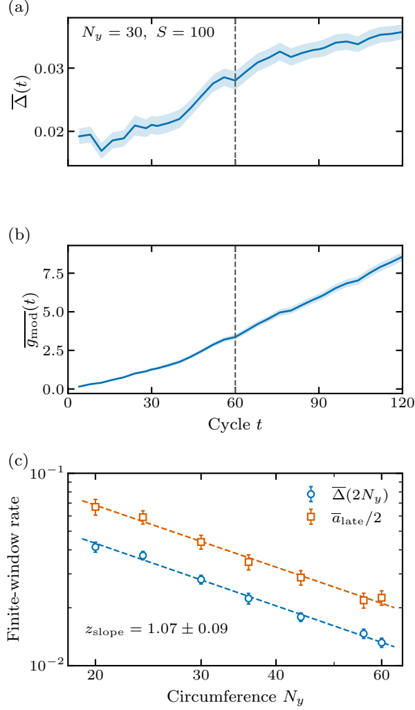
FIG. A2. Finite-time purification and raw-gap growth. (a) Mean rate \bar{\Delta}(t) and (b) mean raw modular gap \overline{g_{\text{mod}}}(t) for N_x = 20 , N_y = 30 , \alpha_1 = 1 , \alpha_2 = 30 , and w = 1 , through 120 cycles. The saved slab-only protocol starts with a maximally mixed slab and a Born-prepared pure exterior; S = 100 independent trajectories. The minimum is taken within each trajectory before averaging. Bands are one trajectory SEM; the vertical reference marks 2N_y . (c) Seven-size comparison of \bar{\Delta}(2N_y) with half the mean raw-gap secant slope over [3N_y, 4N_y] , defined in Eq. (C2). Bars are trajectory SEMs, with endpoint differences formed within each trajectory. Dashed lines are SEM-weighted power-law fits over all seven sizes; the displayed slope exponent has a formal regression error. The growth rate is a finite-window diagnostic, not an established asymptotic gap.
