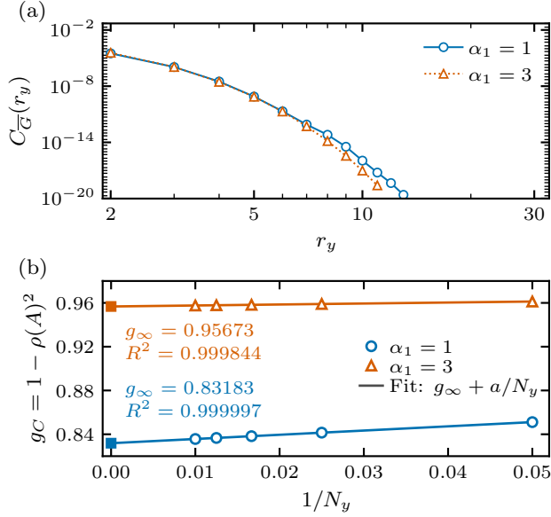
FIG. 12. Short-range correlations and relaxation of the averaged channel. (a) Squared correlator C_{\overline{G}}(r_y) for \alpha_1 = 1, 3 , with N_x = 20 , N_y = 64 , after 128 cycles from maximal mixing. Open circles and triangles denote \alpha_1 = 1, 3 . Logarithmic axes show r_y \geq 2 and omit correlations below 10^{-20} . (b) Fits of g_C = 1 - \rho(A)^2 to g_\infty + a/N_y at fixed N_x = 20 , using N_y = 20, 40, 60, 80, 100 ; squares mark extrapolated intercepts. These deterministic calculations use the fixed repeated raster schedule. There are no sampled trajectories or statistical error bars.
