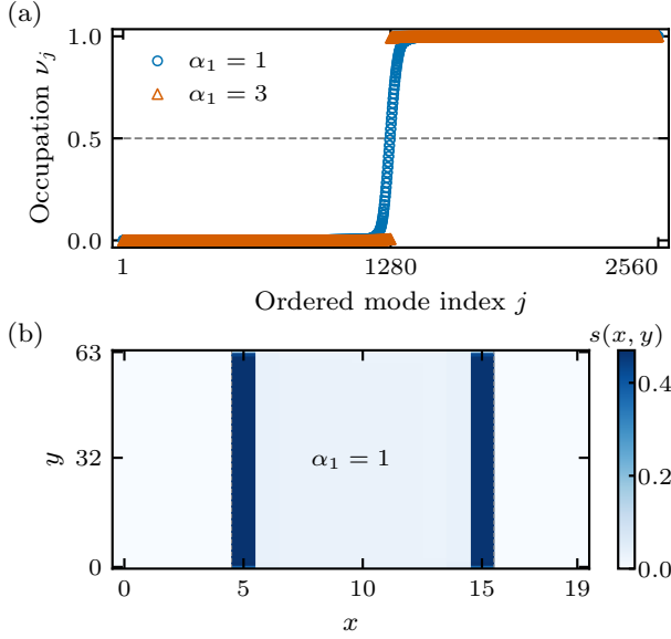
FIG. 11. Spectrum and entropy of the outcome-averaged state. (a) Ordered occupation spectrum of \bar{G} for \alpha_1 = 1, 3 . (b) Full-system entropy contour s(x, y) of the outcome-averaged Gaussian state for \alpha_1 = 1 , evaluated from \bar{G} and summed over both orbitals, in nats per unit cell. The contour is unnormalized; dashed lines delimit the slab. It is not an average of trajectory entropy contours. Both panels use N_x = 20 , N_y = 64 , after 128 cycles from maximal mixing. Open circles and triangles denote \alpha_1 = 1, 3 . These deterministic calculations use the fixed repeated raster schedule, with no sampled trajectories or statistical error bars.
