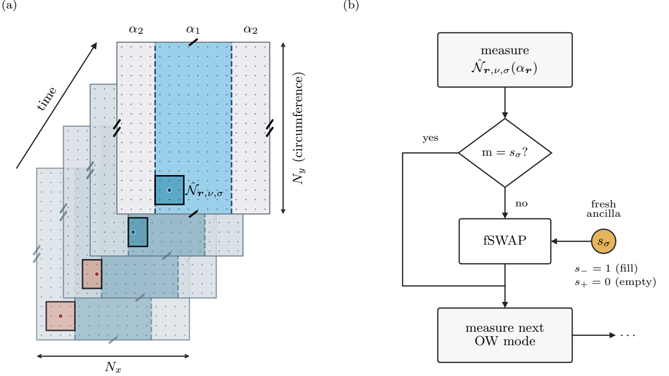
FIG. 1. Domain-wall geometry and adaptive circuit. (a) Four time slices illustrate OW updates in the periodic geometry, with \alpha_{\mathbf{r}} = \alpha_1 in the central slab and \alpha_2 fixed at 30 in the trivial exterior. Along the time arrow, the supports progress from the exterior bulk through either side of the left interface to the slab bulk. Matching marks identify opposite boundaries. Salmon and blue windows show exterior and slab OW supports; dots mark their centers. Bulk supports contain 3 \times 3 cells; interface supports are clipped and renormalized. (b) An occupation measurement returns the Born outcome m . If m = s_{\sigma} , correction is bypassed; otherwise an fSWAP with a fresh ancilla restores s_{-} = 1 or s_{+} = 0 . The branches rejoin and the procedure repeats for subsequent OW modes.
