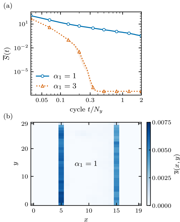
FIG. 3. Slow purification and residual entropy at the walls. Full-system maximally mixed initial states on a 20 \times 30 lattice, evolved for 60 full-measurement cycles with S = 100 independent trajectories per \alpha_1 . (a) Mean total entropy for \alpha_1 = 1, 3 on logarithmic axes; bands are one trajectory SEM. The trivial plateau is a numerical floor. (b) Full-system entropy contour \bar{s}(x, y; 60) for \alpha_1 = 1 [Eq. (13)], summed over both orbitals. Contours are evaluated within each trajectory and then averaged without normalization, translation averaging, or smoothing. The contour sum equals the mean total entropy at cycle 60; the remaining entropy is concentrated at the two interfaces.
