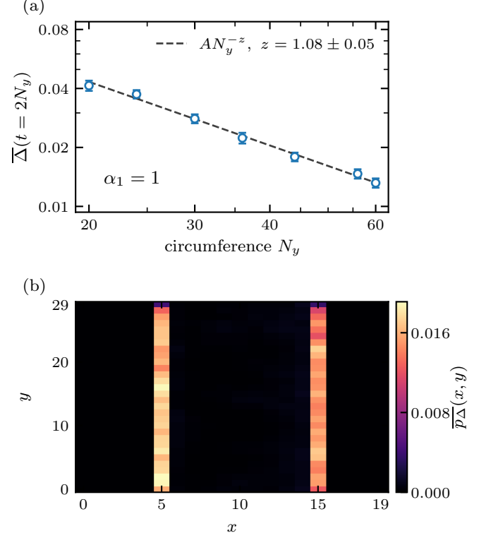
FIG. 4. Finite-time Lyapunov gap and boundary localization. (a) Mean gap \overline{\Delta}(t = 2N_y) for \alpha_1 = 1 and N_y = 20, 24, 30, 36, 44, 56, 60 at fixed N_x = 20 . The dashed line is an SEM-weighted fit over all seven sizes, with z = 1.08 \pm 0.05 ; error bars are one trajectory SEM. The slab is initially maximally mixed and the decoupled exterior is pure. (b) Mean spatial density of the unique slowest mode for \alpha_1 = 1 , N_y = 30 , and t = 60 , starting with the full system maximally mixed. Each panel uses S = 100 independent trajectories; gaps and normalized mode densities are evaluated per trajectory before averaging.
