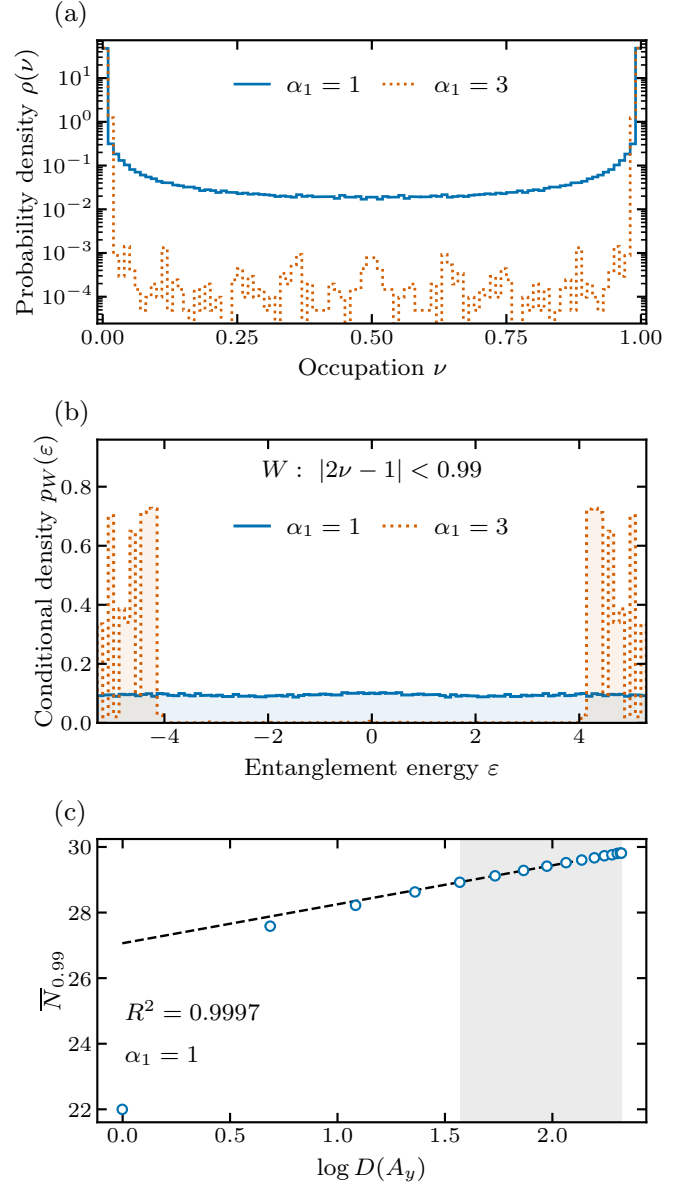
FIG. 7. Restricted spectra and mode count. Hard-wall states at N_x = 20 , N_y = 32 , cycle 64, from S = 100 independent random-pure half-filled trajectories per \alpha_1 = 1, 3 . (a) Full occupation histogram on 0 \leq \nu \leq 1 , normalized to unit area. (b) Conditional unit-area energy density for |2\nu - 1| < 0.99 , in 101 equal bins on [-\log 199, \log 199] . The central depletion at \alpha_1 = 3 contrasts with the finite near-zero density at \alpha_1 = 1 . Both histograms pool all 32 translated half-strips per trajectory. The retained totals are 95,398 and 83,326 for \alpha_1 = 1, 3 . (c) Raw mean window count for \alpha_1 = 1 , averaging origins within each trajectory. Bars are one trajectory SEM; the dashed fit uses 5 \leq A_y \leq 16 (shaded), while all widths are displayed. Translated cuts are correlated observations, not additional trajectories.
