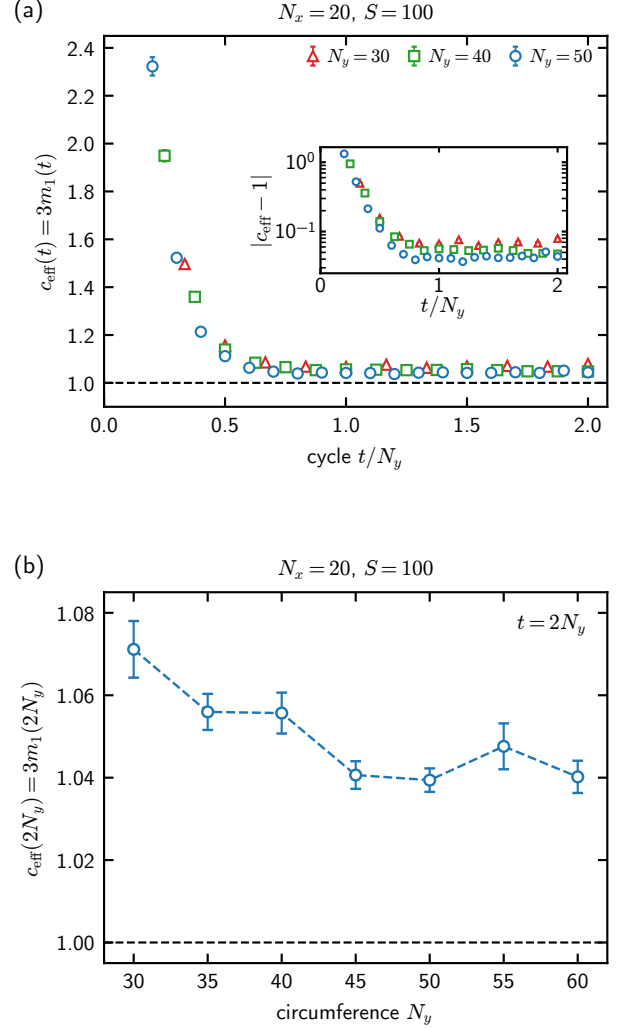
FIG. 8. Convergence of the entropy coefficient. c_{\text{eff}} = 3m_1 is extracted from a free-intercept fit of \bar{S} versus \log chord length over 8 \leq A_y \leq N_y/2 . (a) Cycle dependence for N_y = 30, 40, 50 ; the inset resolves |c_{\text{eff}} - 1| . Bars are regression standard errors of the mean-curve slope. (b) Endpoint values after 2N_y cycles for N_y = 30, 35, \dots, 60 ; bars are trajectory SEMs propagated with the covariance between widths. Both panels use S = 100 independent random-pure trajectories per size and origin averaging, but come from separate ensembles. The horizontal reference is one; connecting lines in (b) are guides.
