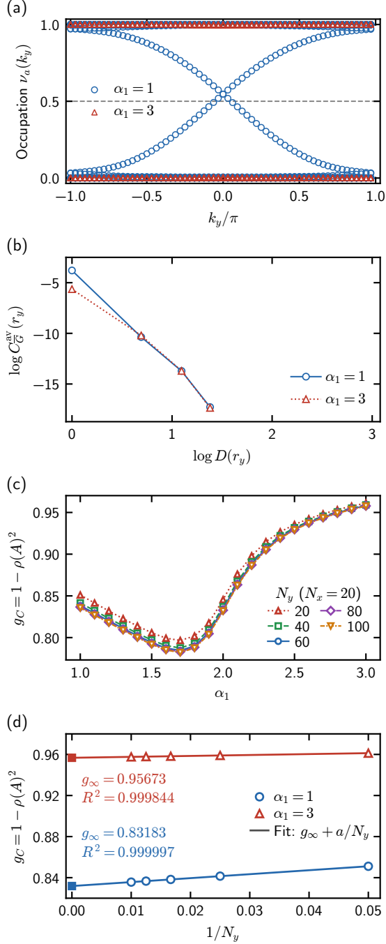
FIG. 11. Trajectory-averaged dynamics and channel gap. (a) Occupations of the translation-averaged two-point matrix and (b) its squared correlation at N_y = 64 , after 128 cycles from maximal mixing, for \alpha_1 = 1, 3 . Correlations below 10^{-8} are not displayed. (c) Exact multiplier gap g_C = 1 - \rho(A)^2 versus \alpha_1 at fixed N_x = 20 and N_y = 20, 40, 60, 80, 100 . (d) Fits g_\infty + a/N_y at \alpha_1 = 1, 3 , using all five sizes; squares at 1/N_y = 0 mark extrapolated intercepts. Outcomes are averaged analytically in the fixed repeated raster schedule, so there is no sampled-trajectory count or SEM. The gap is dimensionless.
