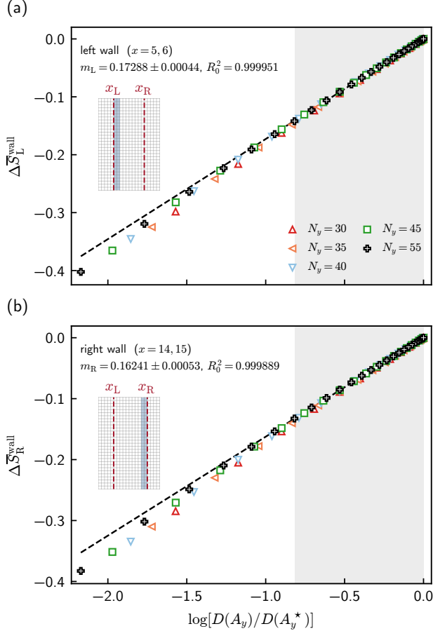
FIG. 9. Entropy carried by each wall. Entanglement contour integrated over (a) x = 5, 6 and (b) x = 14, 15 , for N_y = 30, 35, 40, 45, 55 . Each case uses S = 100 independent random-pure trajectories after 2N_y cycles. Contours are averaged over all translated strips within each trajectory before trajectory averaging, and anchored at A_y = \lfloor N_y/2 \rfloor . Dashed lines are joint fits over 8 \leq A_y \leq \lfloor N_y/2 \rfloor (shaded), with equal total weight per size and trajectory-based uncertainties including correlations between widths. Insets mark the integrated columns. The point A_y = 1 is omitted from display only.
