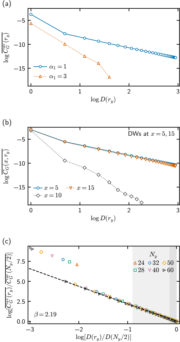
FIG. 5. Algebraic correlations on the walls. (a) Full- x average \overline{C}_G^{\text{av}}(r_y) at N_y = 60 , comparing \alpha_1 = 1, 3 . (b) Column-resolved correlations at \alpha_1 = 1 , for x = 5, 10, 15 . (c) Antipodally normalized correlations for N_y = 24, 28, 32, 40, 50, 60 . The dashed line is a joint power-law fit over 8 \leq r_y \leq N_y/2 , with equal total weight per size and \beta = 2.1903 . Gray shading marks the fit-window range. The data use S = 100 independent random-pure half-filled trajectories per case, observed after 2N_y cycles; spatial averaging precedes trajectory averaging, and the logarithm is taken last. Values below 10^{-8} are omitted from (a,b).
