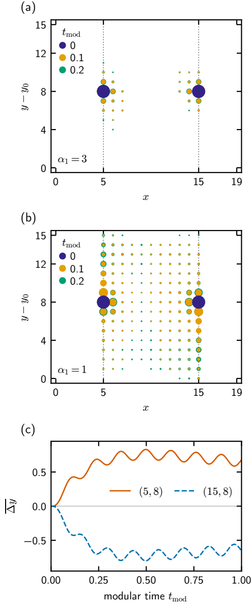
FIG. 10. Modular evolution on the walls. Two incoherent orbital profiles are initialized at each source cell (x, \delta y) = (5, 8) or (15, 8) in a half-cylinder of 16 rows. The states come from S = 100 independent random-pure trajectories per \alpha_1 = 1, 3 on a 20 \times 32 lattice after 64 cycles. (a,b) Mean densities at t_{\text{mod}} = 0, 0.1, 0.2 (purple, orange, green) for (a) \alpha_1 = 3 and (b) \alpha_1 = 1 . (c) Mean displacement for \alpha_1 = 1 within five-column source-wall windows; solid and dashed lines denote sources at x = 5 and 15 . Each observable is evaluated per cut, then averaged over 32 origins and trajectories. Bands are one trajectory SEM. Centered occupations are clipped at \pm(1 - 10^{-10}) when constructing h_A .
