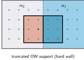
FIG. 2. Hard domain wall. The parameter \alpha takes the value \alpha_2 in the exterior (left) and \alpha_1 in the slab (right). OW modes centered on either side of the interface (dashed line) are truncated at the interface and renormalized, so their supports (shaded) do not cross it.
