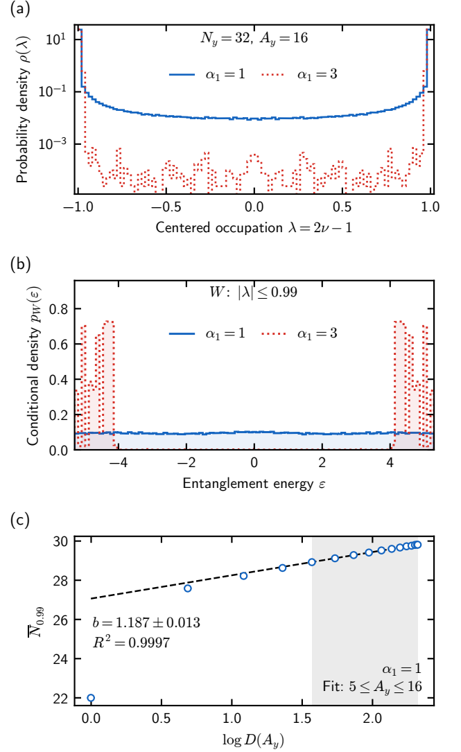
FIG. 7. Restricted spectra and mode count. Hard-wall states at N_x = 20 , N_y = 32 , cycle 64, from S = 100 independent random-pure half-filled trajectories per \alpha_1 = 1, 3 . (a) Full centered-occupation histogram, normalized to unit area. (b) Conditional unit-area energy density for |\lambda| \leq 0.99 , in 101 equal bins on [-\log 199, \log 199] . The central depletion at \alpha_1 = 3 contrasts with the finite near-zero density at \alpha_1 = 1 . Both histograms pool all 32 translated half-strips per trajectory. The retained totals are 95,398 and 83,326 for \alpha_1 = 1, 3 . (c) Raw mean window count for \alpha_1 = 1 , averaging origins within each trajectory. Bars are one trajectory SEM; the dashed fit uses 5 \leq A_y \leq 16 (shaded), while all widths are displayed. Translated cuts are correlated observations, not additional trajectories.
