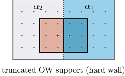
FIG. 2. Hard domain wall. The parameter \alpha takes the value \alpha_2 in the exterior (left) and \alpha_1 in the slab (right). OW modes centered on either side of the interface (dashed line) are truncated at the interface and renormalized, so their supports (shaded) do not cross it.
