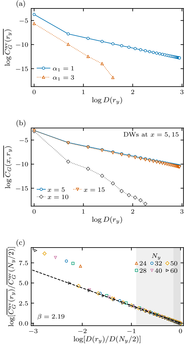
FIG. 5. Algebraic correlations on the walls. (a) Full- x average \overline{C}_G^{\text{av}}(r_y) at N_y = 60 , comparing \alpha_1 = 1, 3 . (b) Column-resolved correlations at \alpha_1 = 1 , for x = 5, 10, 15 . (c) Antipodally normalized correlations for N_y = 24, 28, 32, 40, 50, 60 . The dashed line is a joint power-law fit over 8 \leq r_y \leq N_y/2 , with equal total weight per size and \beta \approx 2.19 . [Claude: General note on captions: many carry estimator details (“transformed through the absolute value”, “translated cuts are correlated observations”, “the gap is dimensionless”). Keep panel descriptions and parameters, and move statistics conventions to one sentence at the start of Sec. III, which you already have.] Gray shading marks the fit-window range. The data use S = 100 independent random-pure half-filled trajectories per case, observed after 2N_y cycles; spatial averaging precedes trajectory averaging, and the logarithm is taken last. Values below 10^{-8} are omitted from (a,b).
