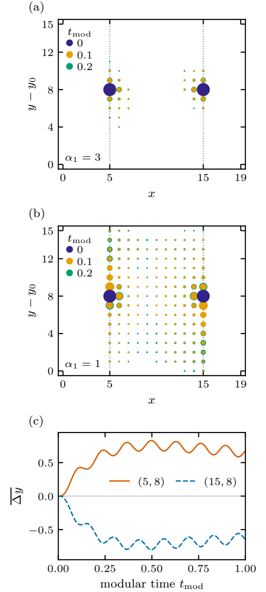
FIG. 10. Modular evolution on the walls. Two incoherent orbital profiles are initialized at each source cell (x, \delta y) = (5, 8) or (15, 8) in a half-cylinder of 16 rows. The states come from S = 100 independent random-pure trajectories per \alpha_1 = 1, 3 on a 20 \times 32 lattice after 64 cycles. (a,b) Mean densities at t_{\text{mod}} = 0, 0.1, 0.2 (purple, orange, green) for (a) \alpha_1 = 3 and (b) \alpha_1 = 1 . (c) Mean displacement for \alpha_1 = 1 within five-column source-wall windows; solid and dashed lines denote sources at x = 5 and 15 . Each observable is evaluated per cut, then averaged over 32 origins and trajectories. Bands are one trajectory SEM. Centered occupations are clipped at \pm(1 - 10^{-10}) when constructing h_A .
