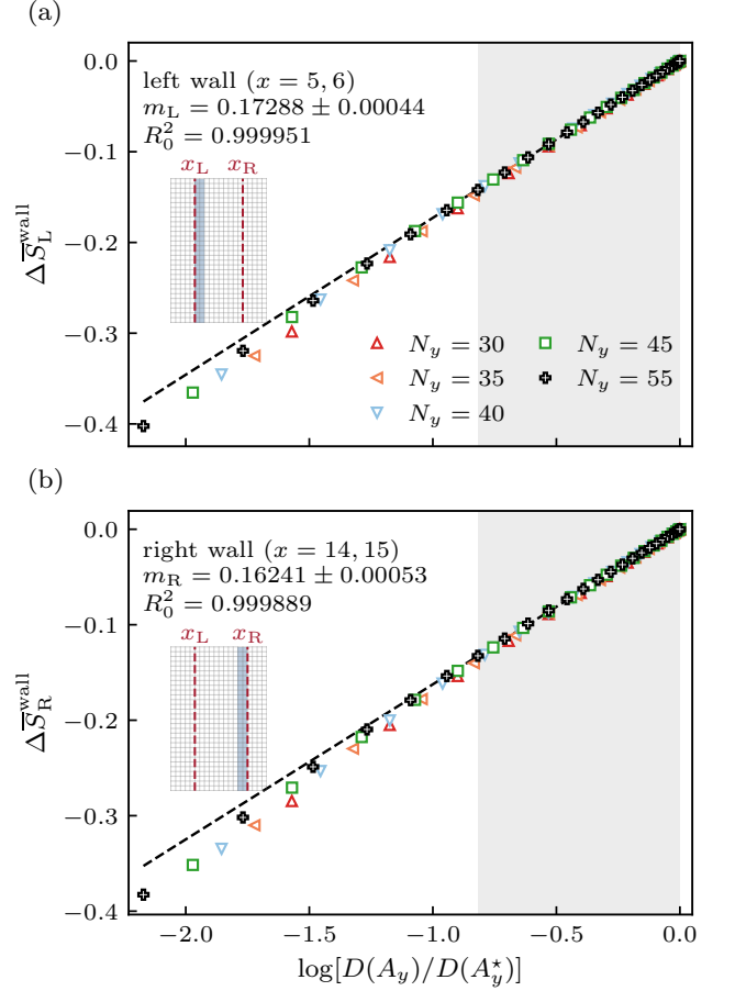
FIG. 9. Entropy carried by each wall. Entanglement contour integrated over (a) x = 5, 6 and (b) x = 14, 15 , for N_y = 30, 35, 40, 45, 55 . Each case uses S = 100 independent random-pure trajectories after 2N_y cycles. Contours are averaged over all translated strips within each trajectory before trajectory averaging, and anchored at A_y = \lfloor N_y/2 \rfloor . Dashed lines are joint fits over 8 \leq A_y \leq \lfloor N_y/2 \rfloor (shaded), with equal total weight per size and trajectory-based uncertainties including correlations between widths. Insets mark the integrated columns. The point A_y = 1 is omitted from display only.
