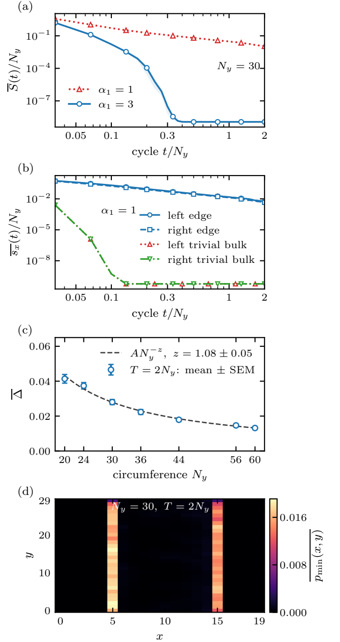
FIG. 4. Slow purification at the domain walls. (a) Mean entropy per unit length at N_y = 30 for \alpha_1 = 1, 3 . (b) Column entropy at \alpha_1 = 1 on the walls, x = 5, 15 , and in the trivial exterior, x = 2, 18 . (c) Mean finite-time gap at T = 2N_y for N_y = 20, 24, 30, 36, 44, 56, 60 ; the dashed line is an SEM-weighted fit over all seven sizes, with z = 1.08 \pm 0.05 . (d) Mean density of the unique slowest mode at N_y = 30 , T = 60 . Panels (a,b,d) start with the full system maximally mixed; the separate ensemble in (c) starts with a maximally mixed slab and a pure exterior. Each case uses S = 100 independent trajectories. Error bars and bands are one trajectory SEM; the trivial entropy plateau is a numerical floor.
