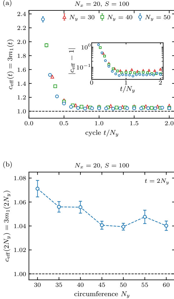
FIG. 8. Convergence of the entropy coefficient. c_{\text{eff}} = 3m_1 is extracted from a free-intercept fit of \bar{S} versus \log chord length over 8 \leq A_y \leq N_y/2 . (a) Cycle dependence for N_y = 30, 40, 50 ; the inset resolves |c_{\text{eff}} - 1| . Bars are regression standard errors of the mean-curve slope. (b) Endpoint values after 2N_y cycles for N_y = 30, 35, \dots, 60 ; bars are trajectory SEMs propagated with the covariance between widths. Both panels use S = 100 independent random-pure trajectories per size and origin averaging, but come from separate ensembles. The horizontal reference is one; connecting lines in (b) are guides.
