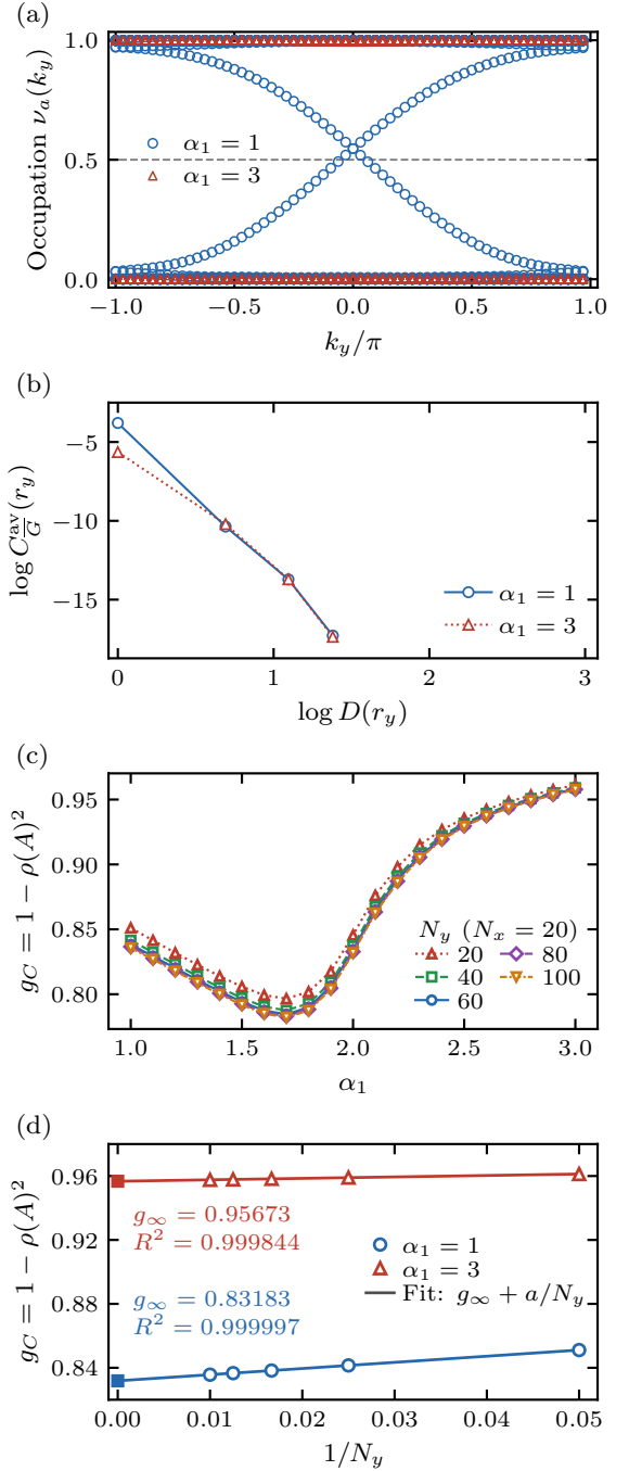
FIG. 11. Trajectory-averaged dynamics and channel gap. (a) Occupations of the translation-averaged two-point matrix and (b) its squared correlation at N_y = 64 , after 128 cycles from maximal mixing, for \alpha_1 = 1, 3 . Correlations below 10^{-8} are not displayed. (c) Exact multiplier gap g_C = 1 - \rho(A)^2 versus \alpha_1 at fixed N_x = 20 and N_y = 20, 40, 60, 80, 100 . (d) Fits g_\infty + a/N_y at \alpha_1 = 1, 3 , using all five sizes; squares at 1/N_y = 0 mark extrapolated intercepts. Outcomes are averaged analytically in the fixed repeated raster schedule, so there is no sampled-trajectory count or SEM. The gap is dimensionless.
