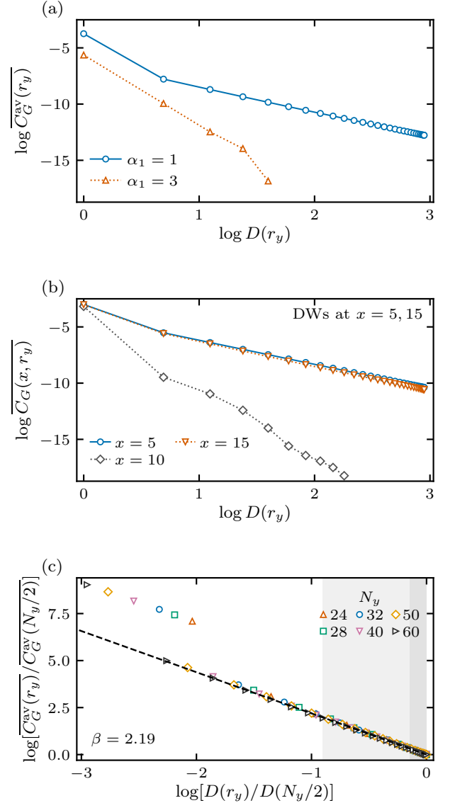
FIG. 5. Algebraic correlations on the walls. (a) Full-x average \overline{C}_G^{\text{av}}(r_y) at N_y = 60 , comparing \alpha_1 = 1, 3 . (b) Column-resolved correlations at \alpha_1 = 1 , for x = 5, 10, 15 . (c) Antipodally normalized correlations for N_y = 24, 28, 32, 40, 50, 60 . The dashed line is a joint power-law fit over 8 \leq r_y \leq N_y/2 , with equal total weight per size and \beta \approx 2.19 . [Claude: General note on captions: many carry estimator details (“transformed through the absolute value”, “translated cuts are correlated observations”, “the gap is dimensionless”). Keep panel descriptions and parameters, and move statistics conventions to one sentence at the start of Sec. III, which you already have.] Gray shading marks the fit-window range. The data use S = 100 independent random-pure half-filled trajectories per case, observed after 2N_y cycles; spatial averaging precedes trajectory averaging, and the logarithm is taken last. Values below 10^{-8} are omitted from (a,b).
