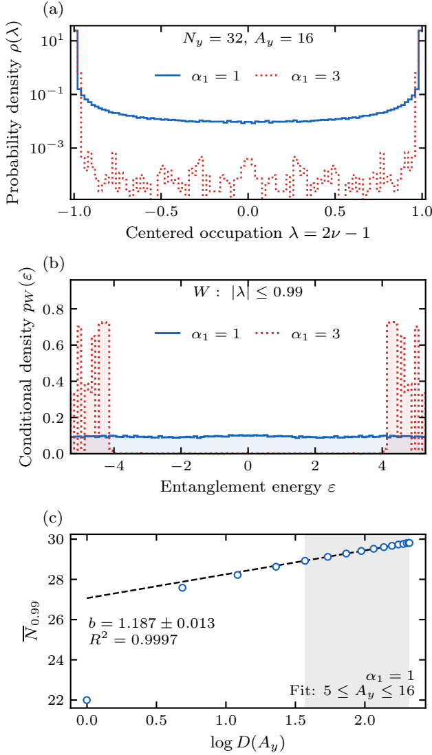
FIG. 7. Restricted spectra and mode count. Hard-wall states at N_x = 20 , N_y = 32 , cycle 64, from S = 100 independent random-pure half-filled trajectories per \alpha_1 = 1, 3 . (a) Full centered-occupation histogram, normalized to unit area. (b) Conditional unit-area energy density for |\lambda| \leq 0.99 , in 101 equal bins on [-\log 199, \log 199] . The central depletion at \alpha_1 = 3 contrasts with the finite near-zero density at \alpha_1 = 1 . Both histograms pool all 32 translated half-strips per trajectory. The retained totals are 95,398 and 83,326 for \alpha_1 = 1, 3 . (c) Raw mean window count for \alpha_1 = 1 , averaging origins within each trajectory. Bars are one trajectory SEM; the dashed fit uses 5 \leq A_y \leq 16 (shaded), while all widths are displayed. Translated cuts are correlated observations; not additional trajectories.
