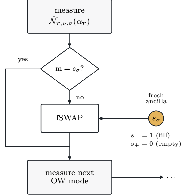
FIG. 2. Adaptive measurement and feedback. The occupation of an OW mode is measured with Born-random outcome m . If m = s_\sigma , the circuit proceeds directly to the next mode. Otherwise, an fSWAP with a fresh ancilla restores the target occupation, s_- = 1 for lower-band modes and s_+ = 0 for upper-band modes. The branches rejoin before the next measurement. The outgoing arrow and ellipsis indicate repetition over subsequent OW modes.
