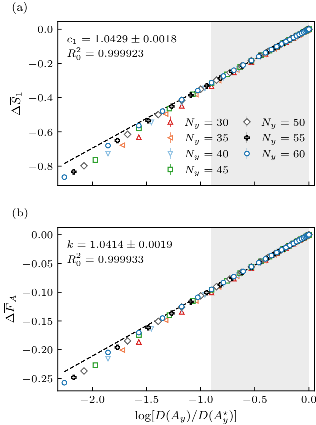
FIG. 6. Entanglement and charge fluctuations. (a) Mean strip entropy and (b) charge variance for N_y = 30, 35, \dots, 60 , shifted by their values at A_y = \lfloor N_y/2 \rfloor . Each case uses S = 100 independent random-pure half-filled trajectories after 2N_y cycles, with all strip origins averaged within each trajectory. Dashed lines are joint fits to Eq. (19) over 8 \leq A_y \leq \lfloor N_y/2 \rfloor (shaded). The point A_y = 1 is excluded from display only. The fits and their trajectory-based uncertainties retain correlations between strip widths.
