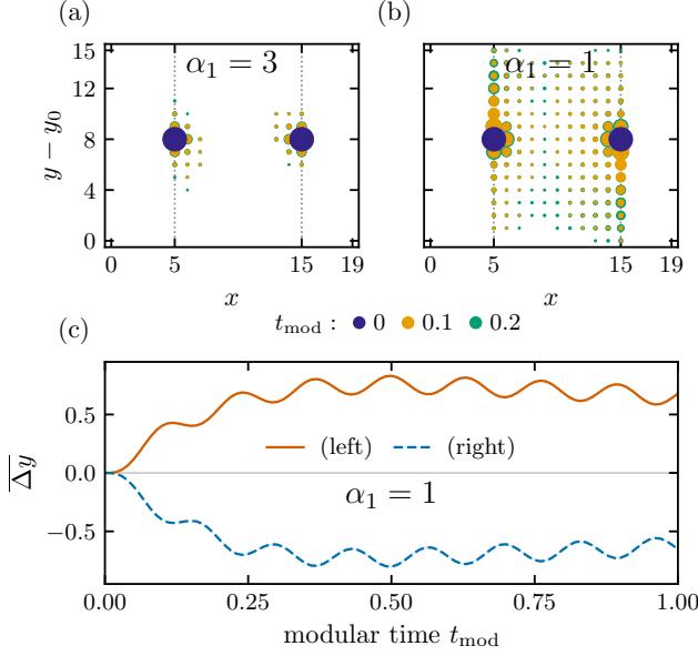
FIG. 9. Modular evolution on the walls. Two incoherent orbital profiles are initialized at each source cell (x, \delta y) = (5, A_y/2) or (15, A_y/2) in a half-cylinder of A_y = 16 rows. The states come from S = 100 independent random-pure trajectories per \alpha_1 = 1, 3 on a 20 \times 32 lattice after 64 cycles. (a,b) Mean densities at t_{\text{mod}} = 0, 0.1, 0.2 (purple, orange, green) for (a) \alpha_1 = 3 and (b) \alpha_1 = 1 . (c) Mean center-of-mass displacement \Delta y_{x_s} from the initial row \delta y = A_y/2 , defined in Eq. (33), for \alpha_1 = 1 . Solid (left) and dashed (right) lines denote x_s = 5 and 15; each five-column window is normalized by its retained weight before averaging. Each observable is evaluated per cut, then averaged over 32 origins and trajectories. Bands are one trajectory SEM. Centered occupations are clipped at \pm(1 - 10^{-10}) when constructing h_A .
