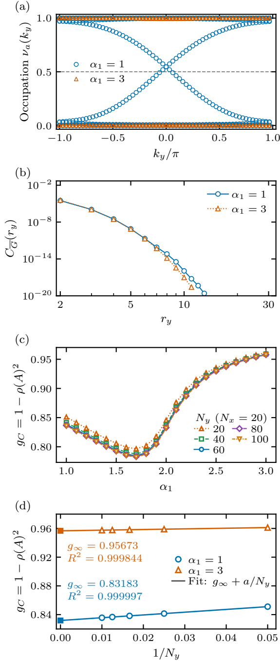
FIG. 10. Trajectory-averaged dynamics and channel gap. (a) Occupations of the translation-averaged two-point matrix and (b) its squared correlation at N_y = 64 , after 128 cycles from maximal mixing, for \alpha_1 = 1, 3 . Panel (b) uses logarithmic axes for C_{\bar{G}}(r_y) versus r_y \geq 2 ; correlations below 10^{-20} are not displayed. (c) Exact multiplier gap g_C = 1 - \rho(A)^2 versus \alpha_1 at fixed N_x = 20 and N_y = 20, 40, 60, 80, 100 . (d) Fits g_\infty + a/N_y at \alpha_1 = 1, 3 , using all five sizes; squares at 1/N_y = 0 mark extrapolated intercepts. Outcomes are averaged analytically in the fixed repeated raster schedule, so there is no sampled-trajectory count or SEM. The gap is dimensionless.
