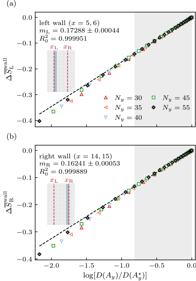
FIG. 8. Entropy carried by each wall. Entanglement contour integrated over (a) x = 5, 6 and (b) x = 14, 15 , for N_y = 30, 35, 40, 45, 55 . Each case uses S = 100 independent random-pure trajectories after 2N_y cycles. Contours are averaged over all translated strips within each trajectory before trajectory averaging, and anchored at A_y = \lfloor N_y/2 \rfloor . Dashed lines are joint fits over 8 \leq A_y \leq \lfloor N_y/2 \rfloor (shaded), with equal total weight per size and trajectory-based uncertainties including correlations between widths. Insets mark the integrated columns. The point A_y = 1 is omitted from display only.
