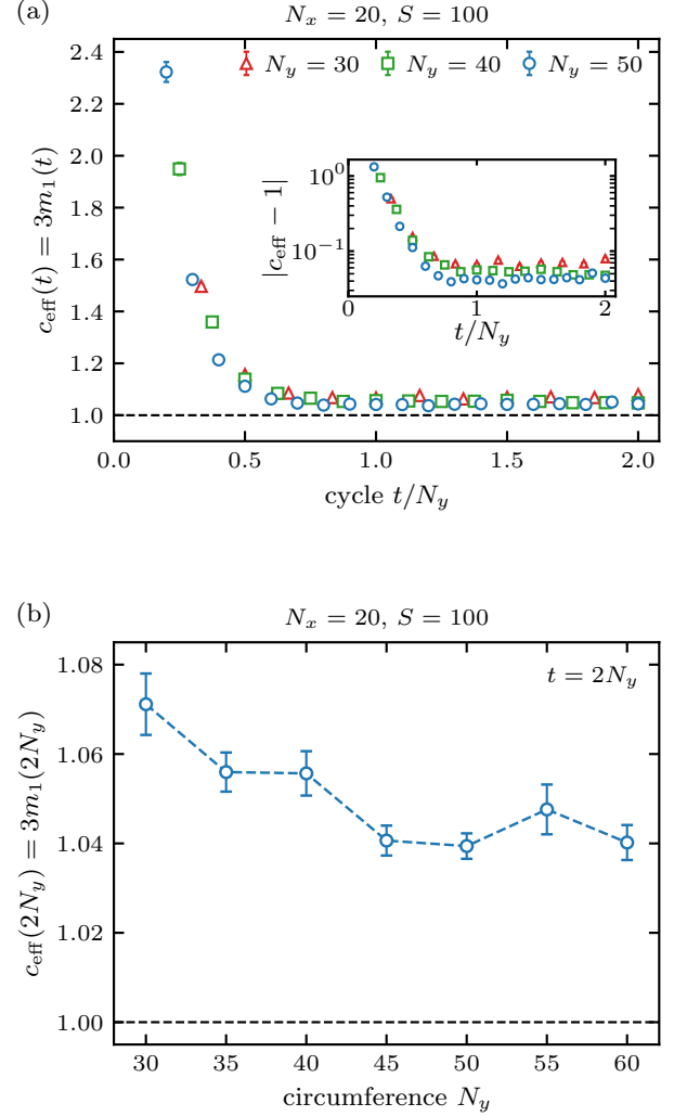
FIG. A3. Convergence of the entropy coefficient. c_{\text{eff}} = 3m_1 is extracted from a free-intercept fit of \overline{S} versus log chord length over 8 \leq A_y \leq N_y/2 . (a) Cycle dependence for N_y = 30, 40, 50 ; the inset resolves |c_{\text{eff}} - 1| . Bars are regression standard errors of the mean-curve slope. (b) Endpoint values after 2N_y cycles for N_y = 30, 35, \dots, 60 ; bars are trajectory SEMs propagated with the covariance between widths. Both panels use S = 100 independent random-pure trajectories per size and origin averaging, but come from separate ensembles. The horizontal reference is one; connecting lines in (b) are guides.
