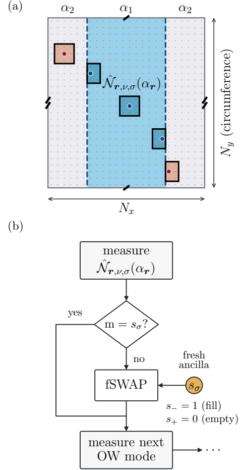
FIG. 1. Domain-wall geometry and adaptive circuit. (a) Periodic geometry with \alpha_{\mathbf{r}} = \alpha_1 in the central slab and \alpha_2 in the trivial exterior. Matching marks identify opposite boundaries. Salmon and blue windows show exterior and slab OW supports; dots mark their centers. Bulk supports contain 3 \times 3 cells; interface supports are clipped and renormalized. (b) An occupation measurement returns the Born outcome m . If m = s_{\sigma} , correction is bypassed; otherwise an fSWAP with a fresh ancilla restores s_- = 1 or s_+ = 0 . The branches rejoin and the procedure repeats for subsequent OW modes.
